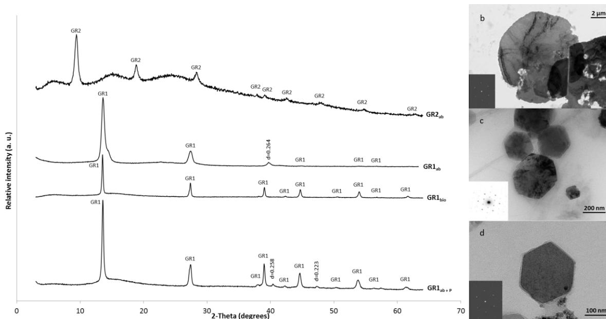
Figure 50. X-ray diffractograms (Co, \lambda = 0.178897 nm) of the biogenic carbonated green rust 1 after microbial reduction of lepidocrocite ( \gamma\text{-FeOOH} ) by Shewanella putrefaciens (GR1 bio ), chemically synthesized carbonate green rust 1 (GR1 ab ), chemically synthesized carbonate green rust 1 stabilized by phosphate (GR1 ab+P ) and sulfate green rust 2 (GR2 ab ) (a); TEM images of GR1 bio , (b), GR2 ab (c), and GR1 ab+P (d) crystals. Inserts show the electron diffraction pattern of each GR. With GR1 ab+P , a few minor peaks ( d = 0.223 nm; d = 0.258 nm) were detected on XRD diffractogram (a), corresponding probably to chukanovite ( \text{Fe}_2(\text{OH})_2\text{CO}_3 ), but this phase was not confirmed by Mössbauer analysis.
