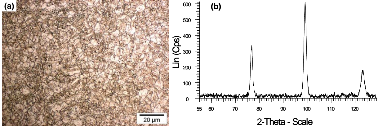
Figure 117 – Structure of medium Mn steel quenched after holding at 750°C for 30min: (a) observation with optical microscope after Dino etching and (b) corresponding X-ray spectrum.
