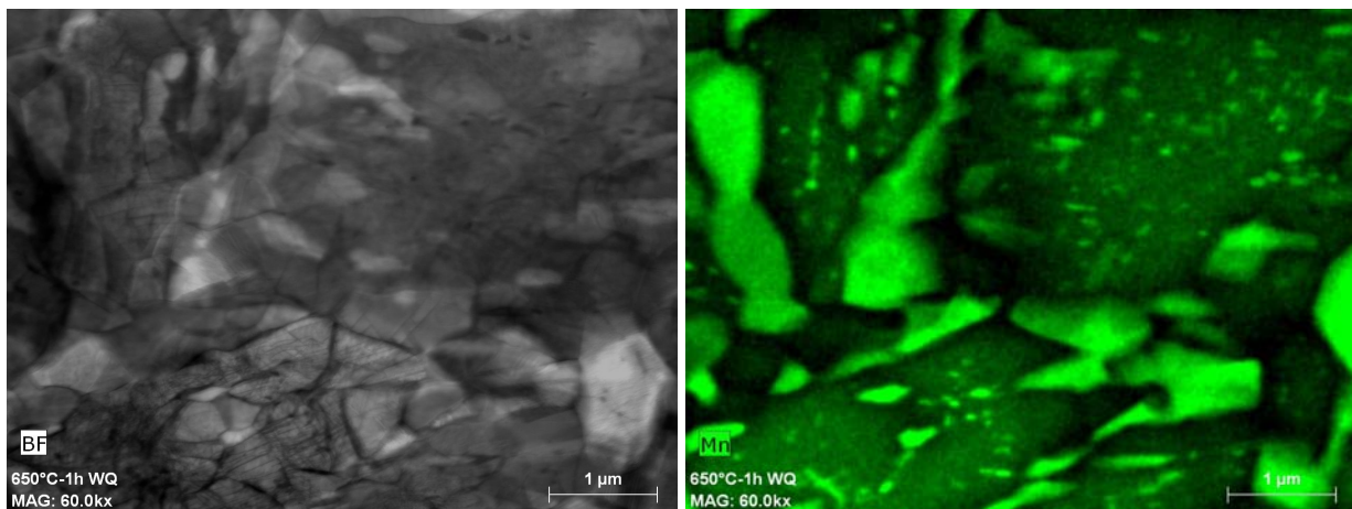
Figure 158 – Bright field TEM image (at left) and the EDX-hypermap of corresponding zone (at right) of 1h sample (3 rd hypermap).
