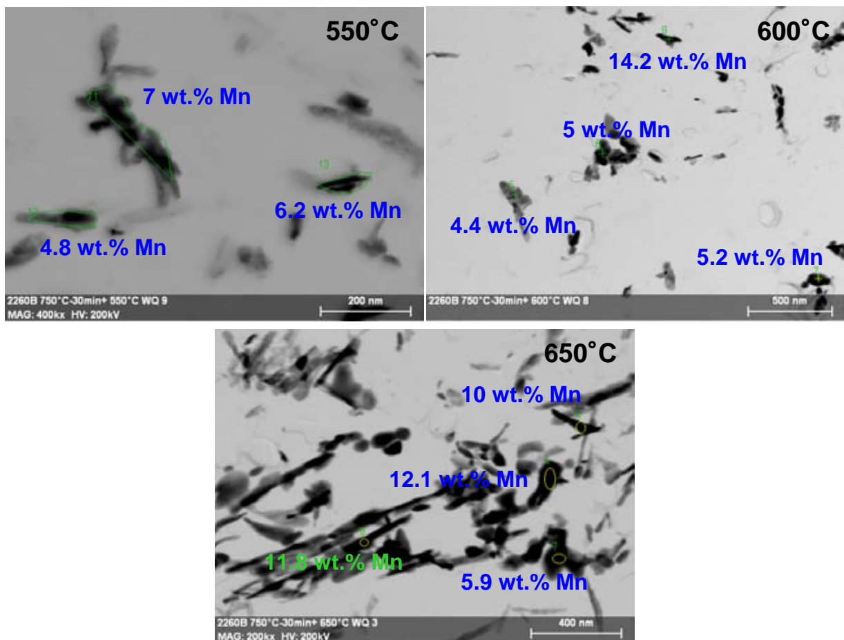
Figure 78 – TEM images on replicas of the samples obtained with different reheating temperatures: 550, 600 and 650°C. Mn content of carbides measured with EDX is shown directly on the images.
