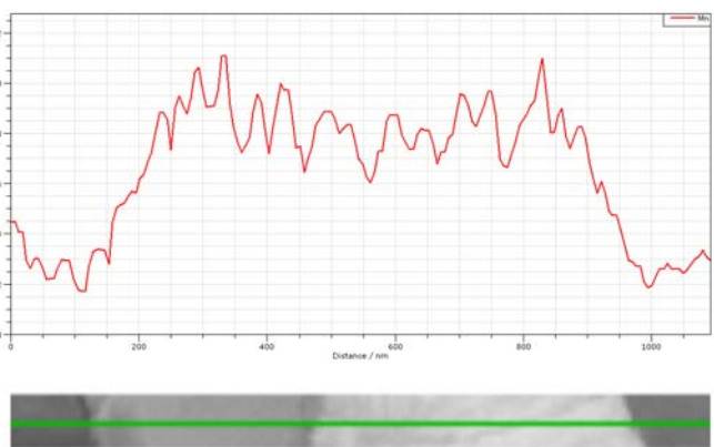
Figure 163 – Mn profiles of 2h sample: at left are presented selected zones and at right – corresponding Mn evolutions as a function of distance.
