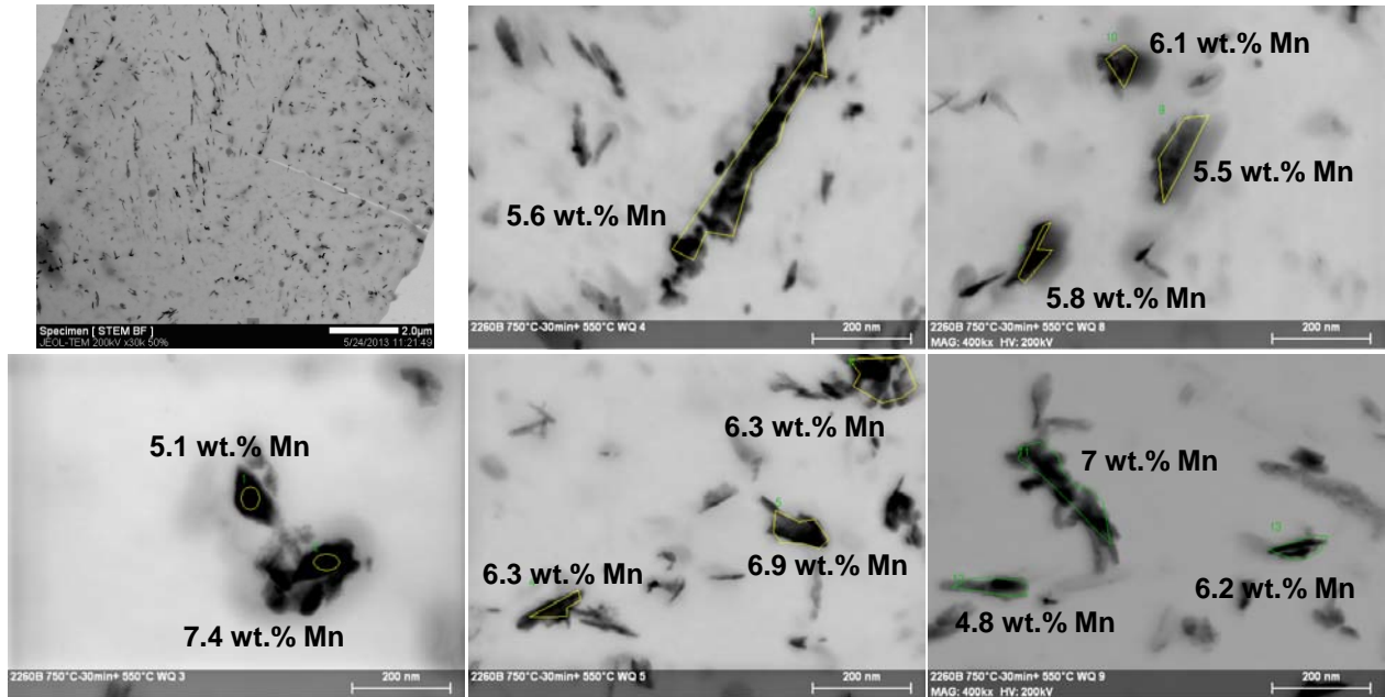
Figure 146 – TEM images obtained using replicas of the sample heated up to 550°C: left up corner - low magnification image of the analyzed zone and the others are images of carbides with their respective Mn content, measured by EDX.
