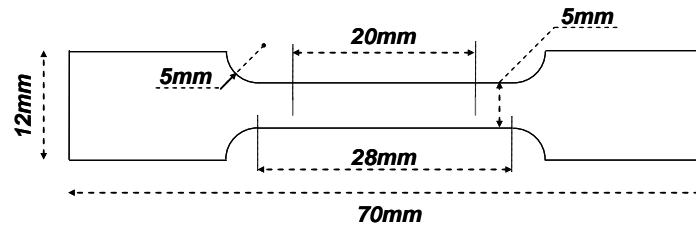
Figure 48 – Scheme of the small (so-called “mini”) specimens used for tensile tests after gradient batch annealing.
