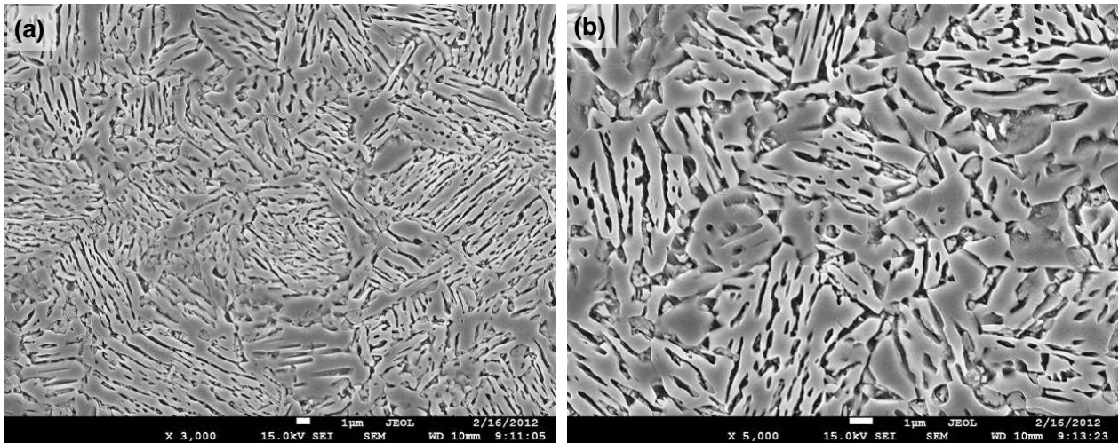
Figure 142 – SEM images of the microstructures obtained after 10h ART annealing at 650°C: (a) \times 3000 ; (b) \times 5000 .
