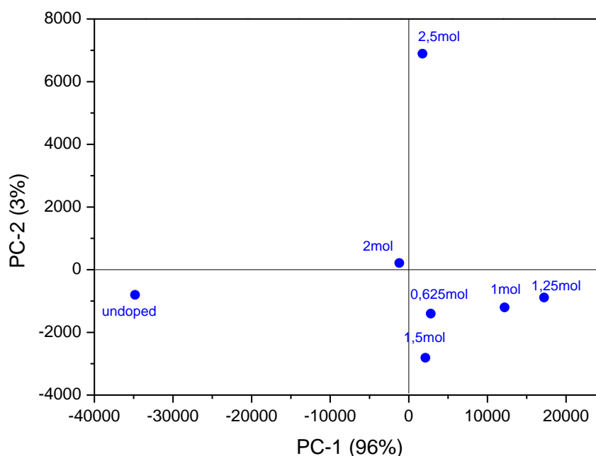
Figure III. 9- Scores of spectra (range of 100\text{cm}^{-1} - 200^{-1} ) of all samples of \text{Y}(\text{ZX})\text{Y} configuration obtained at low temperature ( -180^\circ\text{C} )
