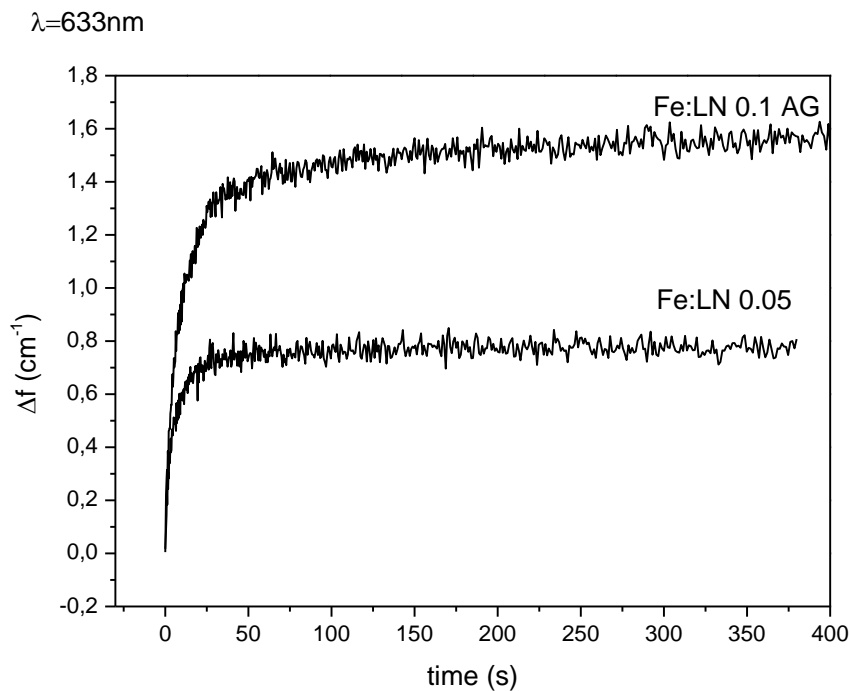
Figure IV. 26 -Time evolution for the peak frequency of the A_1(\text{TO}_4) mode in samples Fe:LN 0.05 and Fe:LN 0.1 asgrown (see table IV.2)
