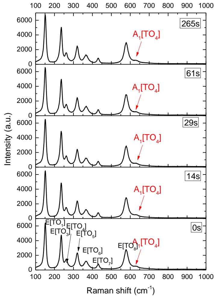
Figure IV. 7 – Backscattering Raman spectra as a function of time for the configuration X(YZ)\bar{X}
