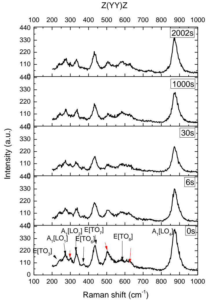
Figure IV. 17 – Forward Raman spectra as a function of time for the configuration Z(YY)Z
