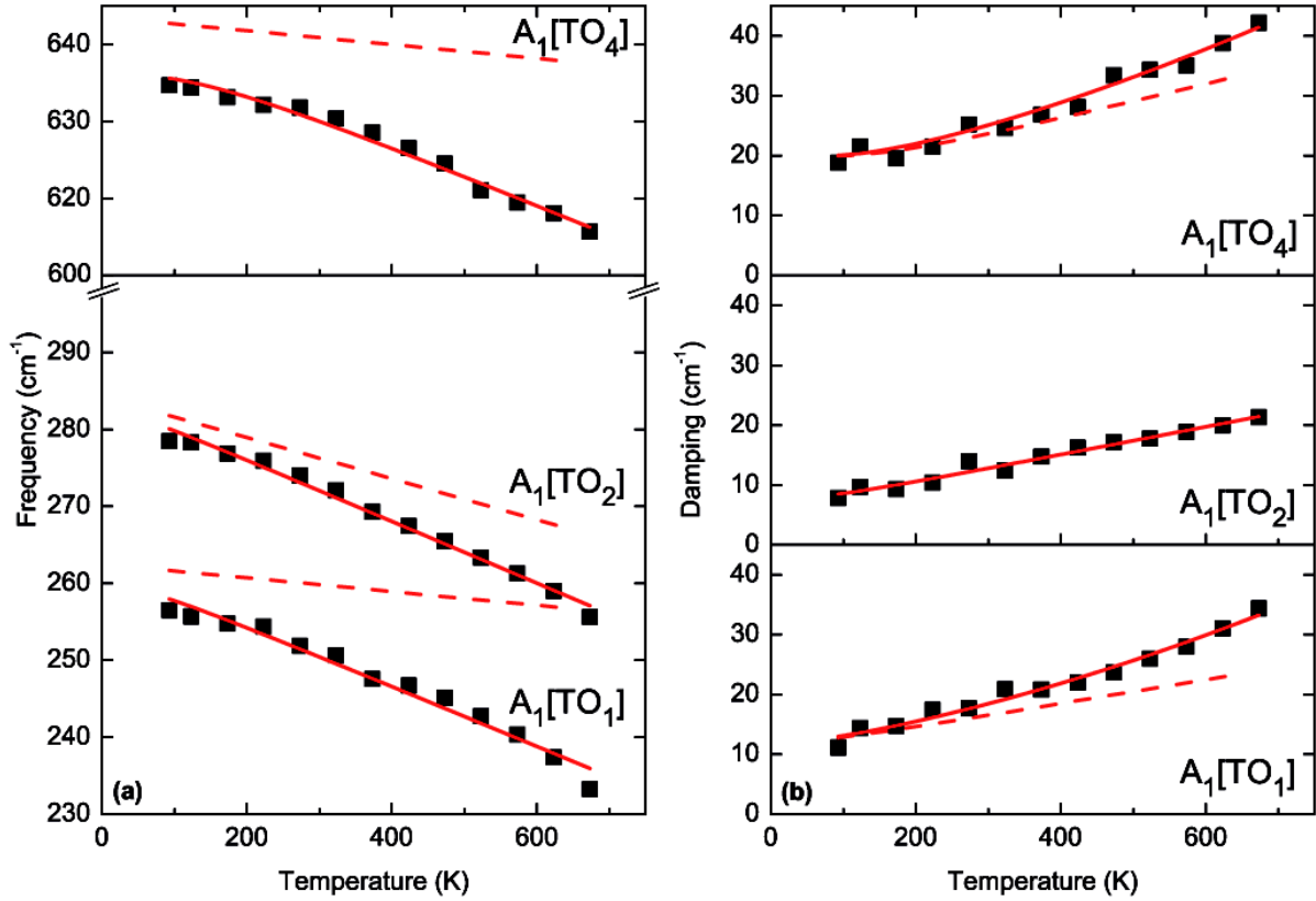
Figure A.5 – Temperature dependence of the frequency (part a) and damping (part b) of A 1 [TO] phonons in LN. Dots are experimental data and continuous lines are fits to equations 5 and 6, respectively. Dashed lines correspond to calculations when the last term in these equations is neglected
