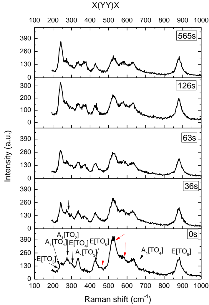
Figure IV. 9 – Forward Raman spectra as a function of time for the configuration X(YY)X . Red arrows indicate unexpected peaks as mentioned
