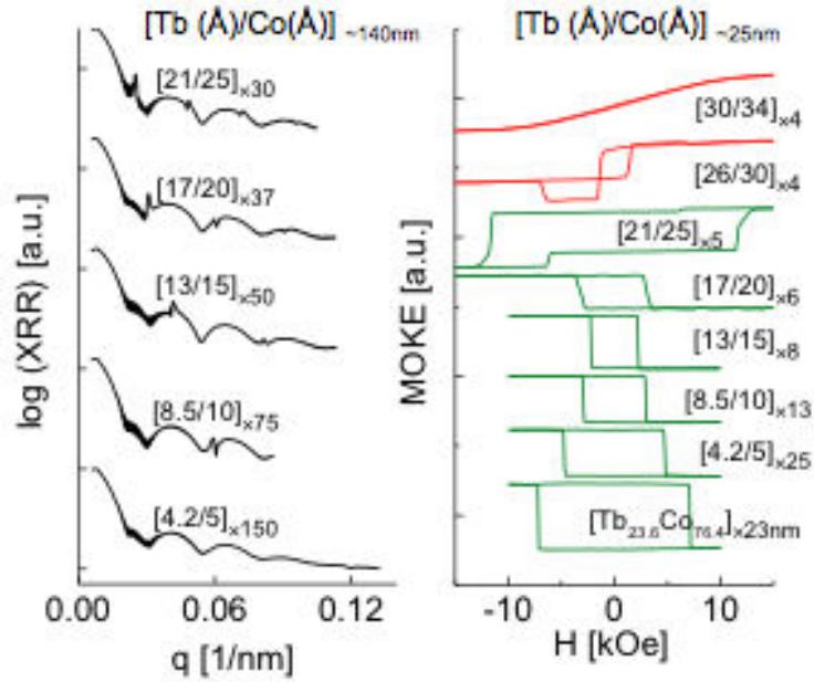
Figure 2.14: (a) X-ray reflectivity (small angle diffraction) curves for Tb/Co multilayers showing clear super-structure peaks that confirm the distinct layers and periodic nature of the multilayer samples, (b) their associated MOKE hysteresis showing the inversion of the hysteresis cycle.
