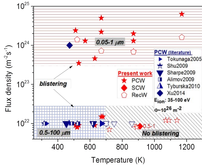
Figure 4.20: Lateral blister size is given as a function of exposure temperature and incident flux density. Empty symbols indicate the lack of blistering. The red stars ( \star ), pentagons ( \square ) and filled diamonds ( \blacklozenge ) represent the present work results on blistering of the “as received” (LGW and SGW), RECW and SCW samples, respectively. The literature data (blue symbols) correspond to polycrystalline tungsten material [4, 10, 11, 22–24]
