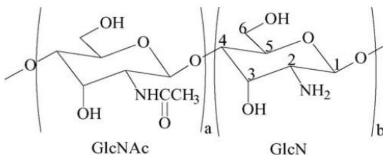
Figure 9. Chemical structure of (a) 2-acetoamido-2-deoxy-glucofuranose (GlcNAc) and (b) 2-amino-2deoxy-D-glucofuranose (GlcN) joined by \beta(1,4) glycosidic bonds (Guinesi and Cavalheiro, 2006)
