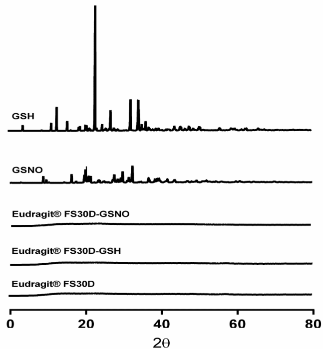
Figure 2. Powder X-ray diffraction (PXRD) pattern of GSH, GSNO and their microparticles
