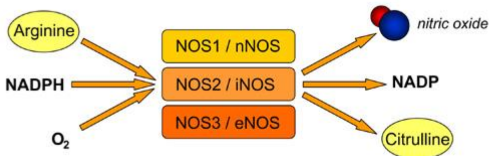
Figure 1. In vivo formation of NO (University of reading)
