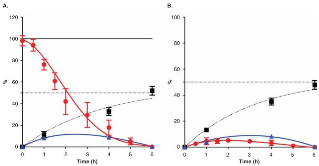
Figure 9. Concentrations of GSNO (●), NO 2 /NO (▲) and NO 3 (■) as the percentage of the initial concentration of the donor chamber (100 μM). A) Donor chamber; B) acceptor chamber (n = 3, mean value ± s.d.). GSNO: S-nitrosoglutathione.
