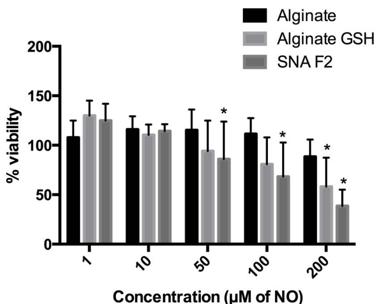
Fig. 8: Cell viability of Caco2 cell line after exposure to different concentrations of alginate, alginate-GSH conjugate and SNA F2 (n=3, mean \pm S.D.). For SNA F2, the concentrations are expressed in \mu\text{M} of NO; for the other polymers, corresponding concentration are used. * Kruskal Wallis test (comparison with alginate) : p < 0.05
