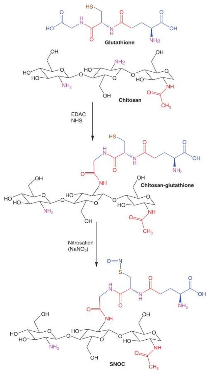
Figure 1. Reaction scheme for the synthesis of SNOC. First step: synthesis of a chitosan-glutathione conjugate. Second step: nitrosation of chitosan-glutathione conjugate. SNOC: S-nitrosoglutathione-oligosaccharide chitosan.
