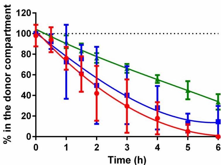
Figure 20. Concentrations of GSNO (- ● -), SNOC G2 (- ■ -) and SNA F2 (- ▲ -) as a function of percentage of the initial concentration of the donor compartment (100 μM). Donor compartment; (n=3, mean value ± S.D)
