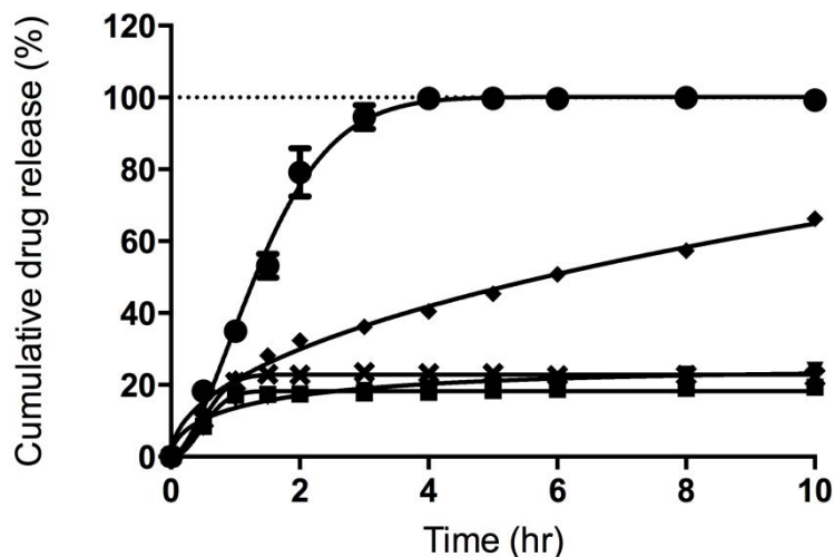
Figure 4. Drug release of GSH (GSH + GSSG) from microparticles at different pH values, - X - pH 1.2, - ■ - pH 3, - ▼ - pH 6, - ◆ - pH 6.8, - ● - pH 7.4, (n = 3, mean value \pm S.D).
