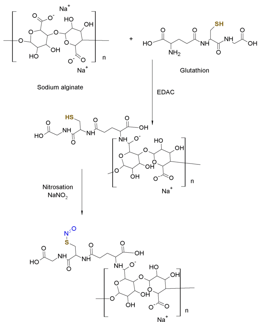
Fig. 1: Reaction scheme for the synthesis of SNA. 1 st step: synthesis of an alginate-glutathione conjugate. 2 nd step: nitrosation of alginate-glutathione conjugate.
