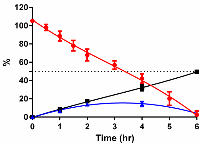
Fig. 4: Concentrations of GSNO (-●-), NO 2 /NO (-▲-) and NO 3 (-■-) as the percentage of the initial concentration of the donor chamber (100 μM). Donor chamber; (n=3, mean value ± S.D)
