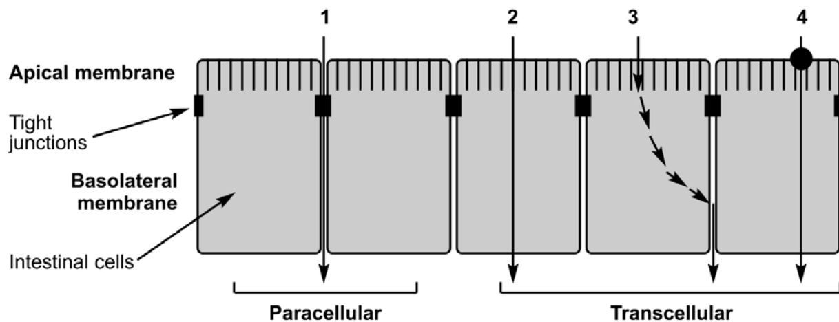
Figure 17. Routes and mechanism of transport of molecules across the intestinal epithelium (Le Ferrec et al., 2001)
