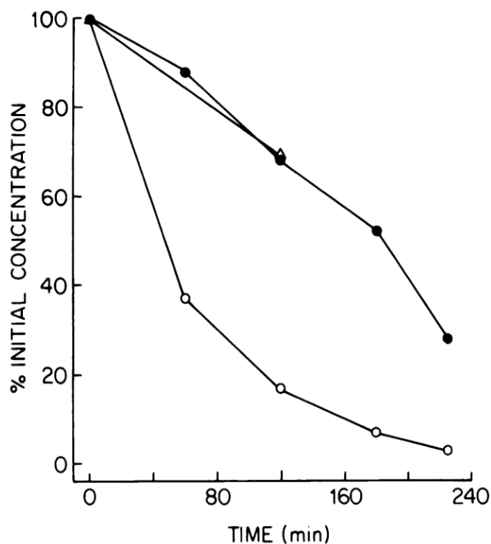
Figure 22. Stability of GSNO in human BALF. Under identical conditions (pH 7.30, 21% O 2 , 25 °C) endogenous GSNO in BALF with a patient with cystic fibrosis and pneumonia (▲) has stability identical to that of exogenous GSNO (●). The decomposition of exogenous GSNO is accelerated in the presence of 95% O 2 (○) (Gaston et al., 1993)
