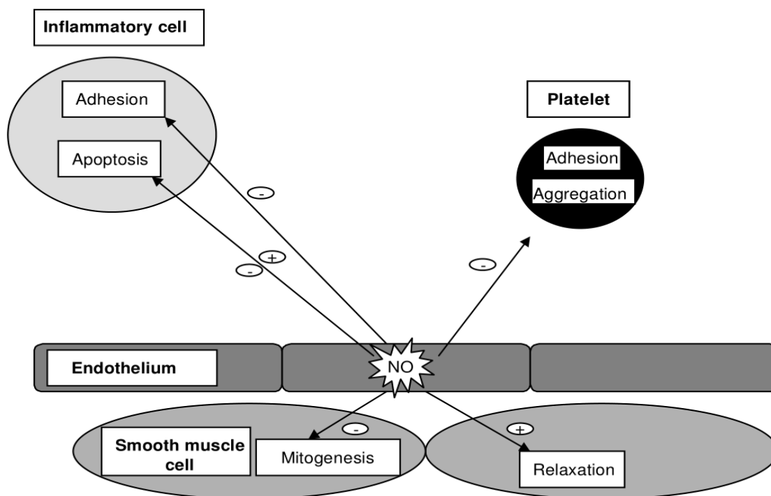
Figure 3. The major vascular functions of endothelium derived NO (Megson and Webb, 2002)
