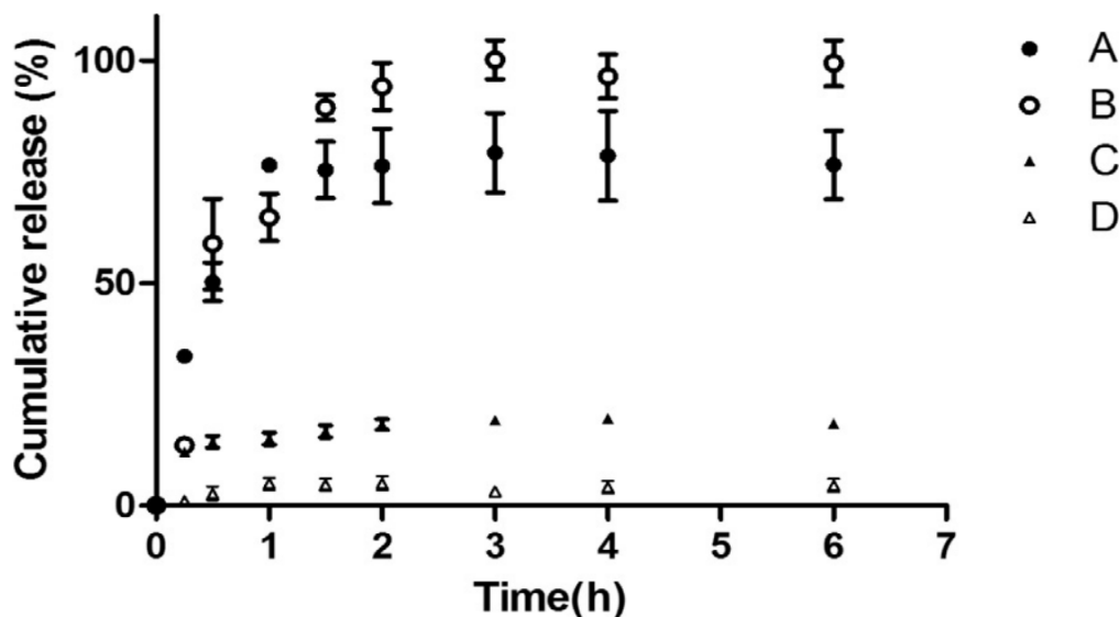
Figure 14. Release kinetics of GSNO-NP in phosphate buffer pH 7.4 at 37 °C. GSNO release from free GSNO (A) or from GSNO-NP (B); Nitrite ions released from free GSNO (C) or from GSNO-NP (D). Mean \pm SD, n = 3 (Wu et al., 2015)
