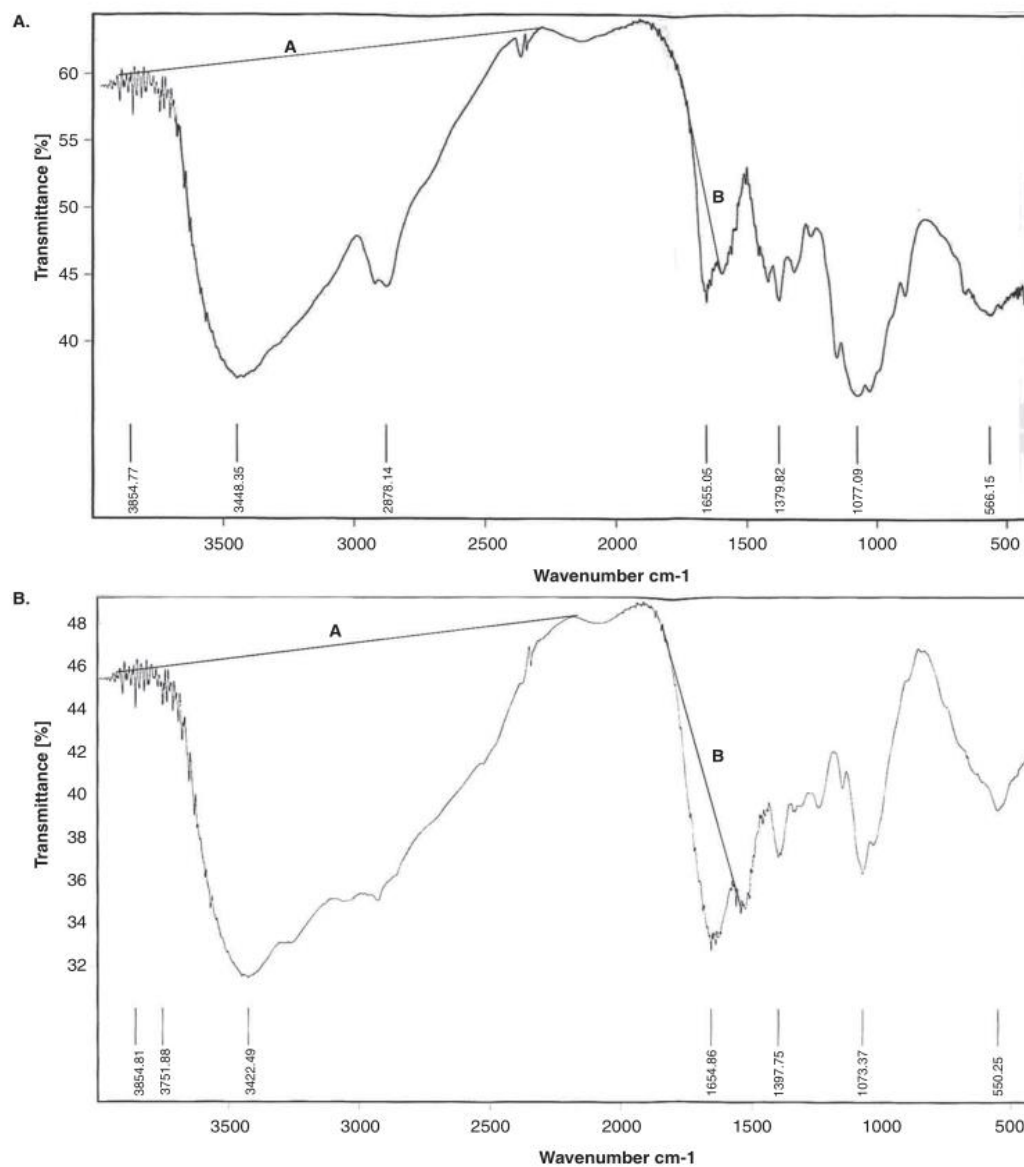
Figure 4. FTIR spectra used for % acetylation determinations. A. Chitosan; B. Chitosan GSH. GSH: Glutathione.
