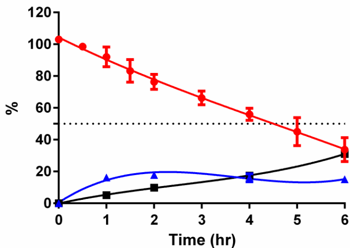
Fig. 6: Concentrations of SNA F2 (-●-), NO 2 /NO (-▲-) and NO 3 (-■-) as the percentage of the initial concentration of the donor chamber (100 μM). Donor chamber; (n=3, mean value ± S.D)
