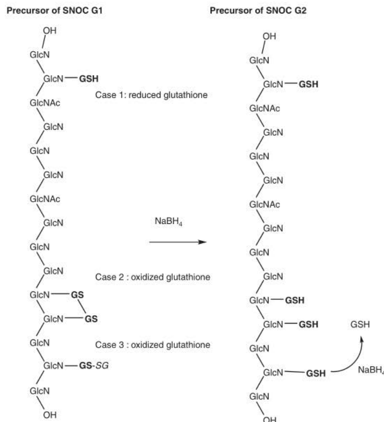
Figure 2. Various possibilities for GSH fixation to the chitosan backbone. Case 1: GSH remains in the reduced form; Case 2: two GSH molecules bound on the polymer can form a disulfide bound; this can also occur between different polymer chains; Case 3: a linked GSH can form a disulfide bound with a free molecule. Reaction after \text{NaBH}_4 treatment.
