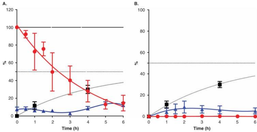
Figure 8. Concentrations of SNOC G2 (●), NO 2 /NO (▲) and NO 3 (■) as the percentage of the initial concentration of the donor chamber (100 μM). A) Donor chamber; B) acceptor chamber (n = 3, mean value ± s.d.). SNOC: S-nitrosoglutathione-oligosaccharide chitosan.
