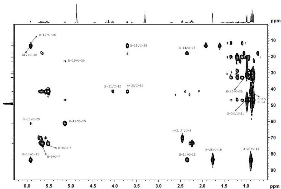
Figure 71. HMBC (1) spectrum of AFB in methanol d_4
