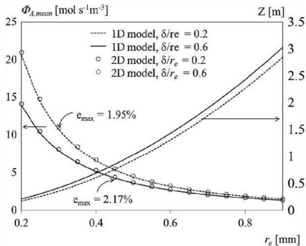
Fig. 7. Variation of the average absorbed fluxes (left axis) and of the contactor length ( Z , right axis) with the external fiber radius; no gas-membrane mass-transfer limitations; u_G^0 varied between 0.53 \text{ m s}^{-1} and 0.78 \text{ m s}^{-1} .
