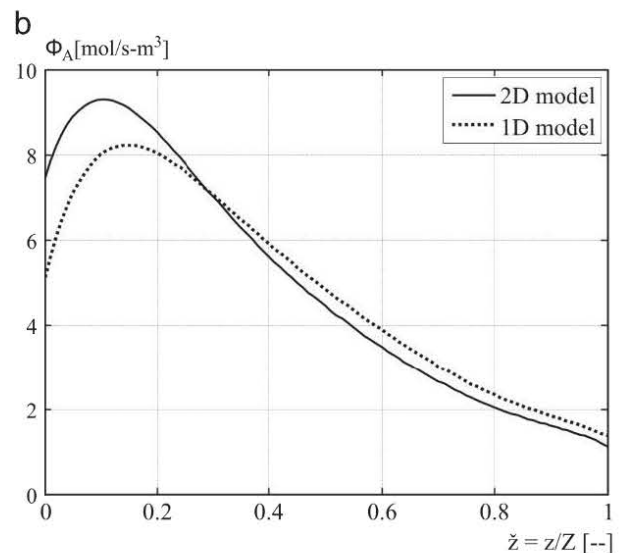
Fig. 8. Variation of the local absorbed flux with the dimensionless axial coordinate; simulations performed for r_e = 0.2 \text{ mm} and \delta/r_e = 0.6 ; (a) \epsilon/\tau = 0.2 , u_G^0 = 0.53 \text{ m s}^{-1} , Z = 0.21 \text{ m} ; (b) \epsilon/\tau = 5 \times 10^{-3} , u_G^0 = 0.32 \text{ m s}^{-1} , Z = 0.36 \text{ m} .
