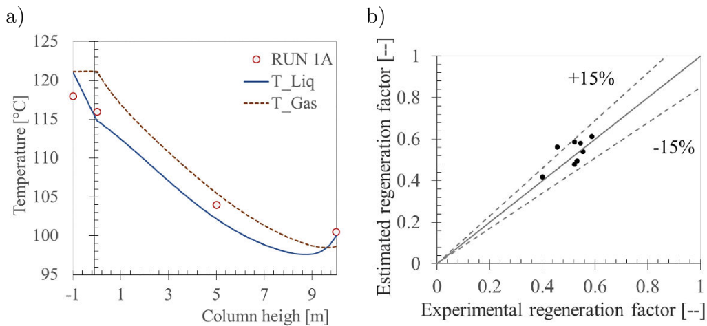
Figure 5.2 Validation of the stripping section simulation of the Esbjerg pilot plant. Solid and dotted lines: model predictions. Dots: experimental data. a) Temperature profile of the stripper for the Run 1A, b) parity plot of regeneration factor for the CASTOR campaign
