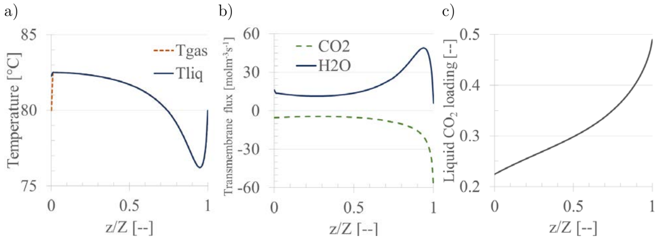
Figure 5.8 Simulation results of LTS. u_G^{\text{in}} = 2.8\text{ms}^{-1} , k_{M,\text{CO}_2^{\text{eq}}} = 10^{-3}\text{ms}^{-1} . Axial profiles of a) temperature, b) transmembrane flux and c) liquid CO 2 loading
