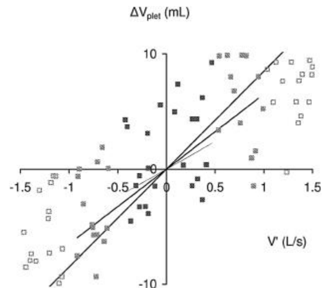
Fig. 2. Same data as in Figure 1. The slope of the \Delta V_{plet} –V’ relationship (specific airway resistance) decreases when flow range for computation is narrowed. y-axis scale has been enlarged and symbols lightened for better readability.
