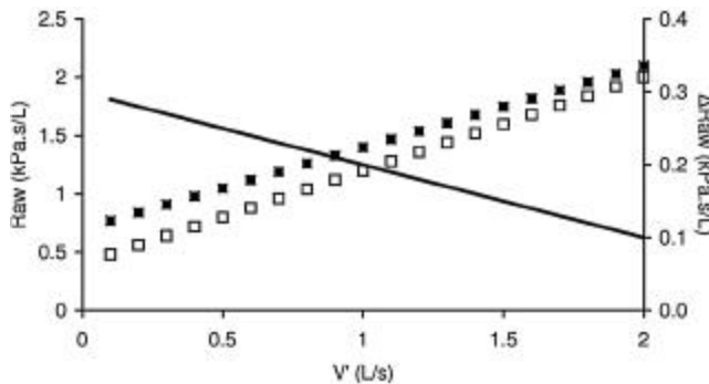
Fig. 5. Airway resistance (Raw) is computed using Roher's model-coefficients K1 and K2 to simulate the contribution of upper and lower airways when flow ( V' ) ranges from 0–2 L/sec. Raw for control and asthma are open and closed squares, respectively. The line is the Raw difference between asthma and control ( DRaw ) that decreases when the amplitude of flow is increased. Raw is given by K1 \pm K2 \cdot V' . K1 and K1/K2 are respectively 4 hPa.s/L and 0.5 L in control, and 7 hPa.s/L and 1 L in asthma.
