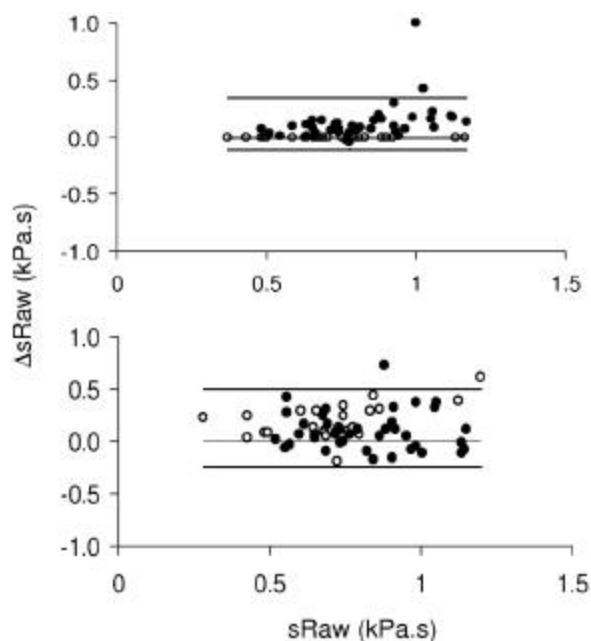
Fig. 4. Bland and Altman plots showing difference between 2 estimates of sRaw (DsRaw) against their mean. (A) sRaw computed within full scale flow and within 1 L/sec; (B) sRaw computed within full scale flow and within 0.5 L/sec. Note the generally positive difference and a trend for larger difference when sRaw increases in panel A. Open circles: control; closed circles: asthma. The 95% confidence interval is indicated.
