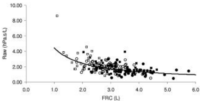
Fig. 1. Relationship between airway resistance (Raw) and functional residual capacity (FRC) in healthy young adult males (closed symbols) and females (open symbols) from Hanoi, Vietnam (squares) and Nancy, France (circles). Note distribution along a single hyperbola, in keeping with lack of gender or ethnic related difference in specific airway resistance.
