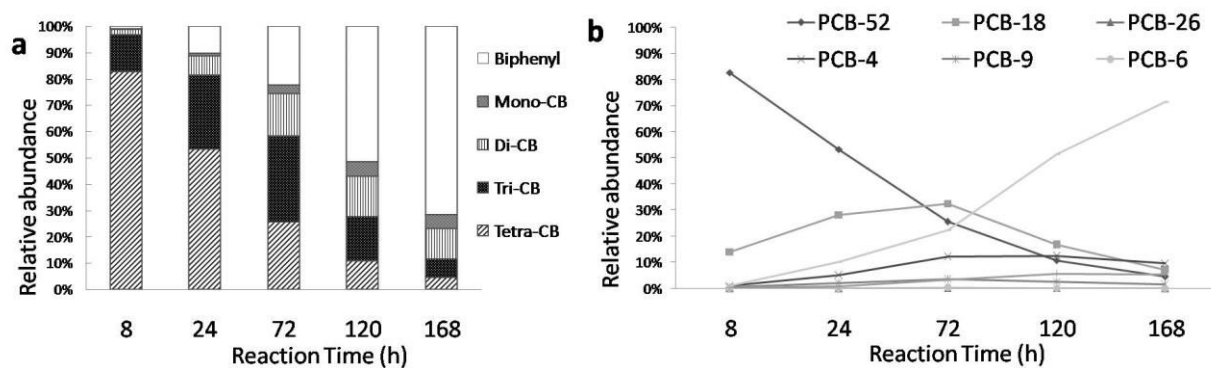
Figure 3.2 Dechlorination of PCB-52 by nZVI in the presence of nickel ions; reaction time = 168 h:
