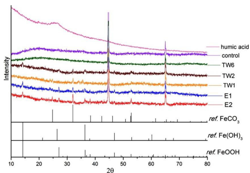
Figure 4.4 XRD spectra of ZVI after experiments with selected treatments, compared with reference spectra of humic acid and the iron minerals FeCO 3 , Fe(OH) 3 , and FeOOH.
