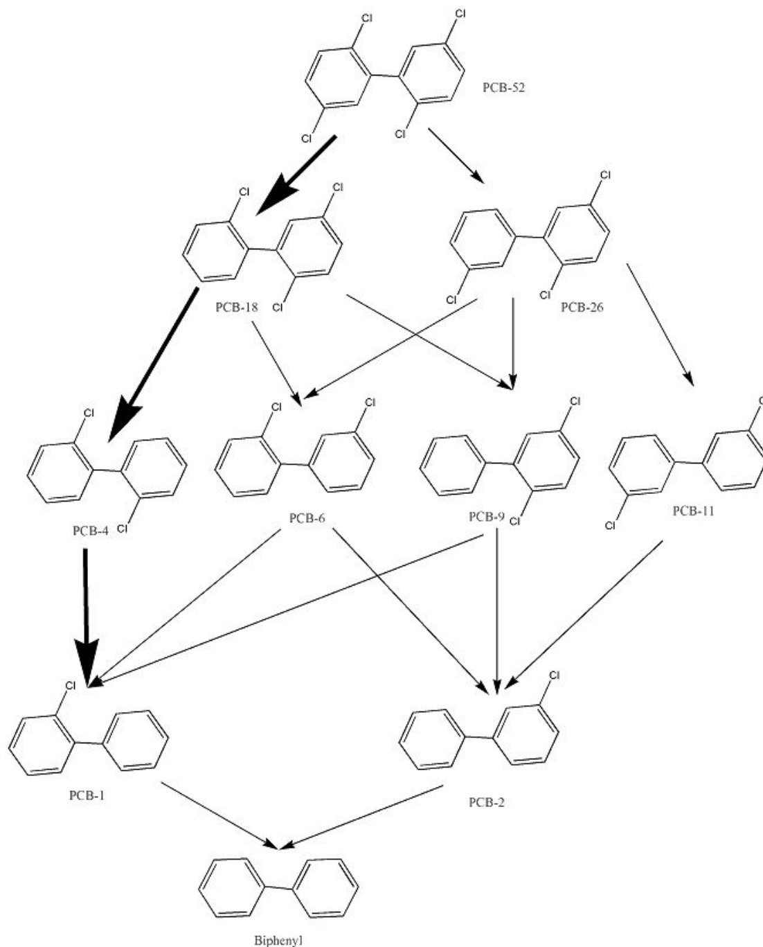
Figure 3.4 Pathways for dechlorination of PCB-52 by nZVI in the presence of \text{Ni}^{2+} ; bold arrows indicate the major pathway.
