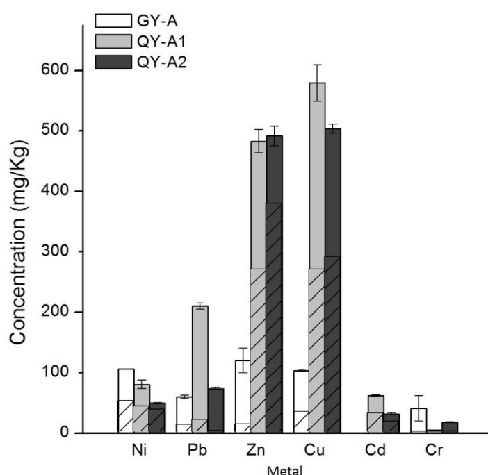
Figure 2.3 Contents of metals in samples from acid washing sites (diagonal portion as the available portion).
