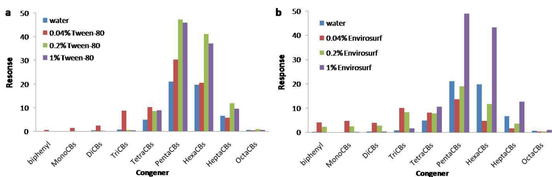
Figure 5.5 Response of mono- through octa-CBs detected by GC-MS SIM mode with different surfactants for 168 h: a, Tween-80 treatment; b, Envirosurf treatment.
