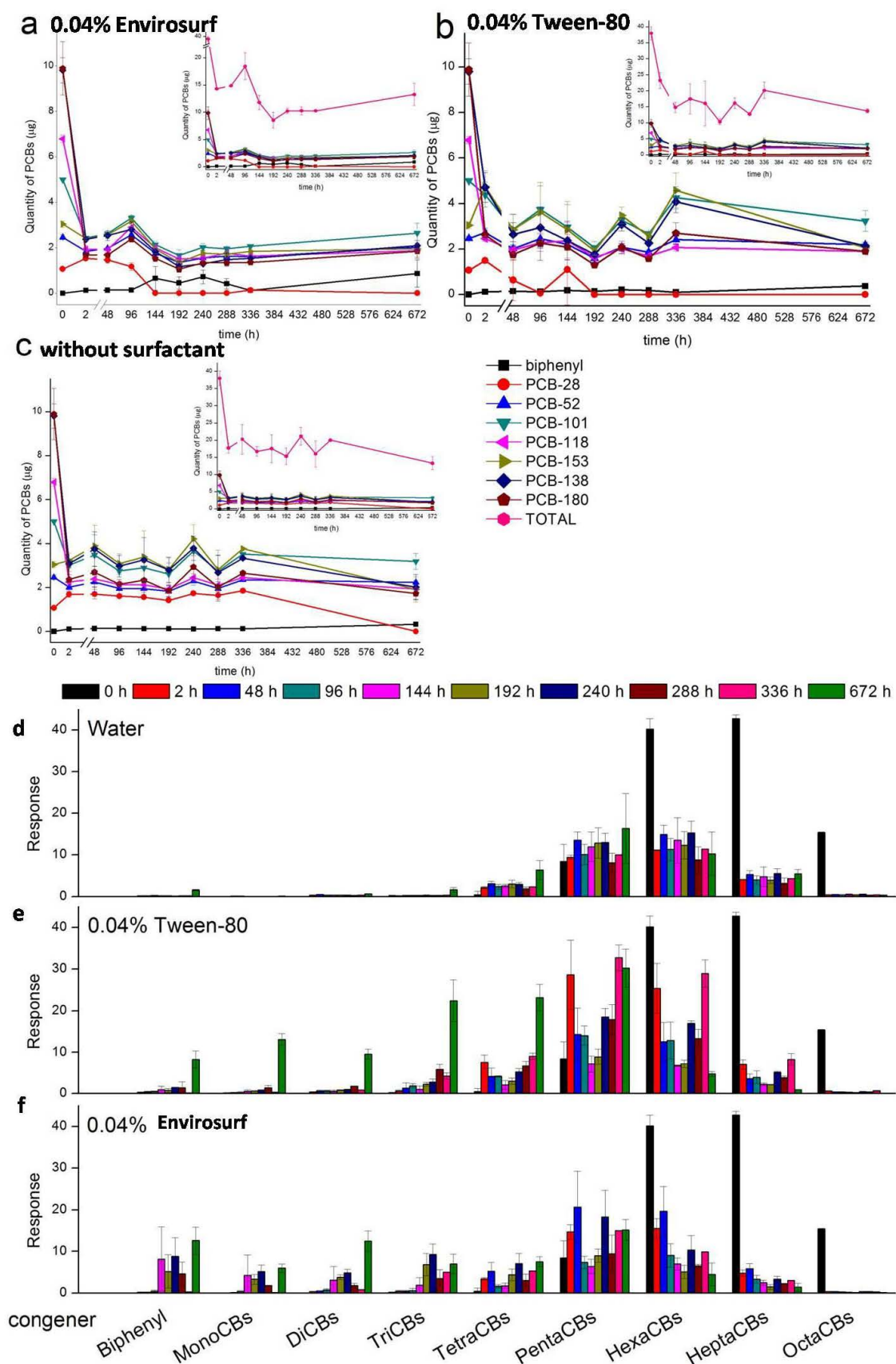
Figure 5.6 Dechlorination kinetics in 28 d (a-c: \Sigma PCBs + biphenyl, e-f: response of mono- through octa-CBs detected by GC-MS SIM mode).
