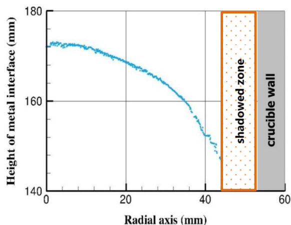
Figure 49: South cross-section of the deformed surface – Experiment 9
