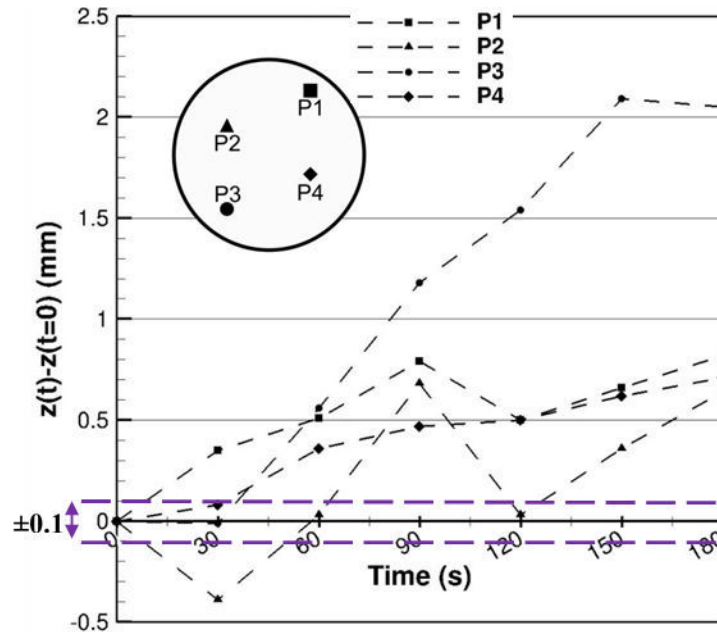
Figure 51: Relative temporal evolution (with t=0 as reference values) of the vertical displacement of four different points on the free surface extracted from data obtained using phase shift technique – Experiment 9
