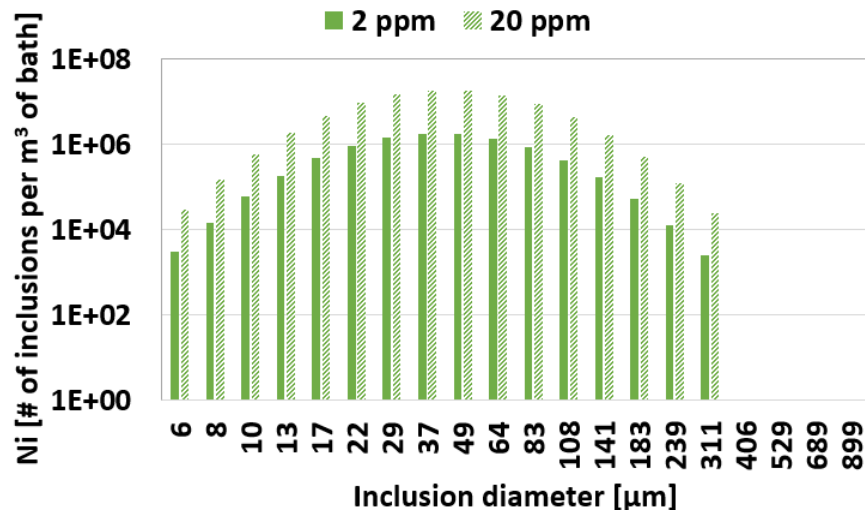
Figure 98: Initial inclusion psd for Exp. B – 2 ppm vs 20 ppm
