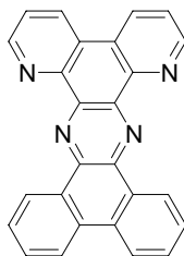
Figure 24 : Ligand dpdbphzH 2
