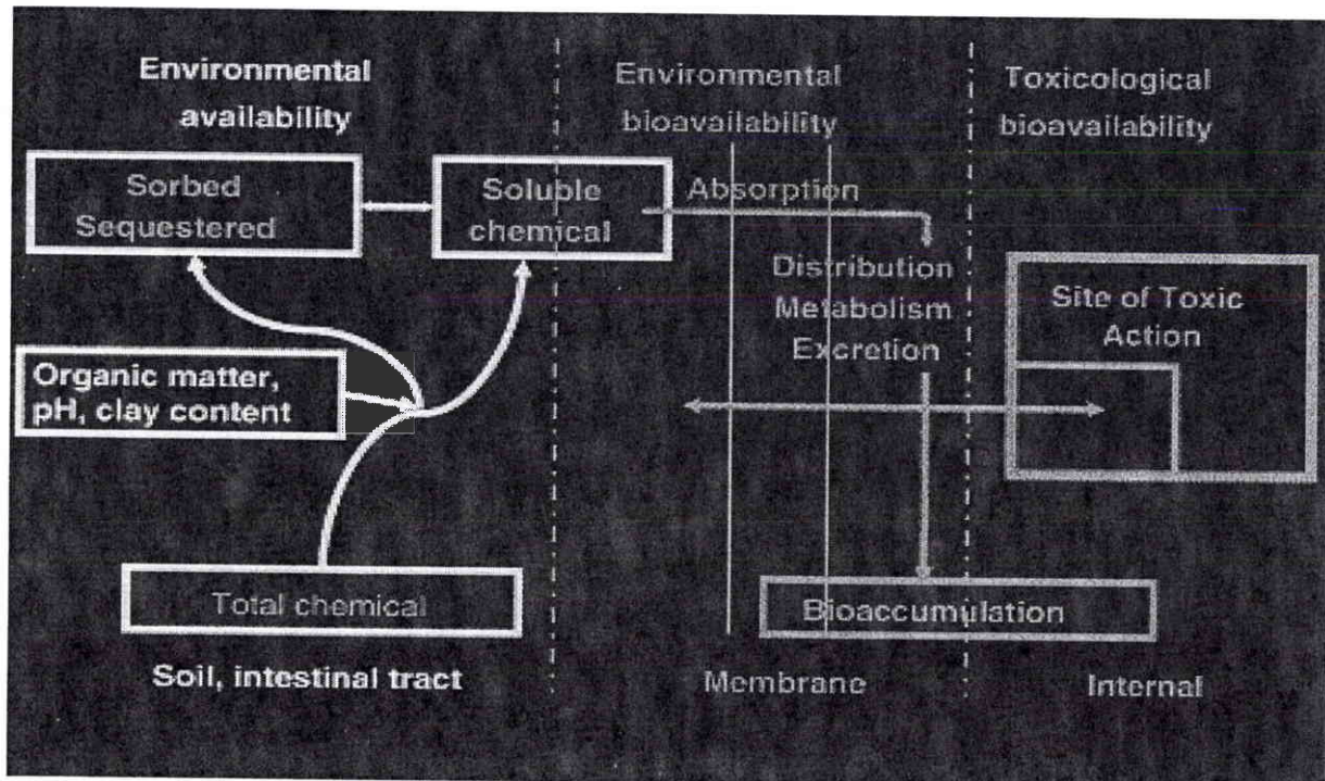
Fig. 8. Schematic model of bioavailability (from Lanno et al., 2004).
