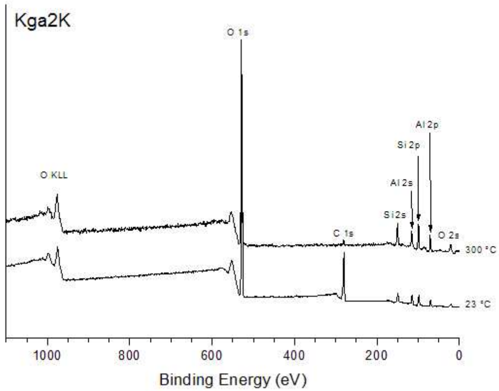
Figure 12. XPS Spectra for Kga2Na and Kga2K at room temperature (23°C) and heated at 300°C.
