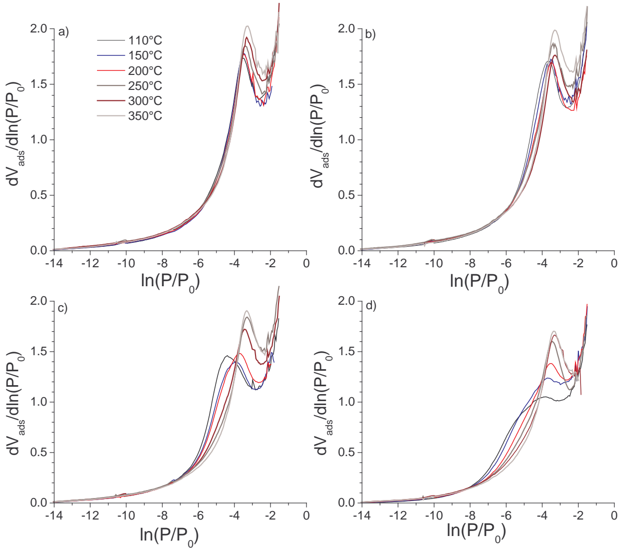
Figure 2. Evolution of the derivative adsorption isotherm with the increasing of temperature on exchanged kaolinite. a) Kga2Li, b) Kga2Na, c) Kga2K, and d) Kga2Cs.
