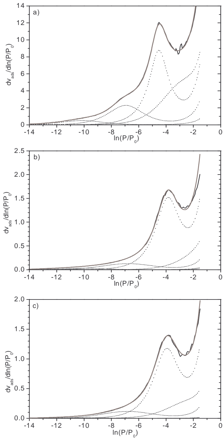
Fig. 3. Experimental derivative Ar adsorption obtained at 77 K on Na-clays: a) Illite [20, 21], b) Kga2 and c) Khg, with their decomposition using the Derivative Isotherm Summation (DIS) method and BET-Hill model.
