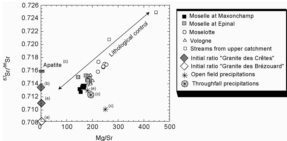
Figure V- 4: ^{87}\text{Sr}/^{86}\text{Sr} vs. Mg/Sr for rivers flowing on silicates compared to values reported for separated minerals, bulk bedrock and initial ^{87}\text{Sr}/^{86}\text{Sr} ratio of local granites (from "Granite des Crêtes" and "Granite de Brézouard" documented by (a) Bonhomme, 1967; (b) France-Lanord (1982); (c) Probst et al. (2000); (d) Aubert et al. (2001)). Biotite ranged between 2.293 and 5.865; Albite between 0.7420 and 0.7743; Apatite value is 0.71612; Bulk granites ranged between 0.7970 and 0.8384; Initial ratio between 0.7080 and 0.7137. Simulated silicate weathering end-member by Probst et al. (2000) is between 0.73629 and 0.74203. Mean open field precipitations are 0.7102 and 0.7128 documented respectively by (c) Probst et al. (2000) and (e) Chabaux et al. (2005). Mean throughfall precipitations is 0.7124 documented by (c) Probst et al. (2000).
