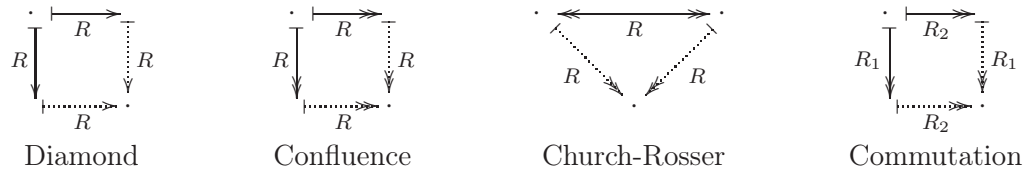
Figure 1.1: Properties of term rewriting
