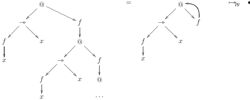
Figure 7.10: Reduction to black hole
