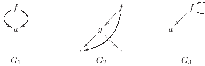
Figure 6.1: Some term graphs
