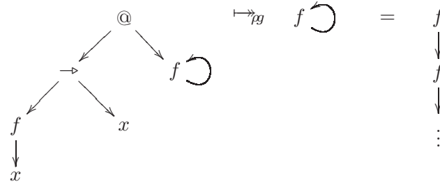
Figure 7.9: Reduction to a cyclic term
