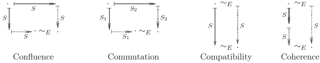
Figure 1.2: Properties of rewriting modulo \sim_E
