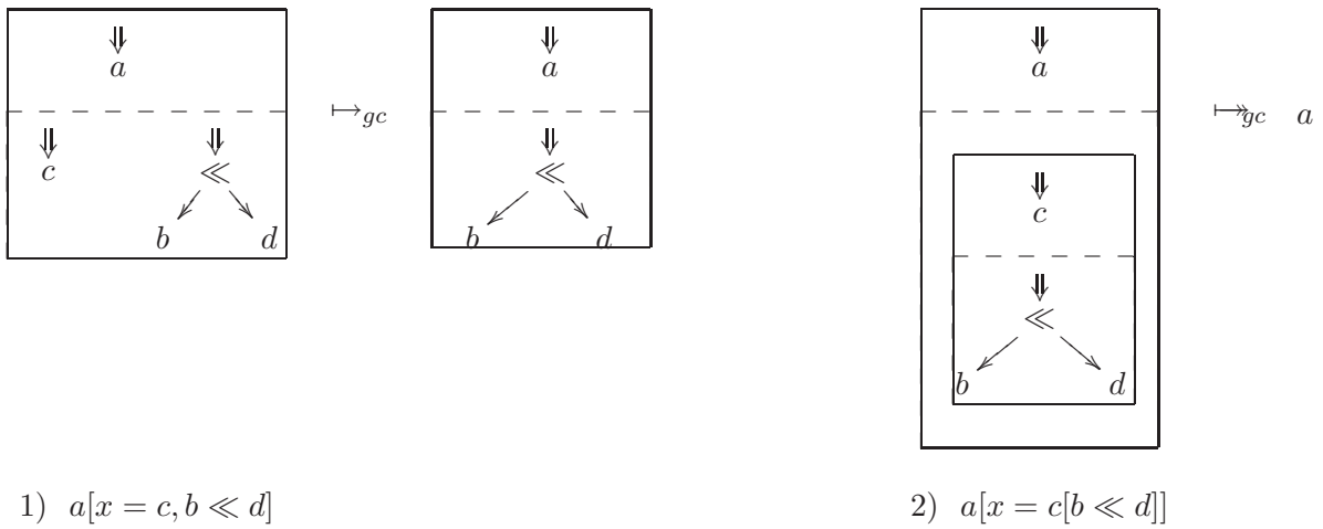
Figure 7.3: \rho_g -terms with matching constraints
