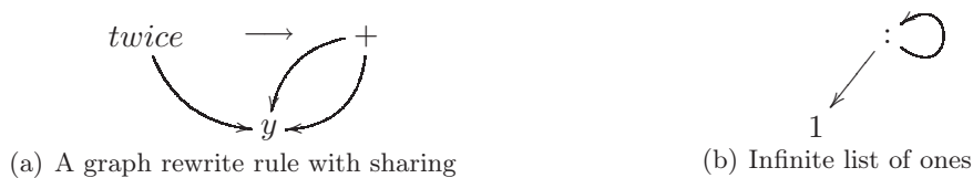
Figure 1: Examples of term graphs
