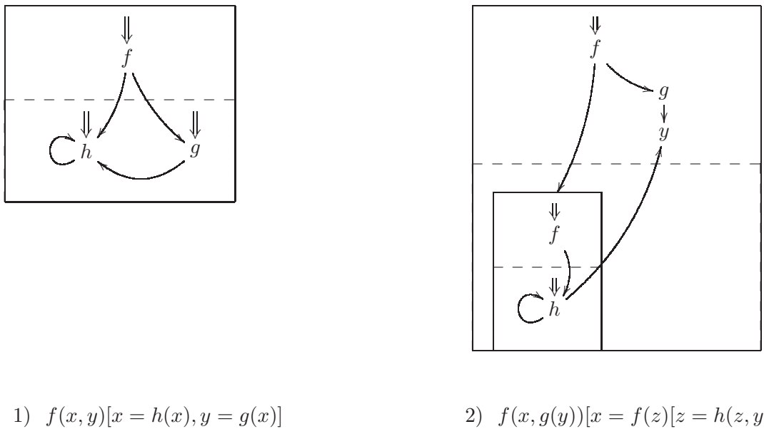
Figure 7.4: Graphs with cycles
