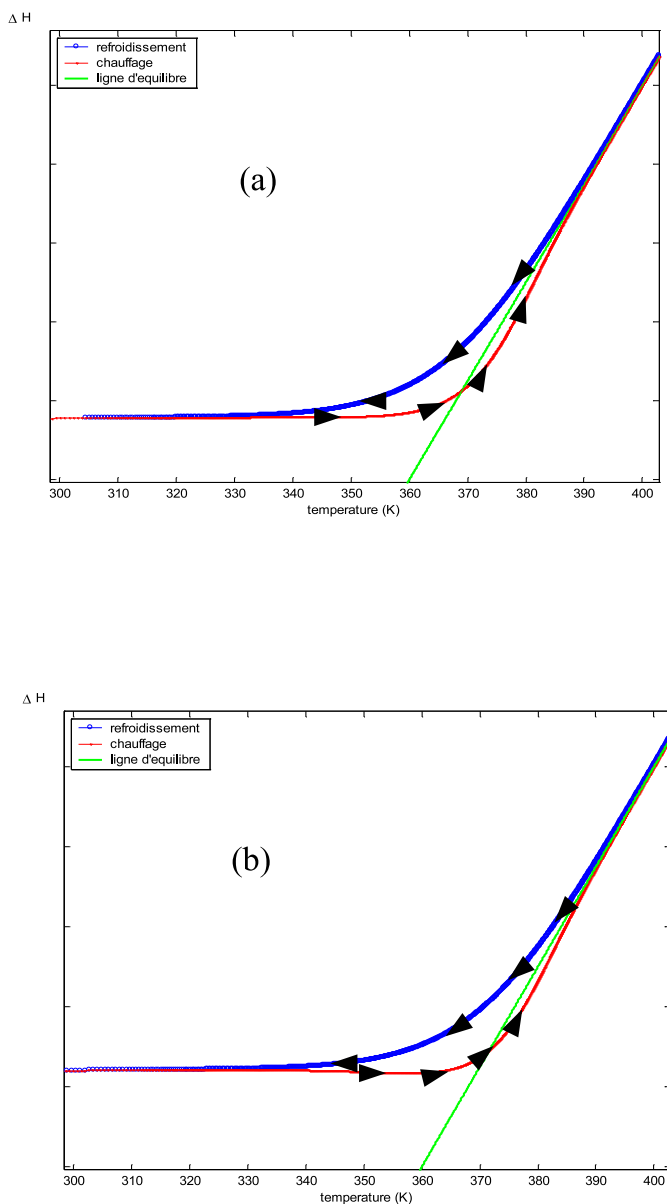
FIG. III.6: diagramme enthalpique
