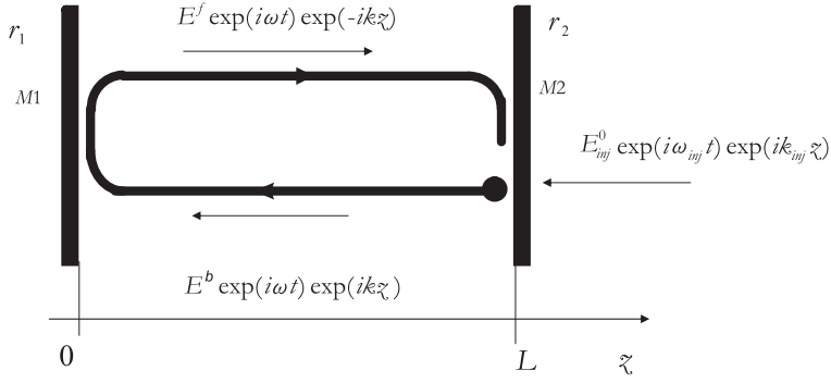
Figure 4.3.1: Schematic of a Fabry-Perot cavity for the modelling of a semiconductor laser under optical injection. The superscripts f and b denote the forward and backward internal travelling field waves.
