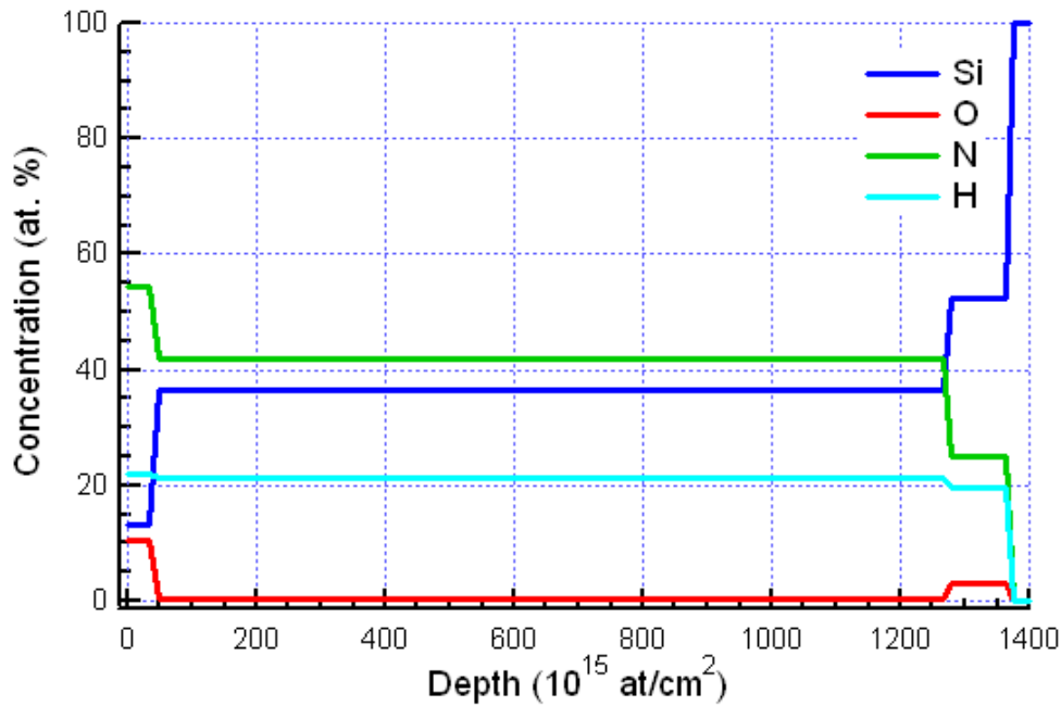
Fig. 29 : Evolution in the depth of the different compounds present in the silicon nitride layer deposited on a crystalline silicon substrate (100% on the right side). 100 \cdot 10^{15} at/cm ^2 represent 11 nm in this case.
