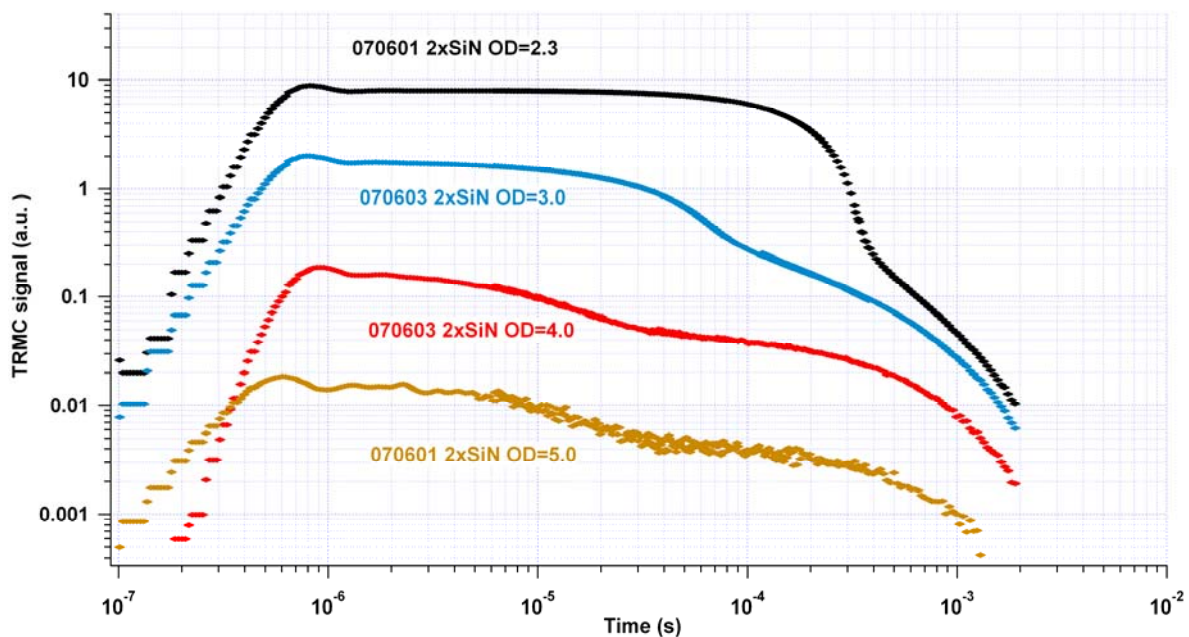
Fig. 90: TRMC signal induced by a 1064 nm laser pulse on a p-type crystalline silicon substrate (100 Ω.cm, 0.530 mm thick) covered on both side with SiN x (standard conditions, R=0.16) for 4 different intensities.
