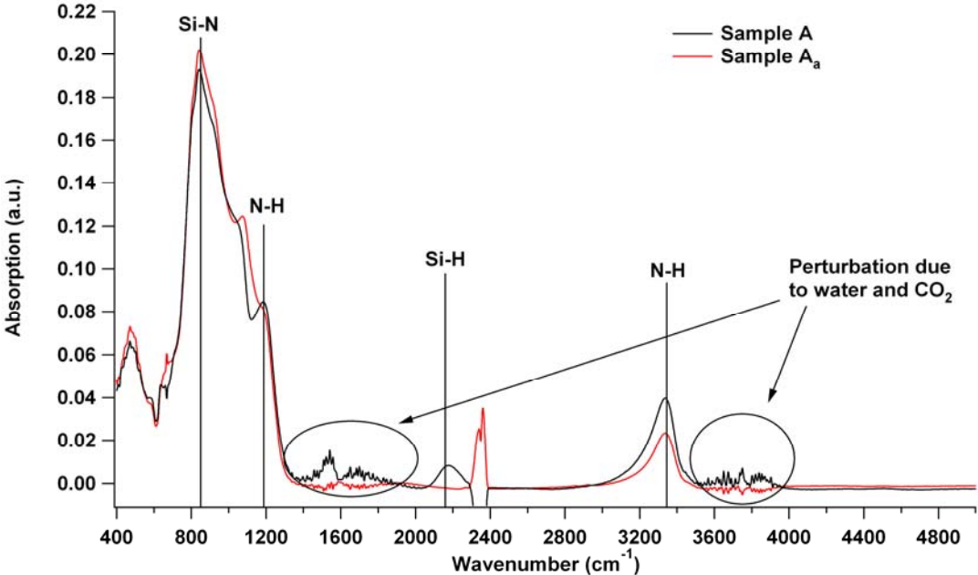
Fig. 81: Spectra of the sample A (with the lower ratio R (=0.16)) before the annealing at 900 °C and after (sample A a ). The diminution of the N-H and especially Si-H bonds are visible.
