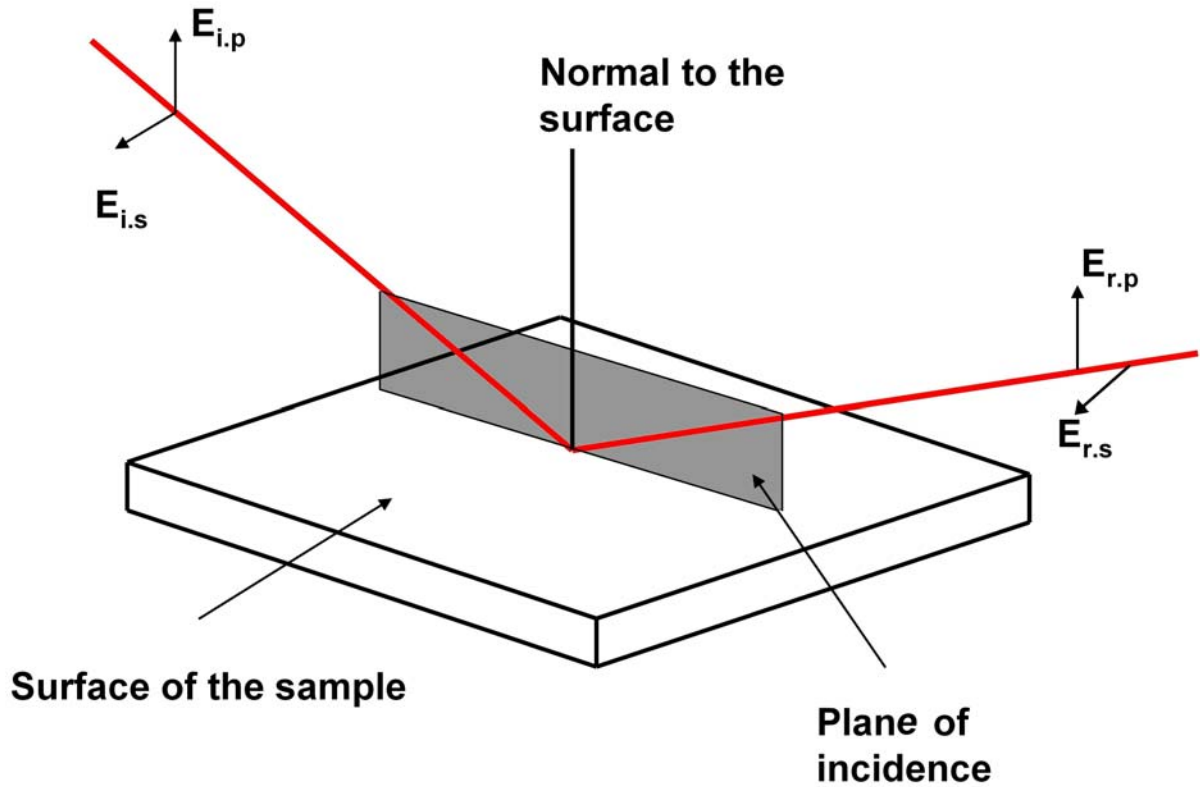
Fig. 3: Reflection of a polarized light on a sample. The incident components of the electric field are noticed E_{\perp,p} and E_{\parallel,s} . The reflected one are E_{r,p} and E_{r,s} . The plan of incidence corresponds to the plan containing the normal to the surface and the incident beam.
