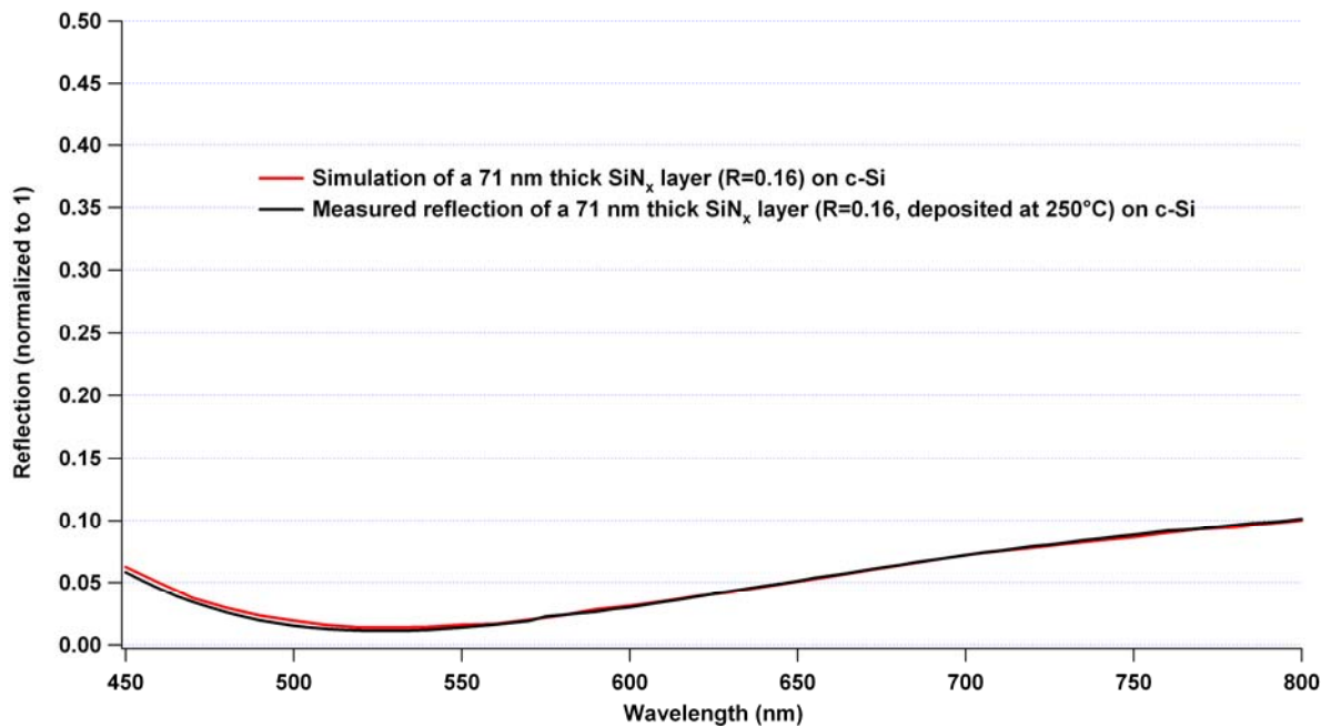
Fig. 20: Simulation (red line) and measure (black line) of the reflection of a crystalline silicon substrate covered with SiN x . The silicon nitride is in this case 71 nm thick and was deposited at 250°C (R=0.16, n 630 =1.808)
