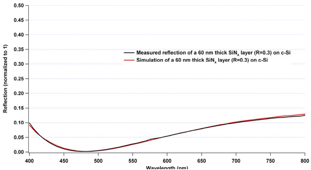
Fig. 21: Simulation (red line) and measure (black line) of the reflection of a crystalline silicon substrate covered with SiN x . The silicon nitride is in this case 60 nm thick and was deposited under standard condition (R=0.3, n 630 =1.912)
