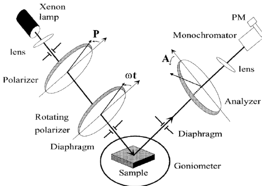
Fig. 16 : Scheme of the PRPSE ellipsometer used at the University of Metz to do the ellipsometric measurements. The Xenon lamp is the light source and PM the photomultiplier which will count the photons of each wavelength coming onto it. The first polarizer is fixed, it polarizes linearly the incoming light and suppresses the residual polarization of the source.
