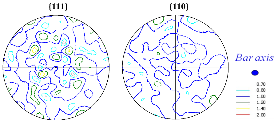
Figure 13:- \{111\}_\gamma and \{110\}_\gamma pole figure of the sample tempered for 2 hrs at 1050°C
