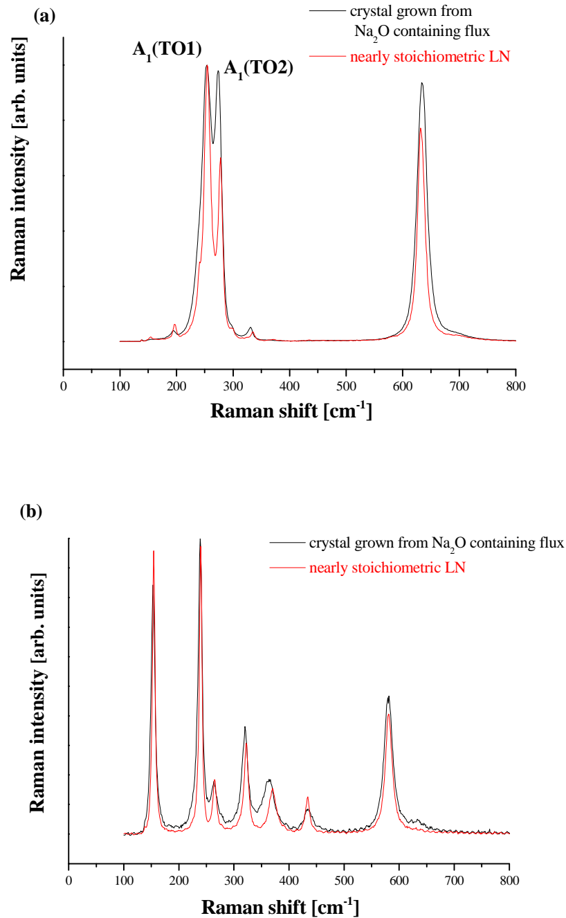
Figure 3.28. Comparison of the Raman spectra of the \text{Na}_2\text{O} containing crystal and the nearly stoichiometric LN ( \text{Li}_2\text{O} content equal to 49.74 mol%) measured in y(zz)y (a) and y(xz)y (b) configurations by He-Ne (633 nm) laser
