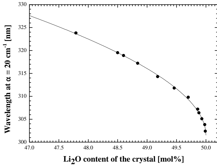
Figure 1.6. Calibration curve between the crystal composition and the UV absorption edge position [38], \text{Li}_2\text{O} content of the samples was determined by using calibration based on the phase matching temperature of the optical second harmonic generation.
