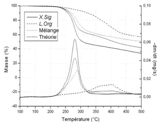
Figure IV.8: Courbes TG-DTG du mélange X.Sig - L.Org
