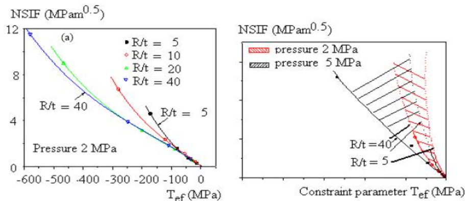
Fig. 6a NSIF versus T_{eff} relation ship ( R/t = 20 ; internal pressure, P = 2-5 MPa)
