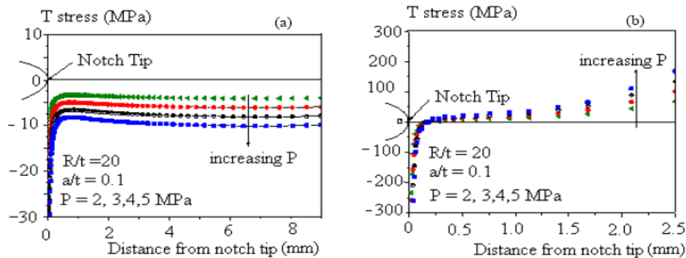
Fig. 3 Evolution of the T-stress values for a longitudinal surface notch under different internal pressure ( P = 20, 30, 40 and 50 bars) for (a) small and (b) length notches ( R/t=20 ).
