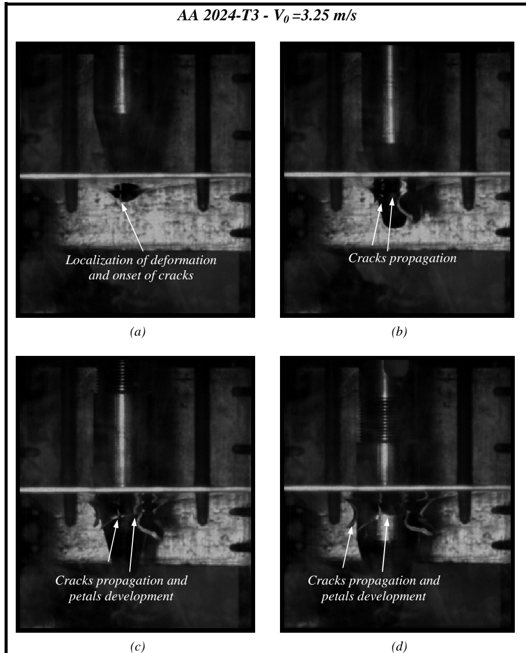
Fig. 4.54. Different stages of the perforation process for V_0=3.25 \text{ m/s} and T_0=288\text{K} . (a) Localization of deformation and onset of cracks. (b) Cracks progression and generation of petals. (c) Development of petalling. (d) Complete passage of the impactor and petalling failure mode.
