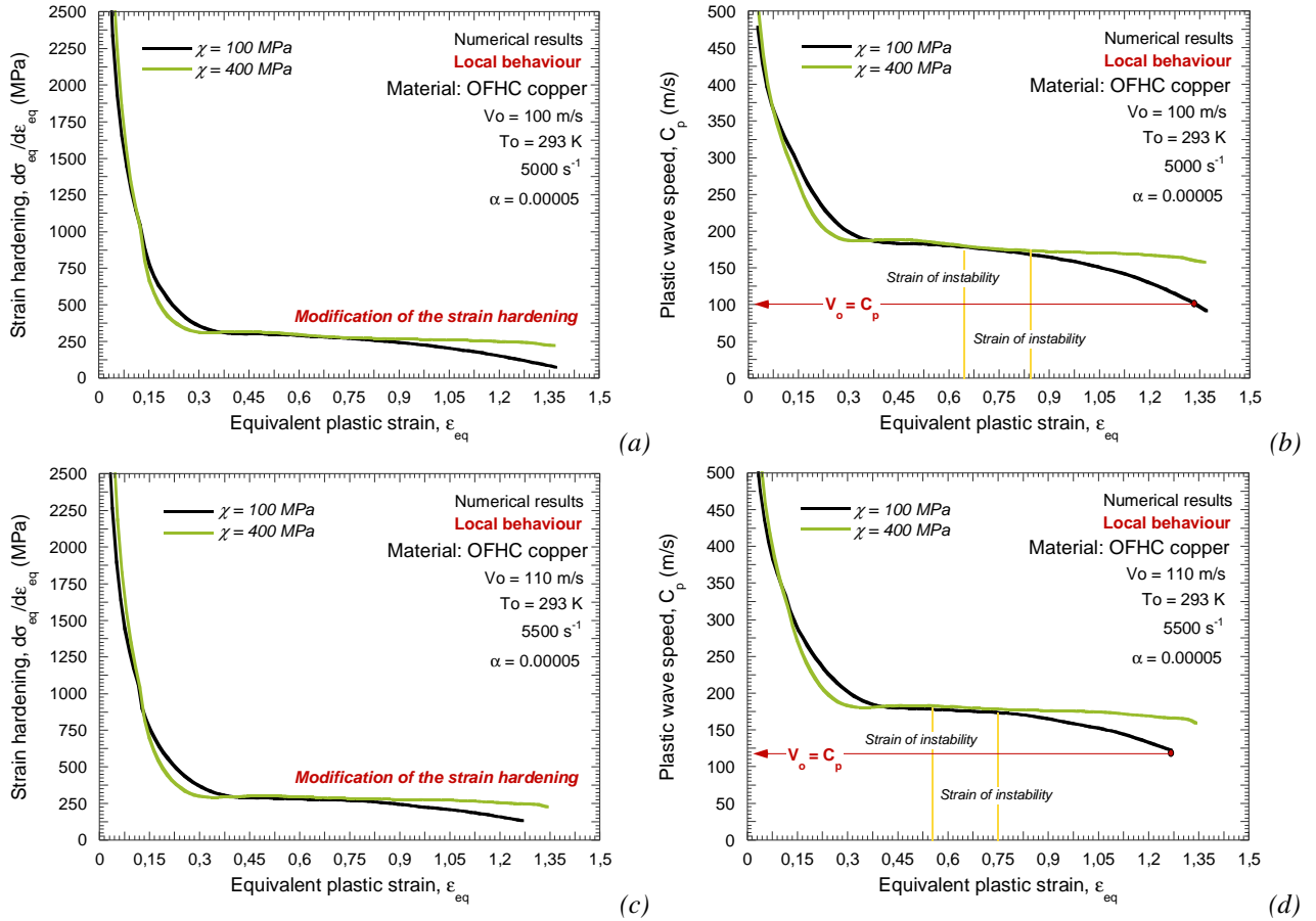
Fig. 3.41. (a) Strain hardening and (b) plastic wave celerity evolution as a function of plastic deformation in the necking zone for \chi=100\text{ MPa} and \chi=400\text{ MPa} at V_0=100\text{ m/s} .
