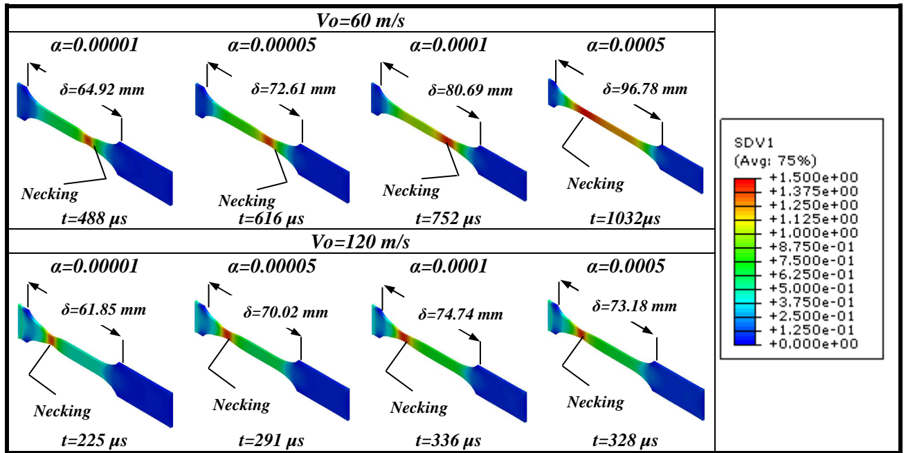
Fig. 3.58. Plastic strain contours at failure time for different values of \alpha and two impact velocities, V_0=60 \text{ m/s} and V_0=120 \text{ m/s} .
