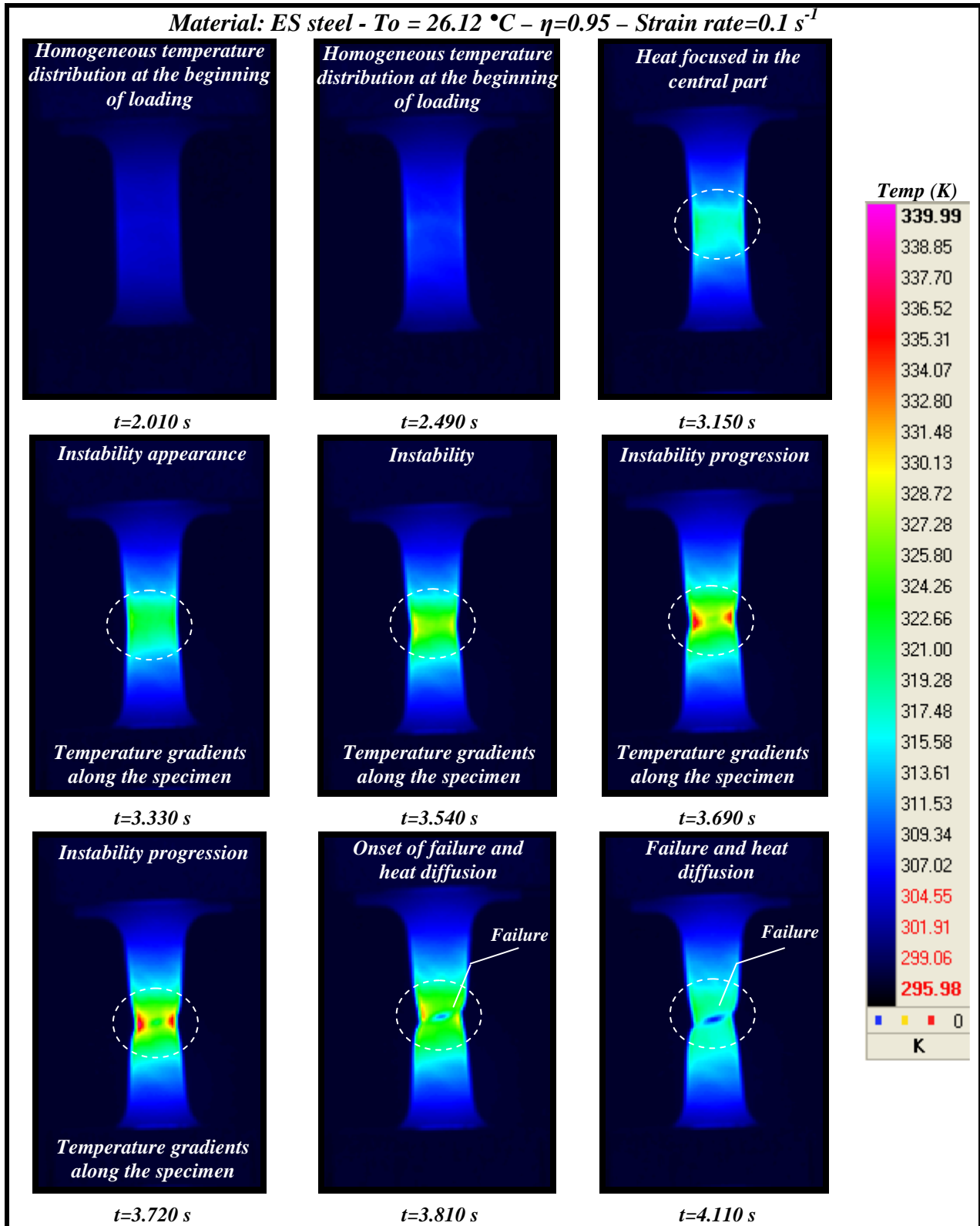
Fig. 4.11. Temperature contours during loading. Picture resolution 320 \times 256 pixels.
