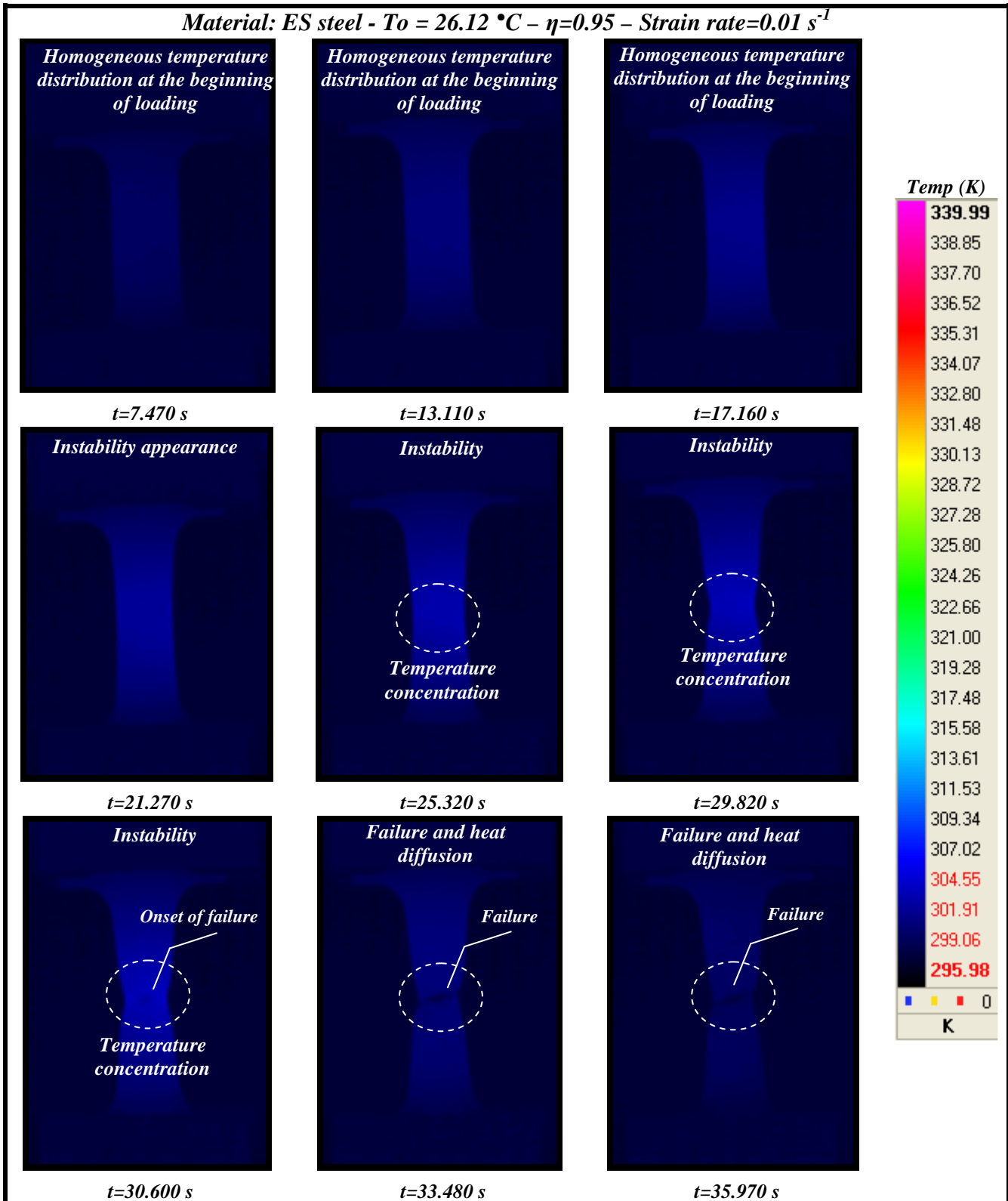
Fig. 4.7. Temperature contours during loading. Picture resolution 320×256 pixels.
