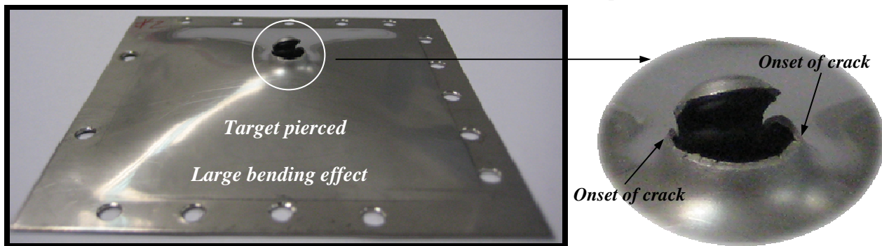
Fig. 5.25. Pierced target, steel AISI 304, V_0=3.0 m/s at room temperature.
