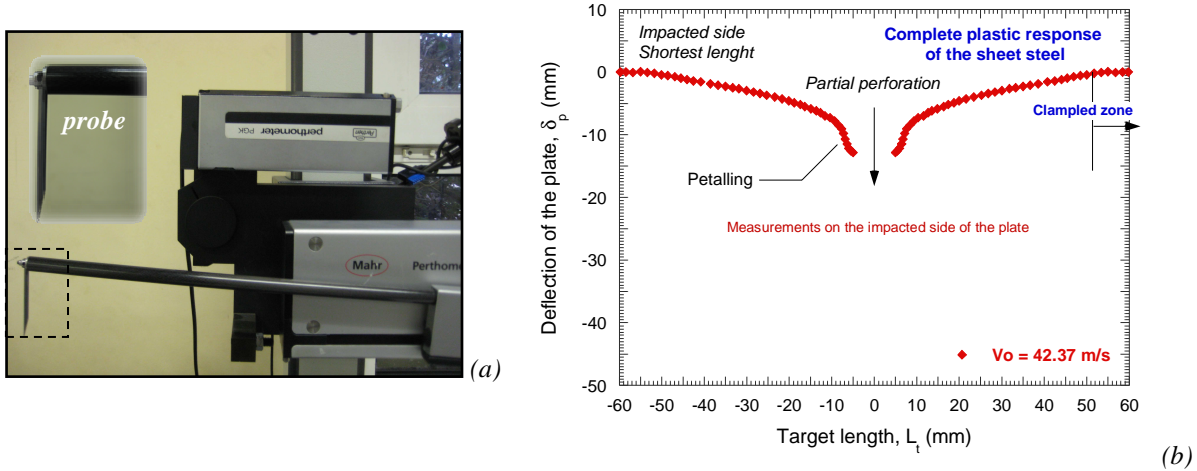
Fig. 4.17. (a) Profilometer used to measure the permanent deflection of the plates. (b) Measurement of the post-mortem deflection of the target.
