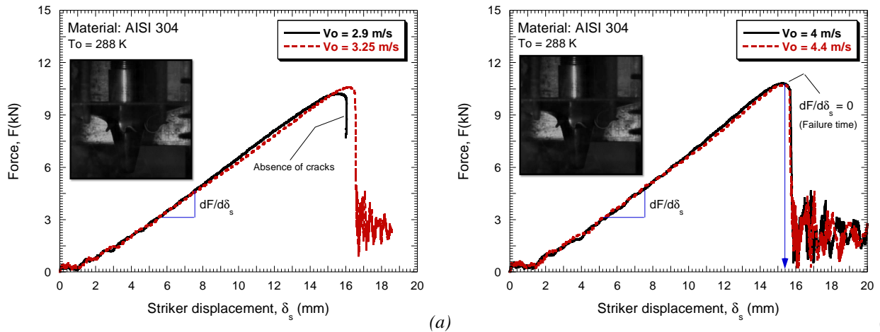
Fig. 5.29. Evolution of the impact force as a function of the striker displacement for different impact velocities at room temperature.
