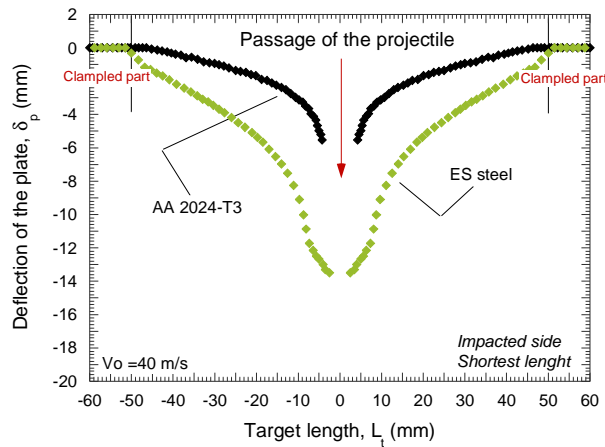
Fig. 4.63. Post-mortem deflection of the target for AA 2024-T3 and steel ES for V_o \approx 40 \text{ m/s} .
