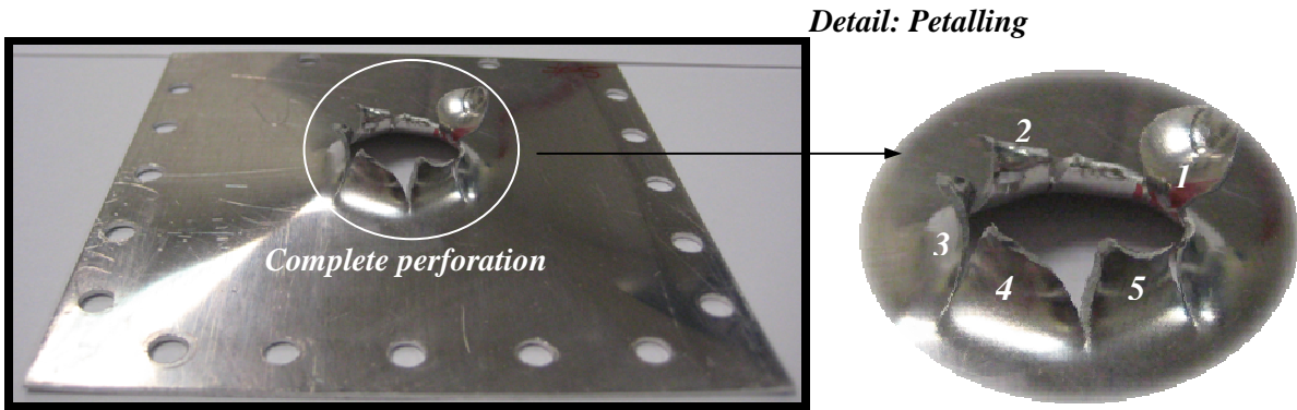
Fig. 4.55. Petalling failure mode for V_0 = 4.0 m/s and T_0 = 213 K.
