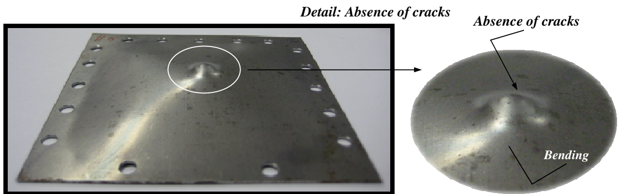
Fig. 5.56. Petalling failure mode, steel TRIP 1000 , V_0 = 2.9 \text{ m/s} and T_0 = 213 \text{ K} .
