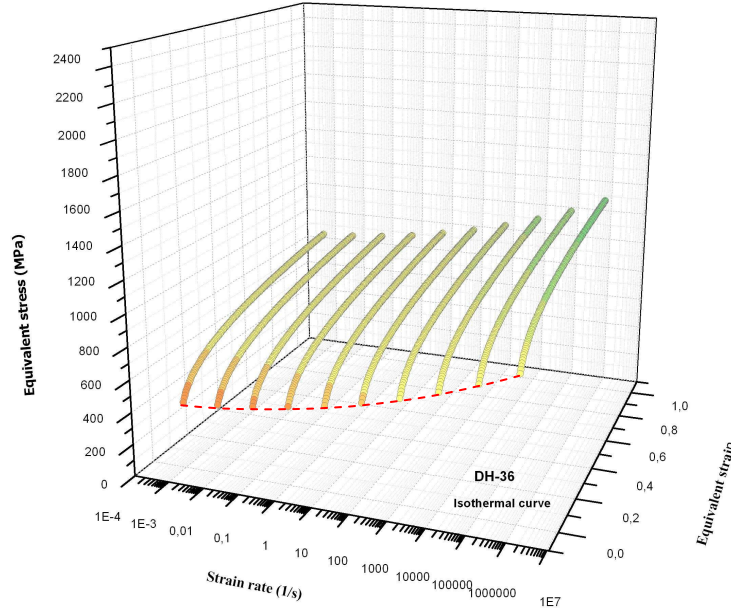
Fig. 2.7. Description of the flow stress of the steel DH-36 provided by the RK model within wide ranges of strain and strain rate.
