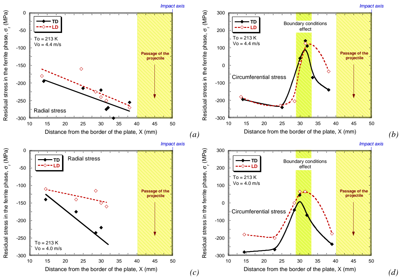
Fig. 5.60. Residual stress in ferrite along the distance from the border to the center of the plate for different initial impact velocities at T_0 = 213 \text{ K} . (a)-(b) V_0 = 4.4 \text{ m/s} , (c)-(d) V_0 = 4.0 \text{ m/s} .
