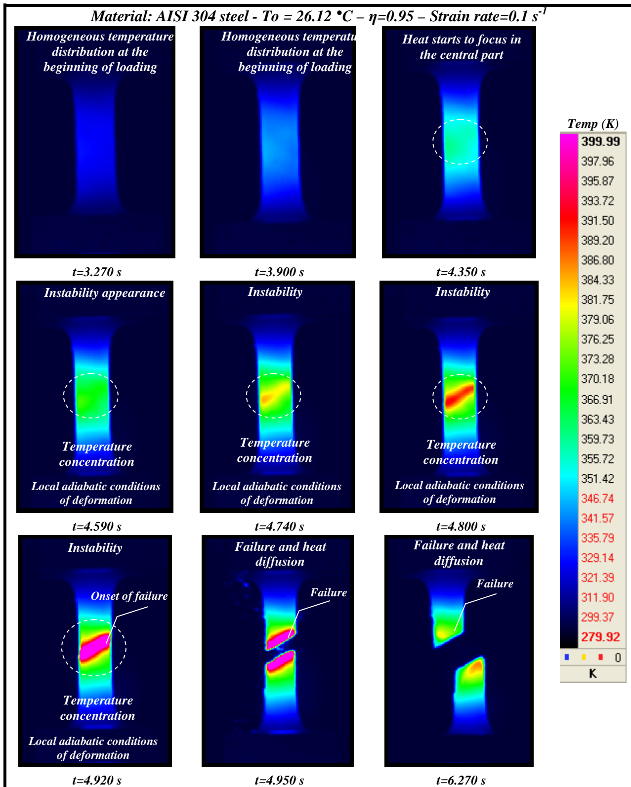
Fig. 5.17. Temperature contours during loading. Picture resolution 320 \times 256 pixels.
