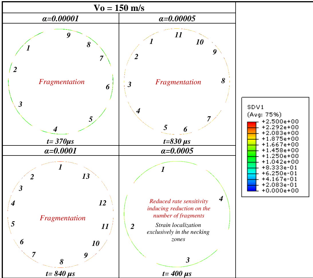
Fig. 3.52. Plastic strain contours at failure time and ring fragmentation for different values of \alpha and V_0=150 m/s.
