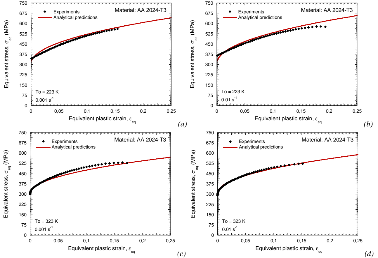
Fig. 4.44. Flow stress evolution versus plastic strain for different strain rates and temperatures and comparison with analytical predictions.
