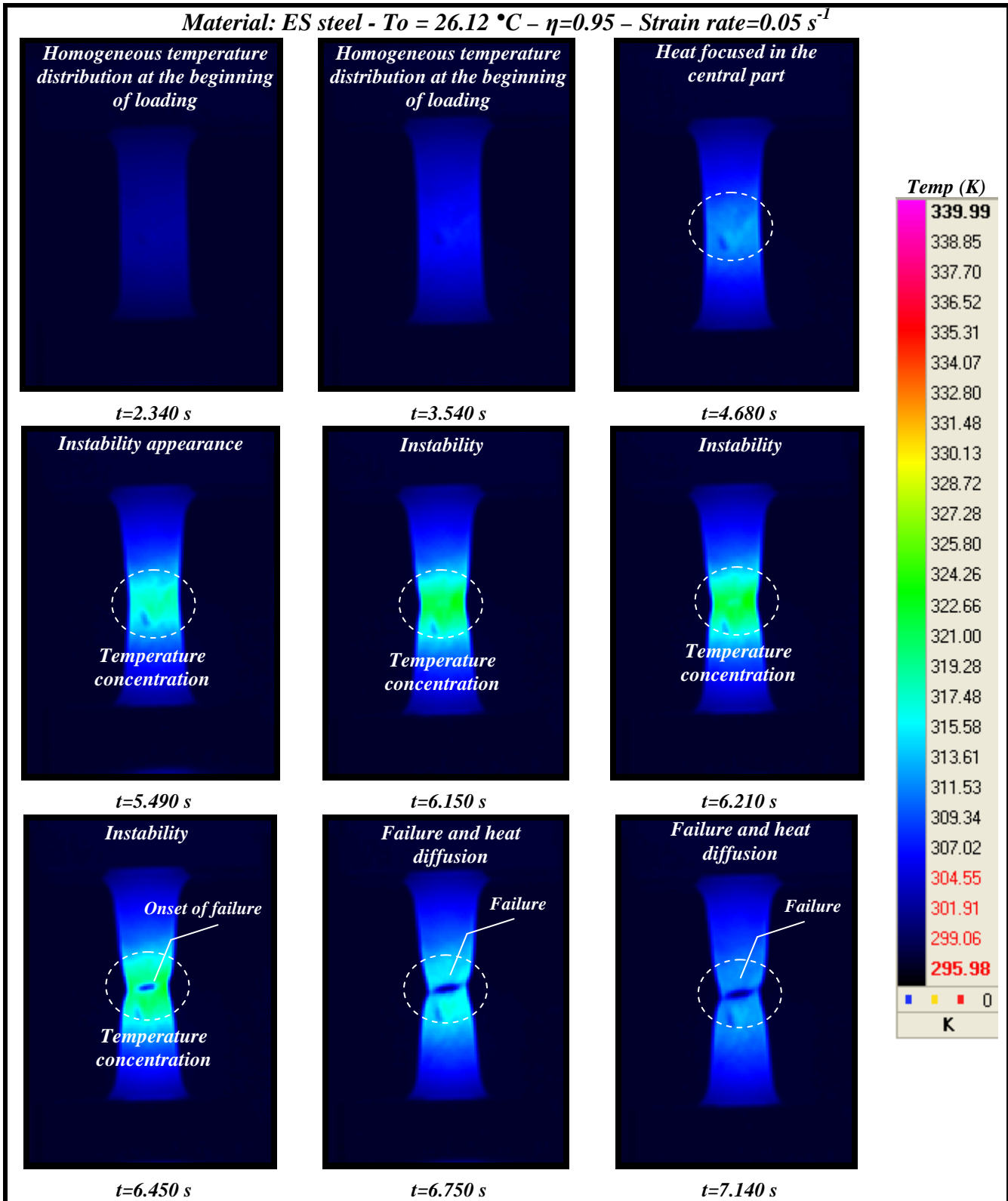
Fig. 4.9. Temperature contours during loading. Picture resolution 320 \times 256 pixels.
