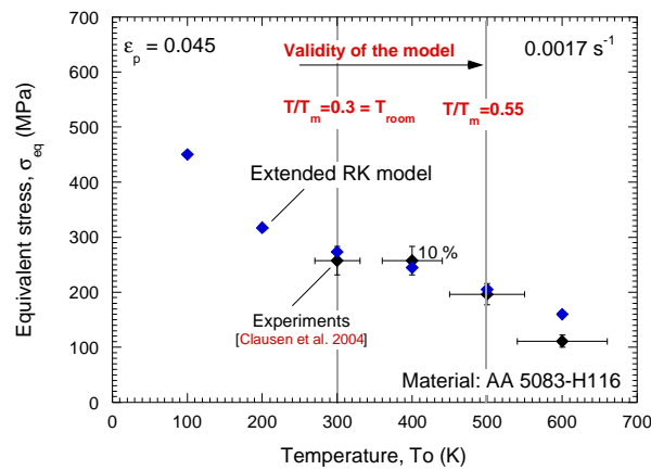
Fig. 2.41. Description of the temperature sensitivity by the extended RK model and comparison with experiments for \epsilon_p=0.045 and 0.0017 \text{ s}^{-1} [Clausen et al. 2004].
