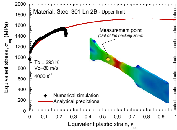
Fig. 3.67. Comparison between numerical results and analytical predictions for the material models considered. Conventional dynamic tension test, V_0=80 m/s.
