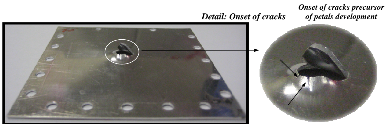
Fig. 4.52. Petalling failure mode for V_0 = 1.0 m/s and T_0 = 288 K.
