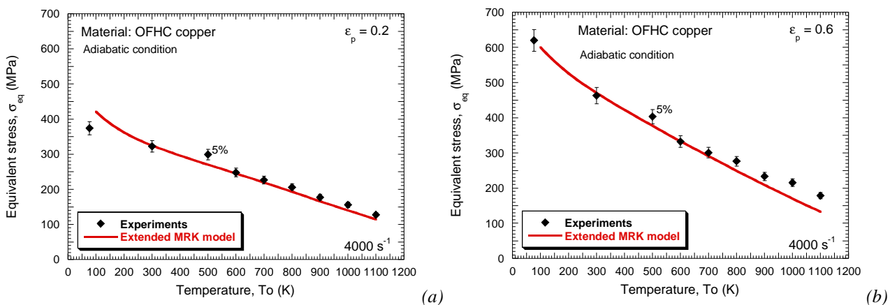
Fig. 2.33. Temperature sensitivity description using the extended MRK model and comparison with experiments at 4000 \text{ s}^{-1} . (a) \epsilon_p=0.2 , (b) \epsilon_p=0.6 [Nemat-Nasser and Li 1998].
