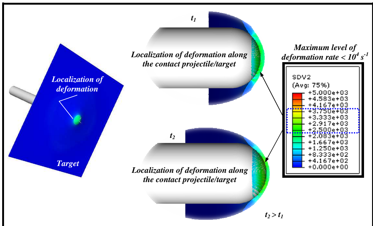
Fig. 4.30. Numerical estimations of strain rate contours during perforation, V_0 = 50 \text{ m/s} .
