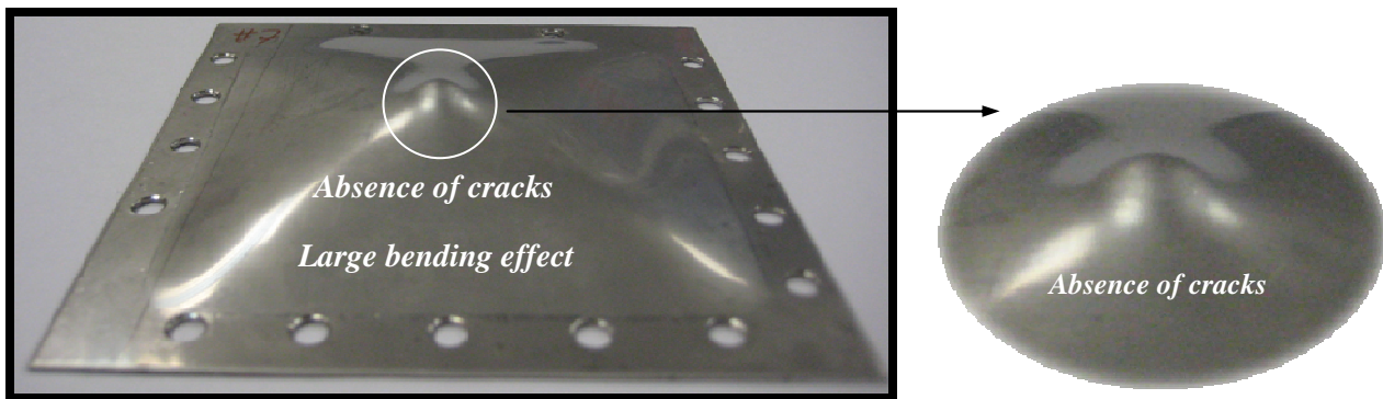
Fig. 5.24. Absence of cracks, steel AISI 304, V_0=2.9 m/s at room temperature.
