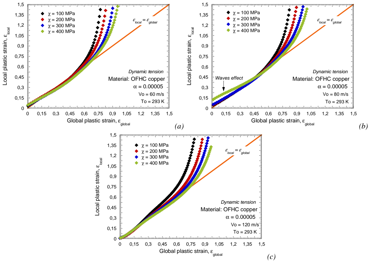
Fig. 3.37. Evolution of the local plastic strain as a function of the global plastic strain for different values of \chi . (a) V_0 = 60 m/s, (b) V_0 = 80 m/s, (c) V_0 = 120 m/s.
