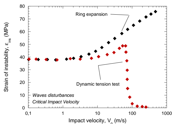
Fig. 3.2. Strain of instability as a function of impact velocity for ring expansion problem and dynamic tension test [Hu and Daehn 1996].
