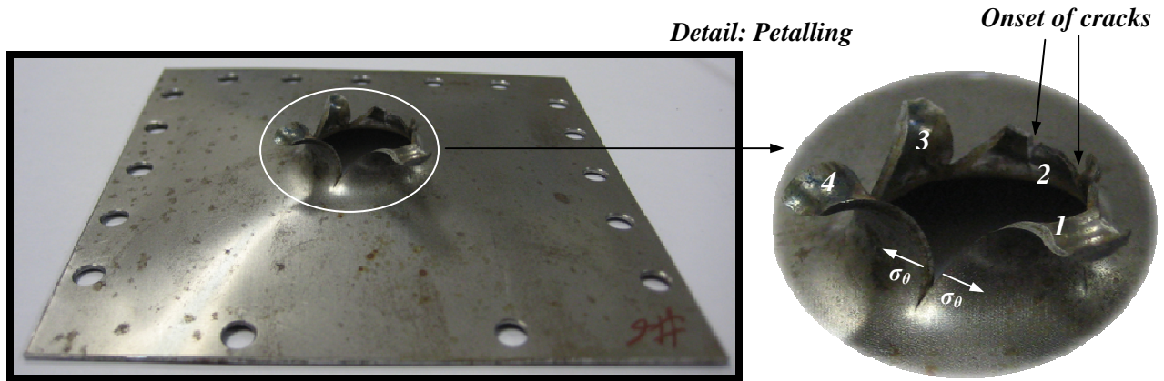
Fig. 5.55. Petalling failure mode, steel TRIP 1000 , V_0 = 3.7 \text{ m/s} and T_0 = 213 \text{ K} .
