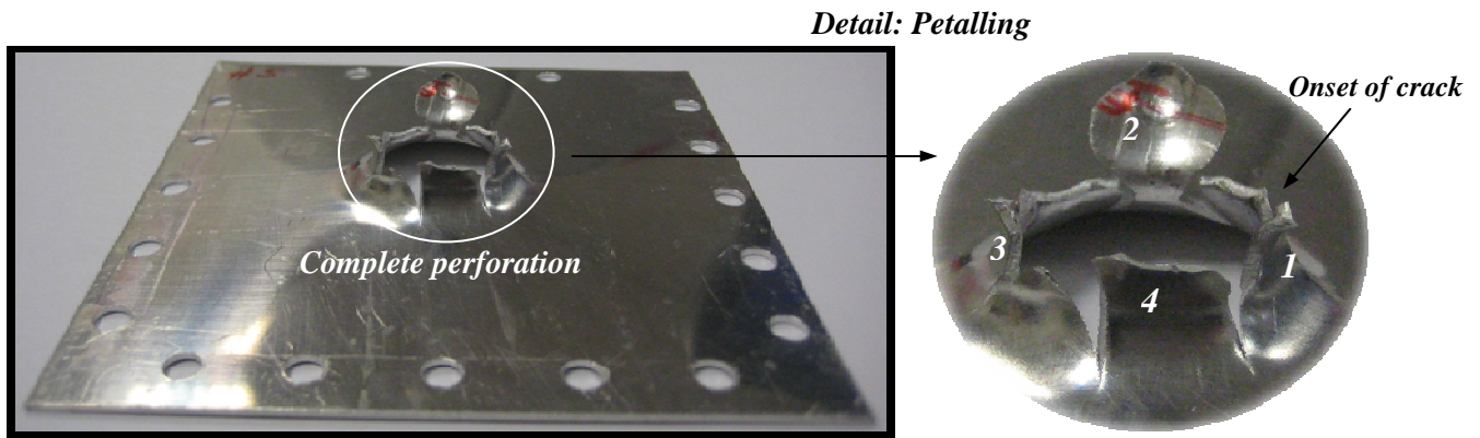
Fig. 4.51. Petalling failure mode for V_0 = 2.0 m/s and T_0 = 288 K.
