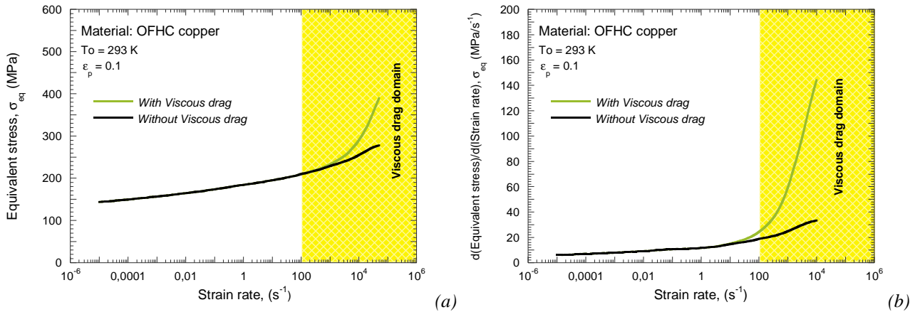
Fig. 3.12. (a) Flow stress evolution versus strain rate of annealed OFHC copper predicted by MRK and extended MRK models. (b) Rate sensitivity of annealed OFHC copper predicted by MRK and extended MRK models.
