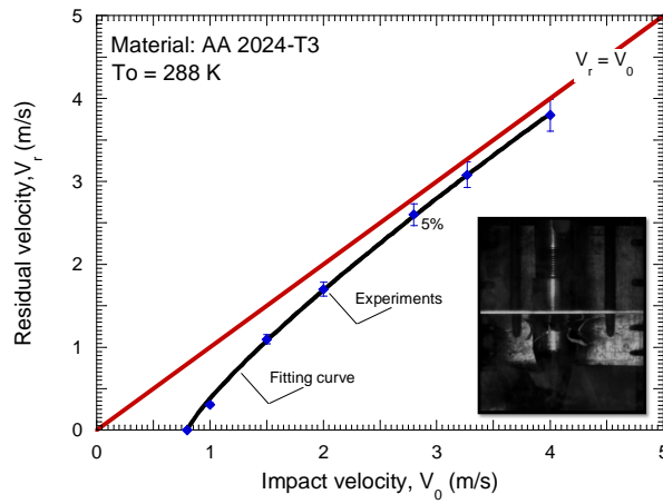
Fig. 4.48. Residual velocity versus impact velocity at room temperature.
