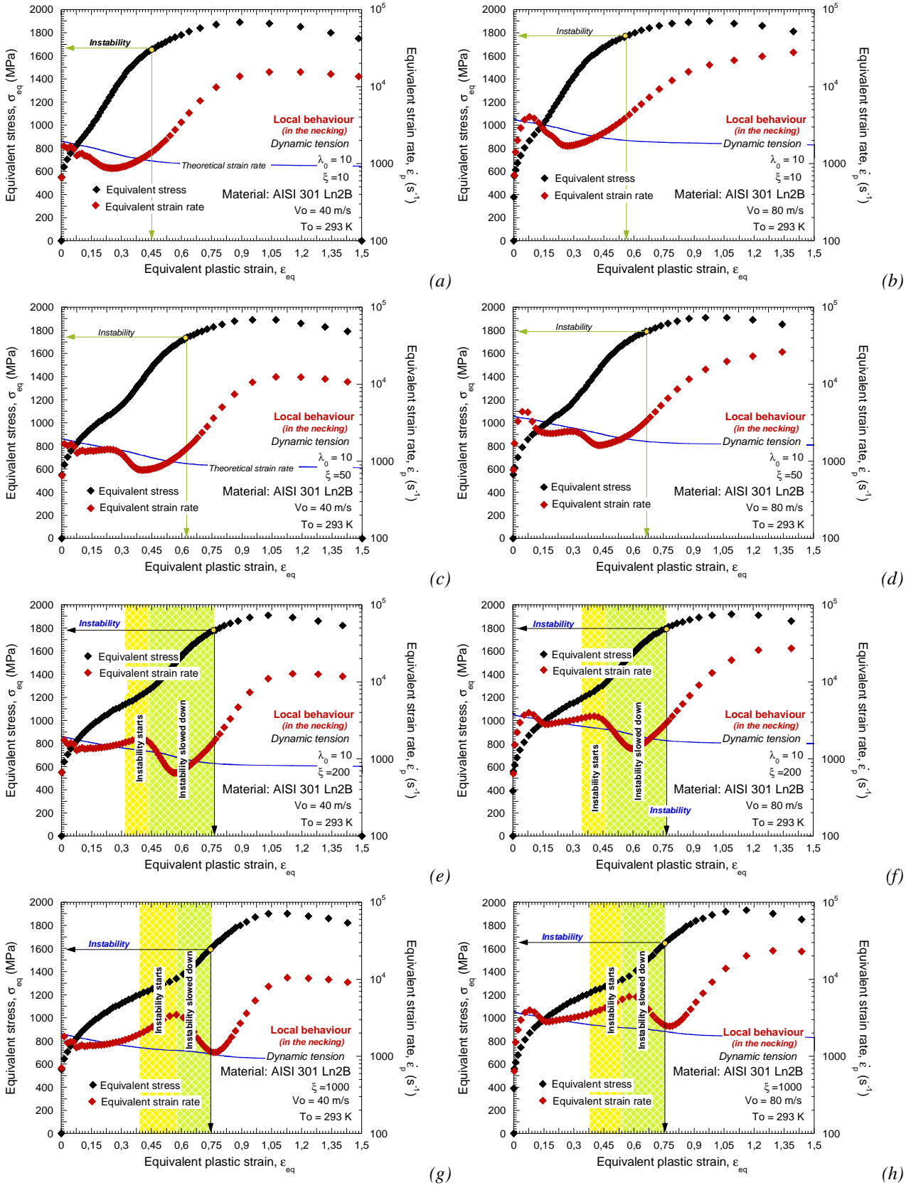
Fig. 3.86. Evolution of the strain rate and the flow stress in the necking as a function of plastic strain for all the values of \xi considered and different impact velocities.
