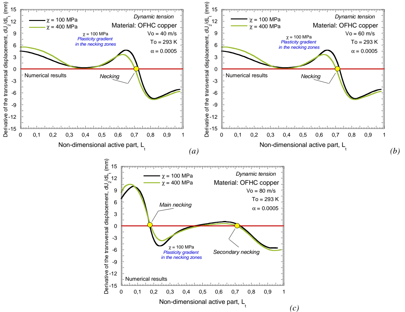
Fig. 3.44. Derivative of the transversal displacement of the active part of the specimen for different values of \chi . (a) V_0=40 m/s, (b) V_0=60 m/s, (c) V_0=80 m/s.
