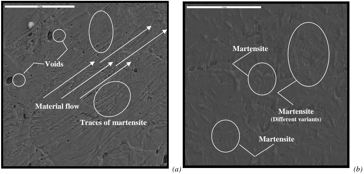
Fig. 5.38. SEM micrographies of petals in AISI 304 impacted plates, V_0=78.15 m/s.
