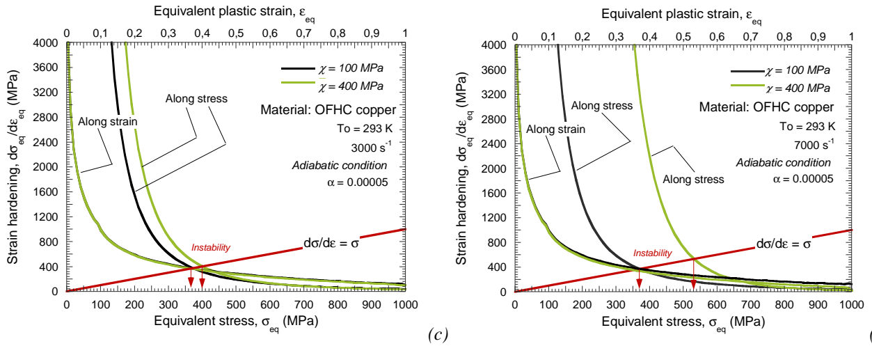
Fig. 3.31. (a)-(b) Flow stress evolution as a function of the plastic strain for different values of \chi . (c)-(d) Strain hardening evolution versus plastic strain and stress for different values of \chi .
