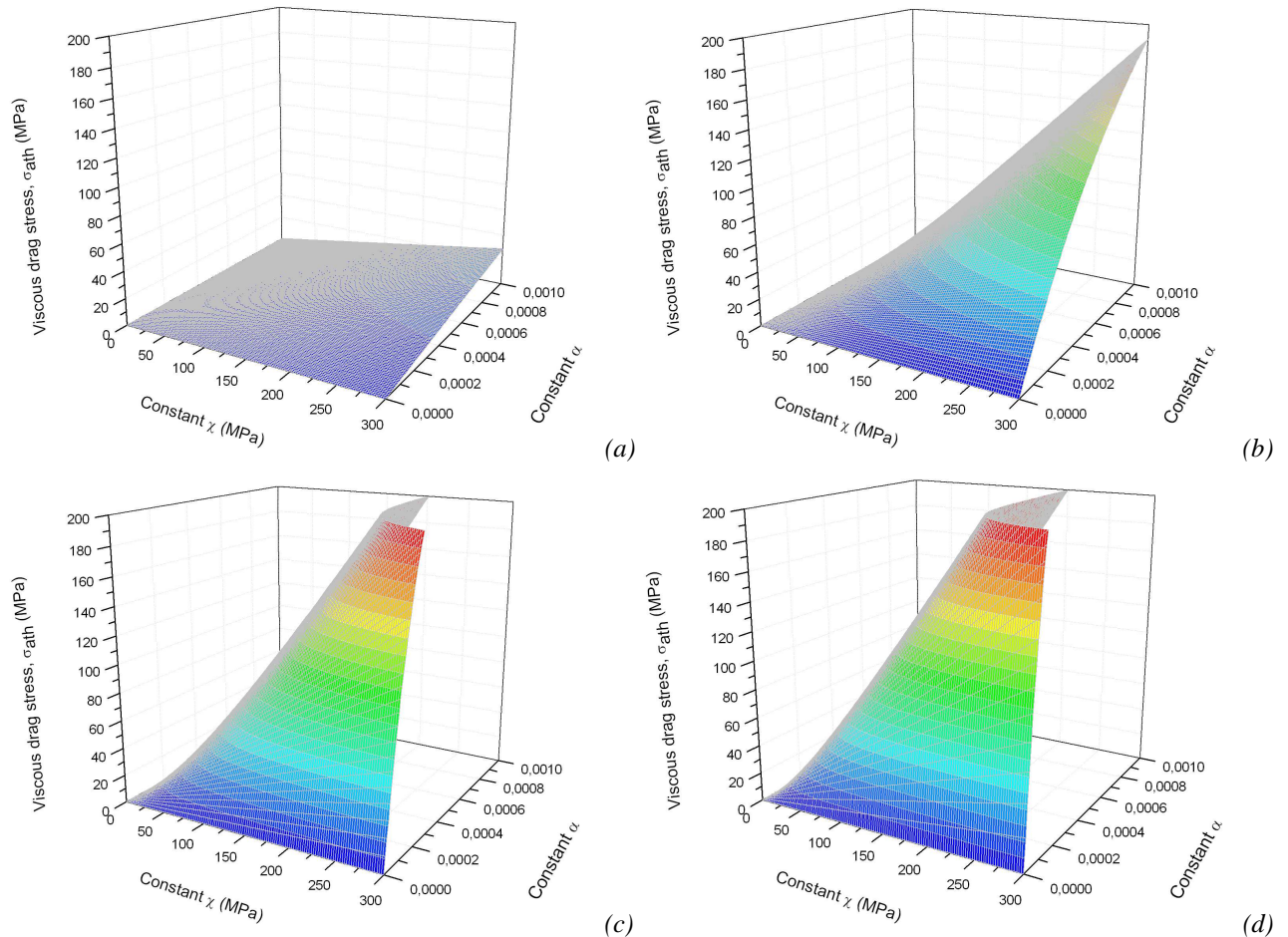
Fig. 2.28. Evolution of the viscous drag component as a function of \chi and \alpha for different strain rate levels. (a) 100 \text{ s}^{-1} , (b) 1000 \text{ s}^{-1} , (c) 5000 \text{ s}^{-1} , (d) 10000 \text{ s}^{-1} .
