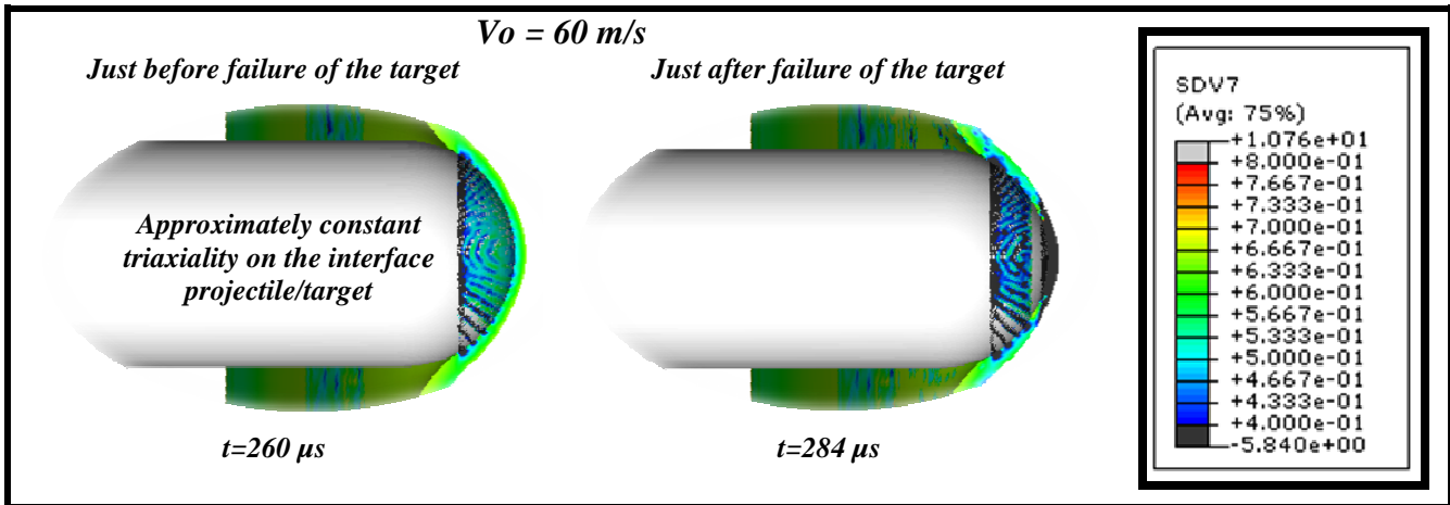
Fig. 4.34. Numerical estimation of triaxiality contours during perforation. V_0 = 60 \text{ m/s}
