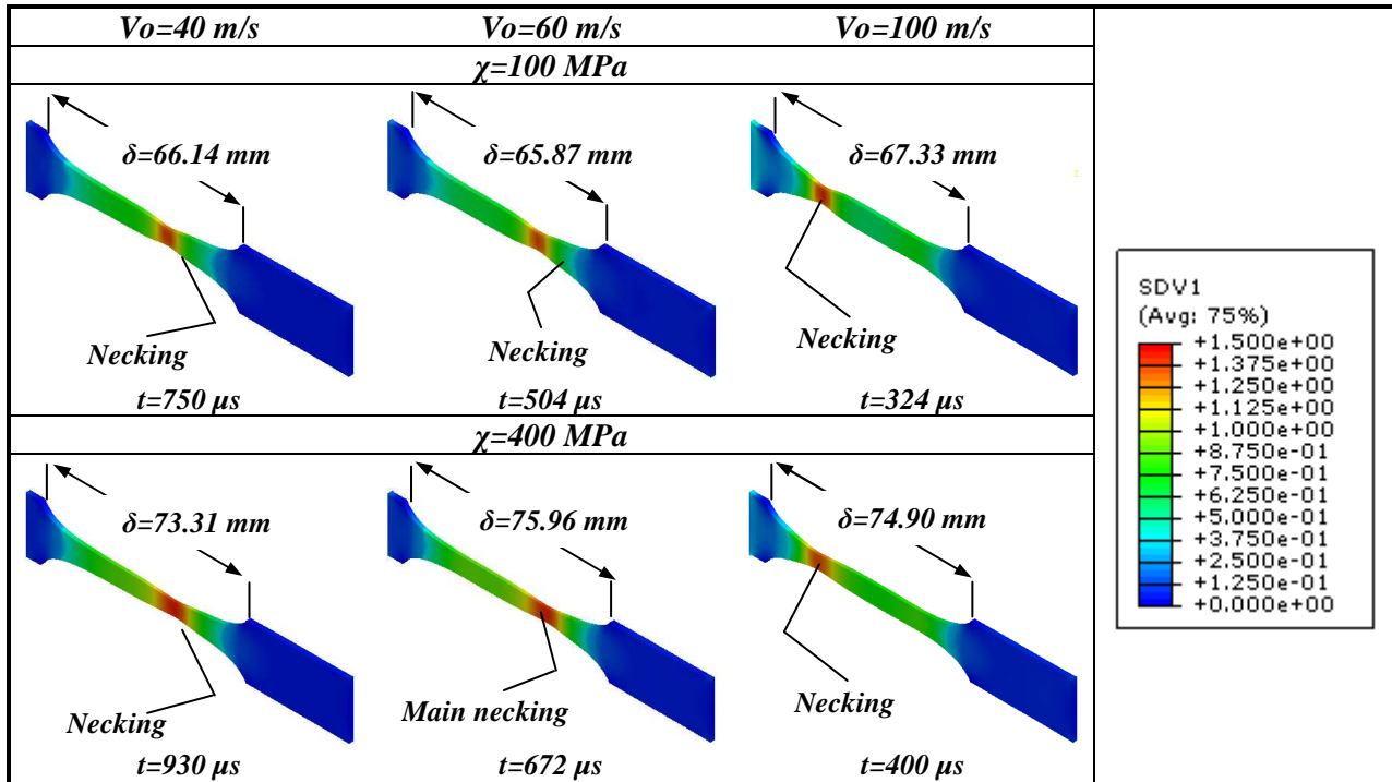
Fig. 3.42. Plastic strain contours at failure time for \chi=100\text{ MPa} and \chi=400\text{ MPa} and different impact velocities.
