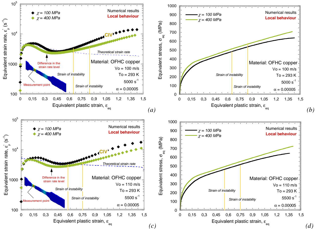
Fig. 3.40. Evolution (a) of strain rate and (b) stress as a function of plastic deformation in the necking zone for \chi=100 MPa and \chi=400 MPa at V_0=100 m/s and V_0=110 m/s.
