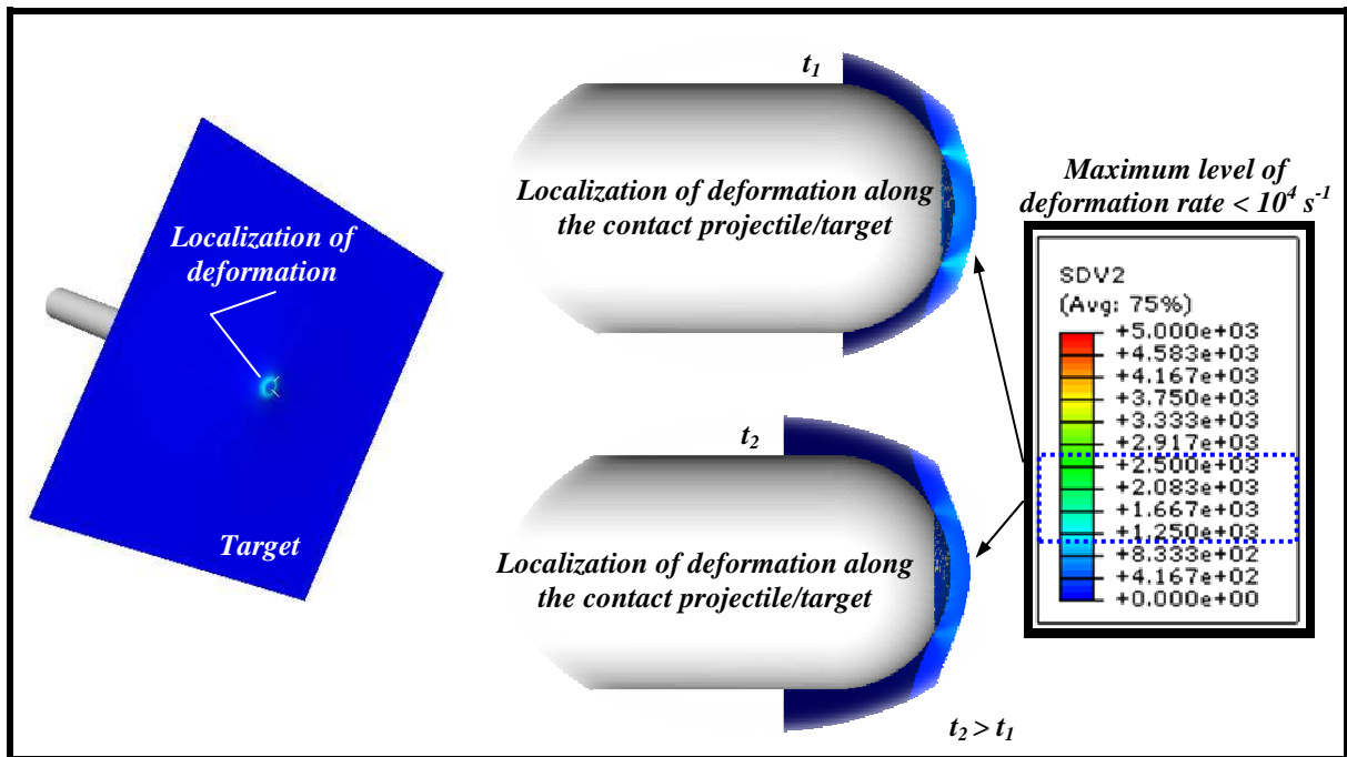
Fig. 4.29. Numerical estimations of strain rate contours during perforation, V_0 = 25 \text{ m/s} .
