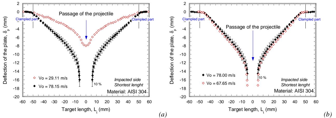
Fig. 5.37. Post-mortem deflection of the target for different initial impact velocities.
