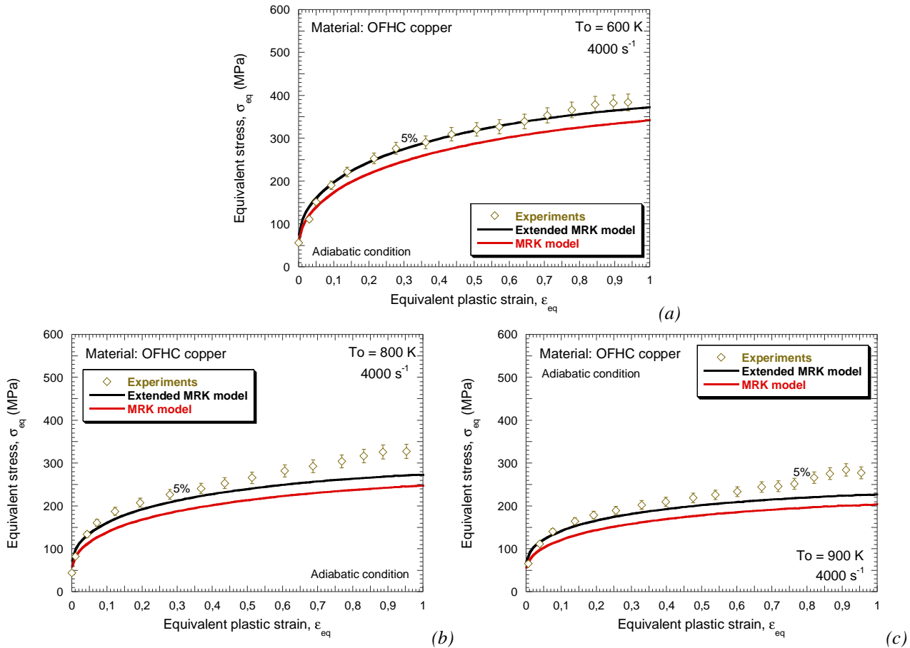
Fig. 2.32. Description of the flow stress evolution as a function of plastic strain by original and extended MRK models and comparison with experiments at 4000 \text{ s}^{-1} . (a) T_0=600 \text{ K} , (b) T_0=800 \text{ K} , (c) T_0=900 \text{ K} [Nemat-Nasser and Li 1998].
