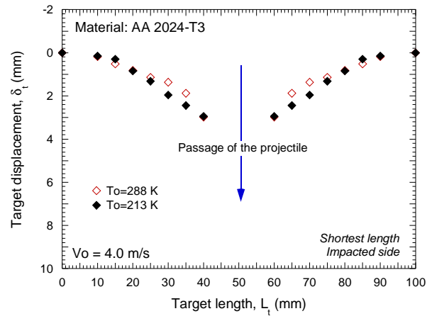
Fig. 4.59. Permanent bending of the target for different impact velocities and initial temperatures
