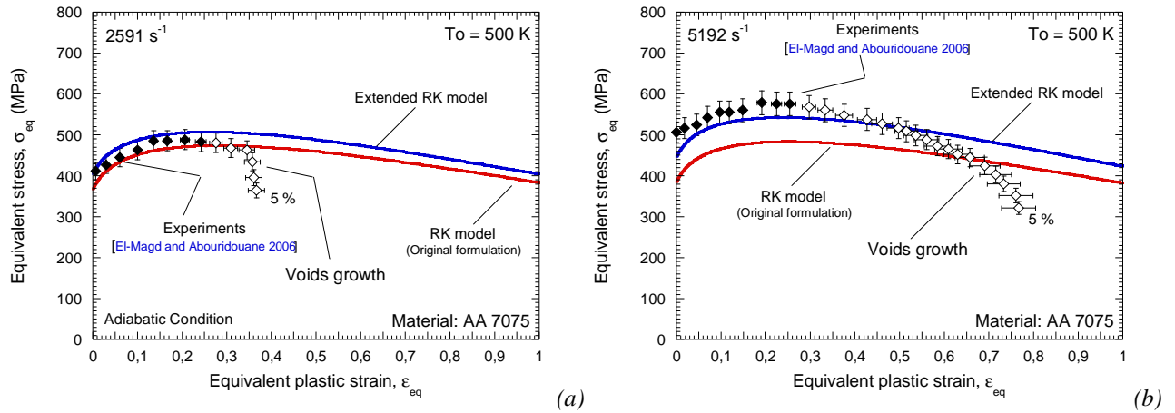
Fig. 2.35. Description of the flow stress evolution versus plastic strain by original and extended RK models and comparison with experiments at T_0 = 500 K [El-Magd and Abouridouane 2006]. (a) 2591 s ^{-1} , (b) 5192 s ^{-1} .
