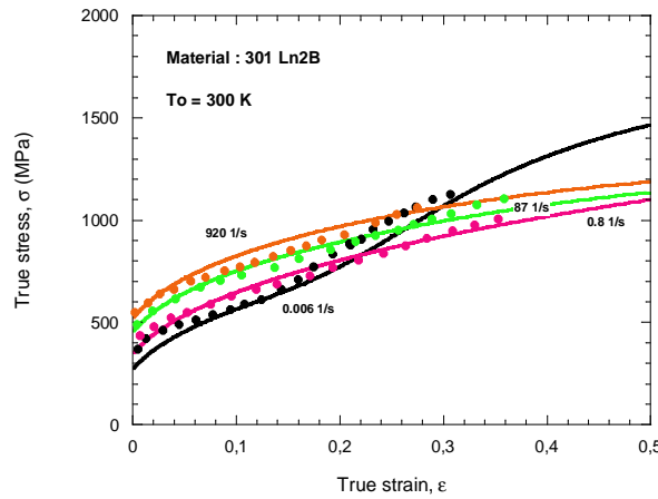
Fig. 2.51. Analytical predictions of the constitutive relation (solid lines) and comparison with experimental results [Larour et al. 2006].
