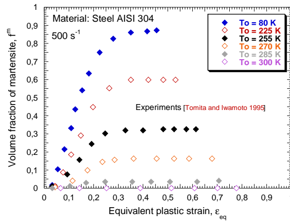
Fig. 2.45. Volume fraction of martensite as a function of plastic deformation for different initial temperatures. Strain rate = 500 \text{ s}^{-1} [Tomita and Iwamoto 1995].
