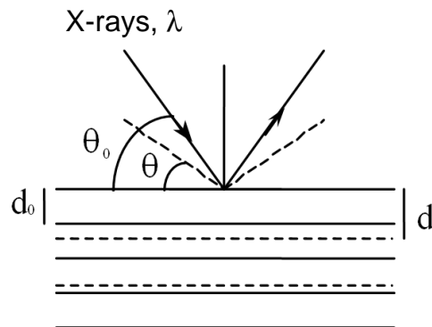
Fig. 5.1. Principle of X-ray diffraction ( d_0 and \theta_0 are respectively the lattice spacing and the Bragg angle corresponding to a stress free state).
