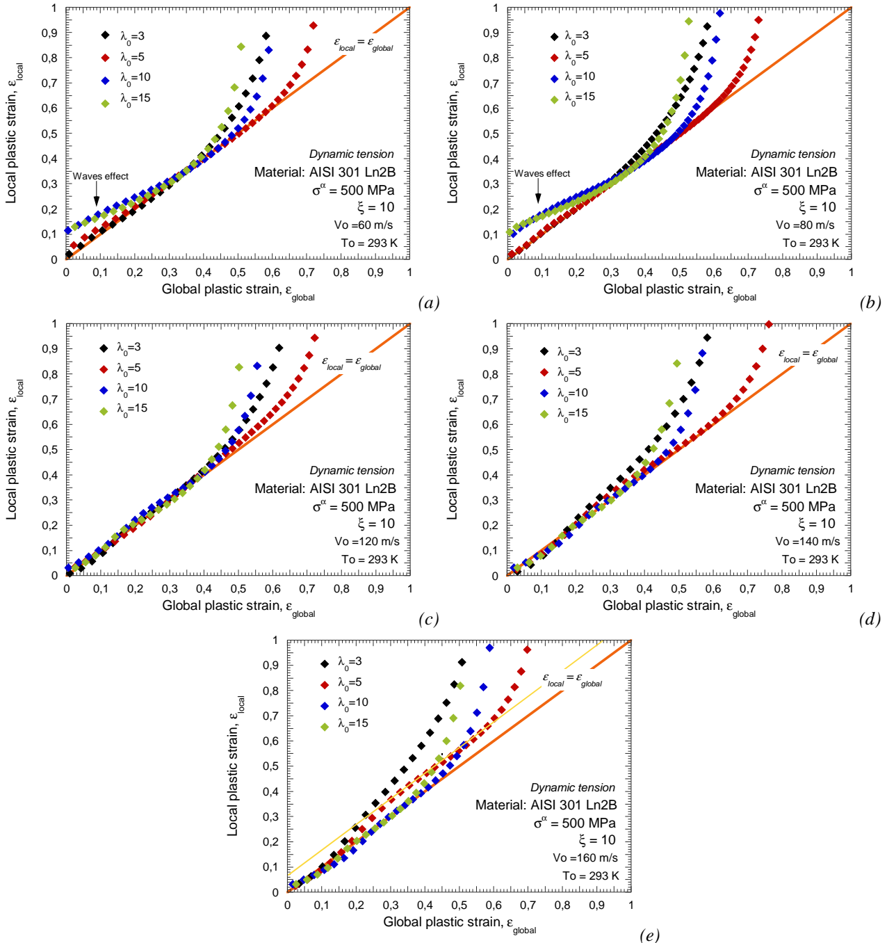
Fig. 3.94. Evolution of the local plastic strain as a function of the global plastic strain for the material configurations analyzed. (a) V_0=60 m/s, (b) V_0=80 m/s, (c) V_0=120 m/s, (d) V_0=140 m/s, (e) V_0=160 m/s.
