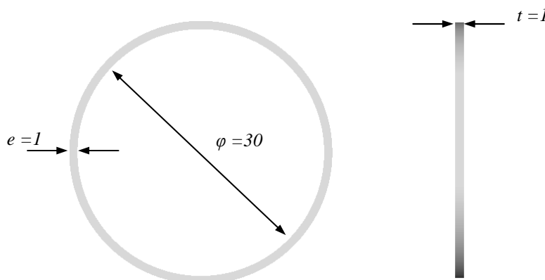
Fig. 3.6. Geometry and dimensions (mm) of the specimen used in the simulations [Rusinek and Zaera 2007].
