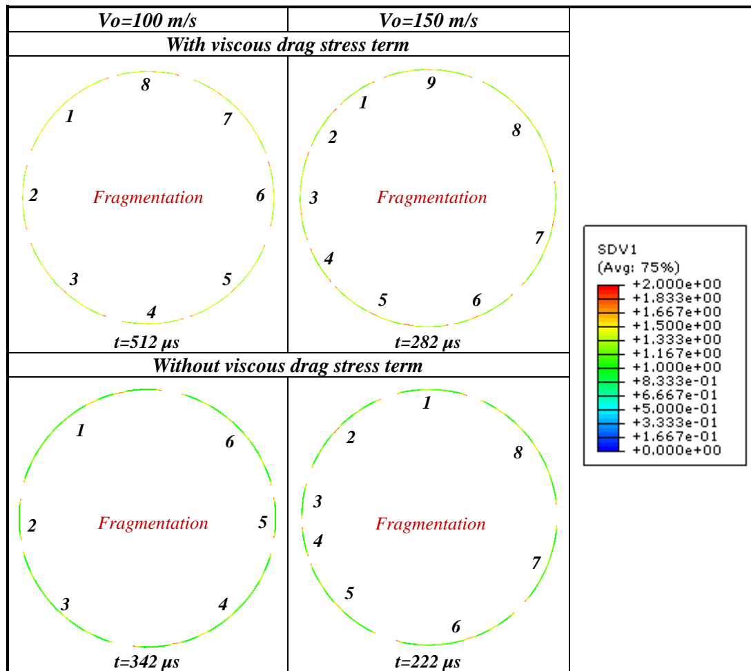
Fig. 3.22. Plastic strain contours at failure time and ring fragmentation for both models analyzed and two different impact velocities, V_0=100 m/s and V_0=150 m/s.
