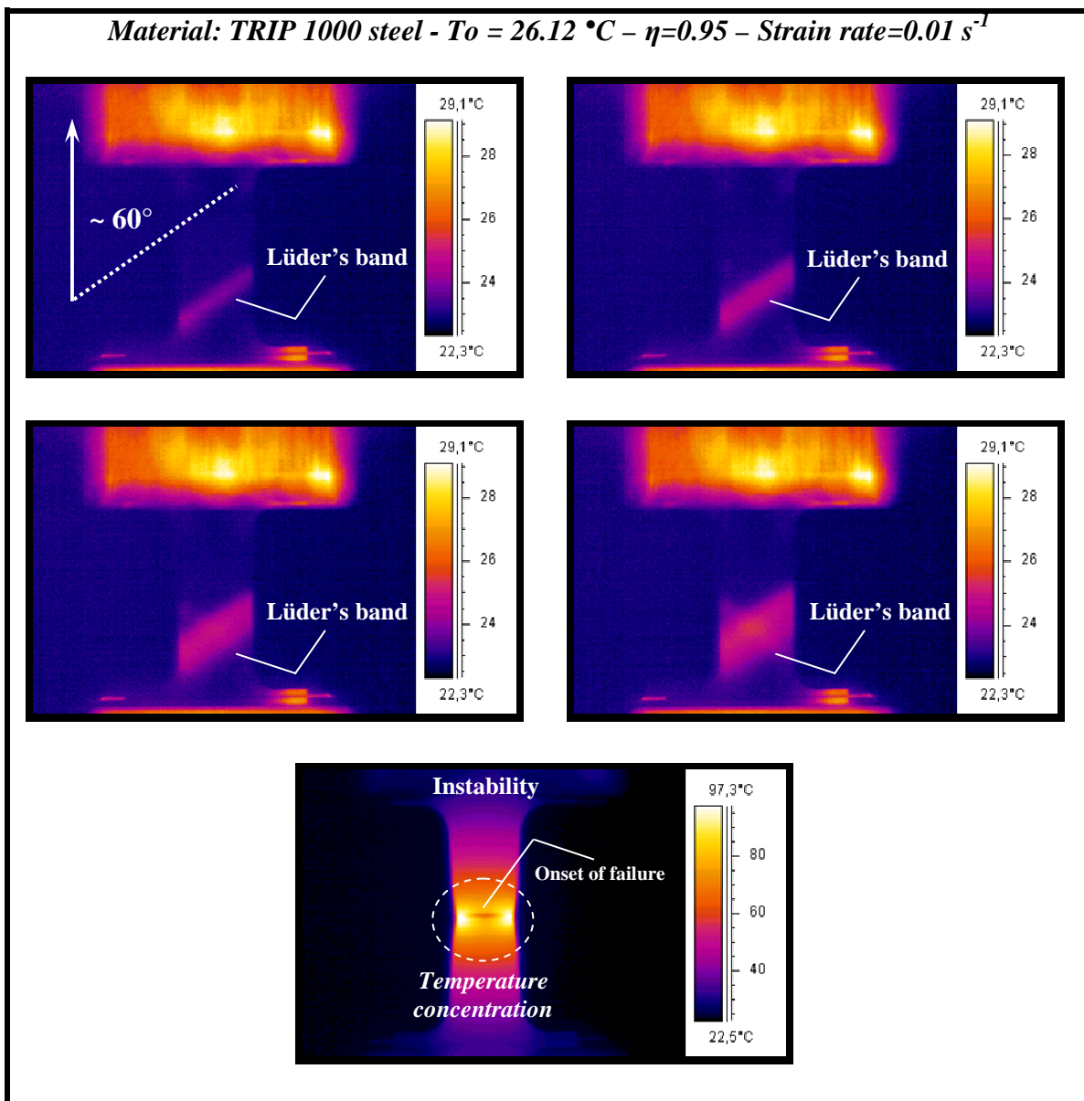
Fig. 5.47. Temperature contours during loading [Rusinek and Klepaczko 2009].
