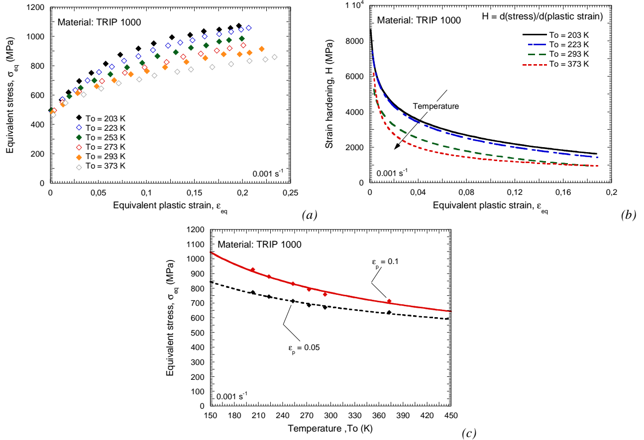
Fig. 5.46. (a) Flow stress of TRIP 1000 as a function of plastic strain for different initial temperatures. (b) Strain hardening of TRIP 1000 as a function of plastic strain for different initial temperatures. (c) Evolution of the flow stress as a function of temperature for different plastic strain values.
