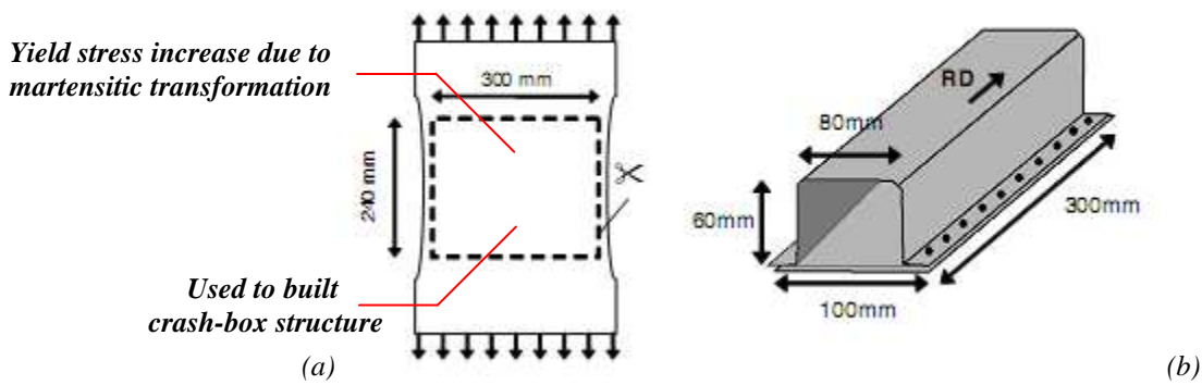
Fig. 2.42. Pre-strain history of a crash box structure (a) Specimen dimensions after pre-strain process. (b) Omega box after bending [Durrenberger et al. 2006].
