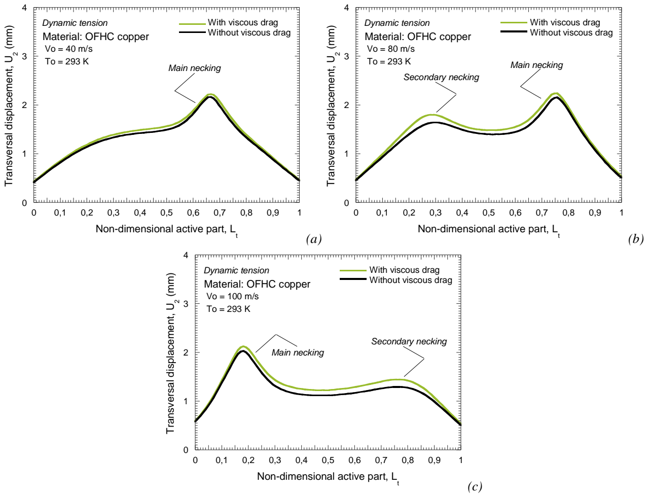
Fig. 3.28. Transversal displacement of the active part of the specimen for MRK and extended MRK models. (a) V_o=40 m/s, (b) V_o=80 m/s, (c) V_o=100 m/s.
