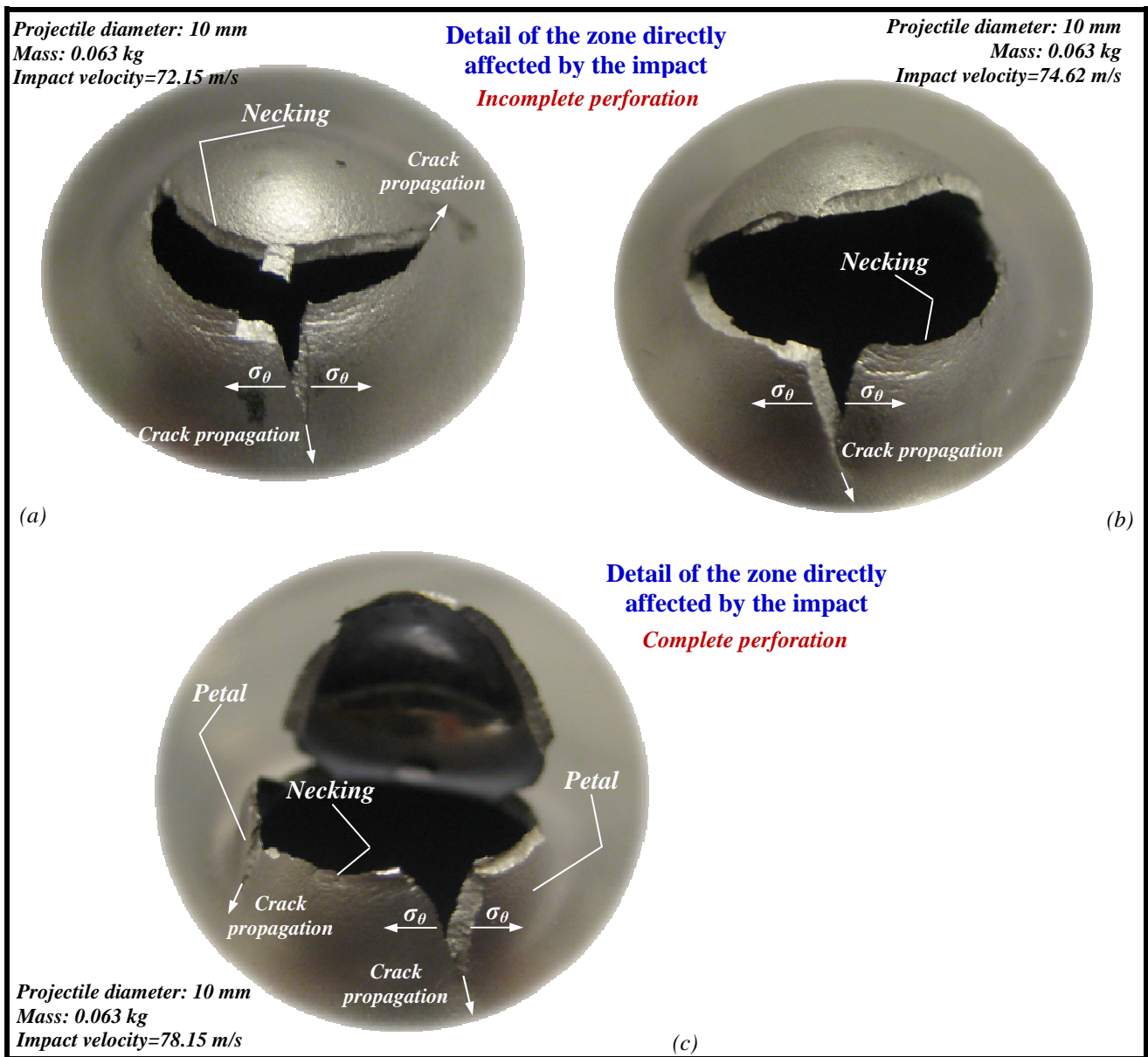
Fig. 5.35. Final stage of the impact process for different initial velocities. (a) V_0 = 72.15 \text{ m/s} , (b) V_0 = 74.62 \text{ m/s} , (c) V_0 = 78.15 \text{ m/s} .
