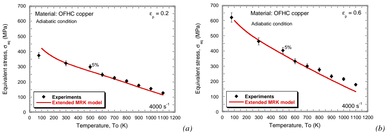
Fig. 2.33. Temperature sensitivity description using the extended MRK model and comparison with experiments at 4000 \text{ s}^{-1} . (a) \epsilon_p=0.2 , (b) \epsilon_p=0.6 [Nemat-Nasser and Li 1998].
