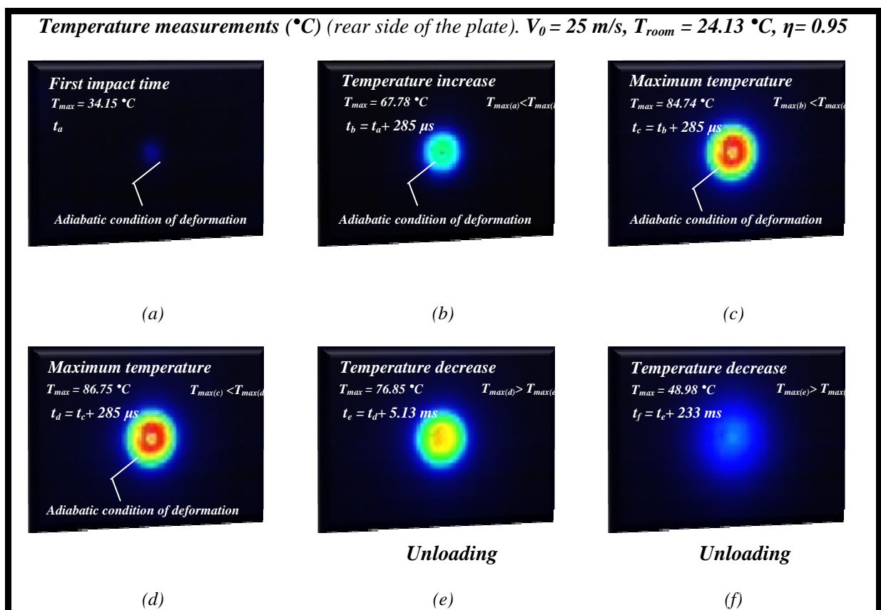
Fig. 4.20. Temperature in the rear side of the target for different stages of the impact process. V_0 = 25 m/s and T_{room} = 24.13 °C. (a) T_{max} = 34.15 °C ; (b) T_{max} = 67.78 °C ; (c) T_{max} = 84.74 °C ; (d) T_{max} = 86.75 °C ; (e) T_{max} = 76.85 °C ; (f) T_{max} = 48.98 °C. Picture resolution 80 \times 64 pixels.
