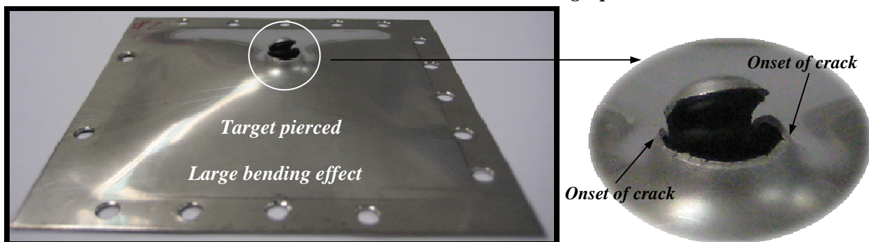
Fig. 5.25. Pierced target, steel AISI 304, V_0=3.0 m/s at room temperature.
