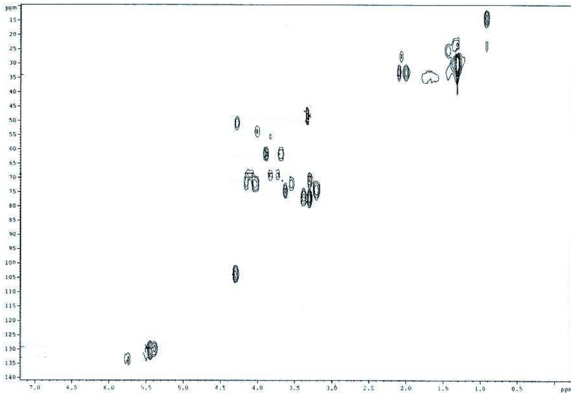
Figure 42: Spectre de corrélation ^1\text{H} - ^{13}\text{C} (HSQC) de LP11
