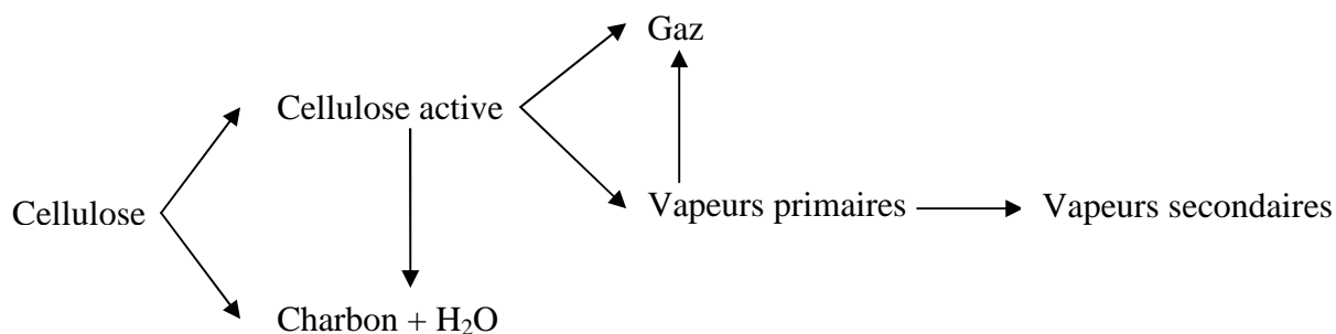
Figure I.5 Schéma de Diebold [7]
