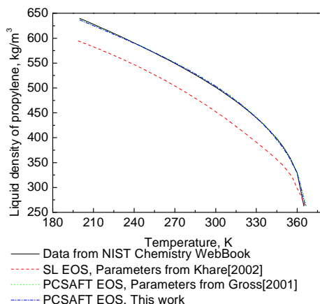
图3.3 液相丙烯密度计算值与文献值的比较 Fig. 3.3 Comparison of calculated data with literature for the density of liquid propylene
