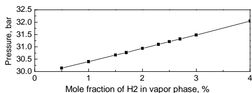
图7.16 液相反应器压力随气相氢浓度变化 Fig. 7.16 Effect of the setpoint of the y_{H_2} on the reactor pressure
