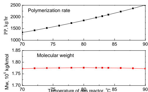
图7.23 聚合物量及其分子量随温度的变化 Fig. 7.23 Effect of the gas reactor temperature on the polymerization rate and weight-average molecular weight of PP
