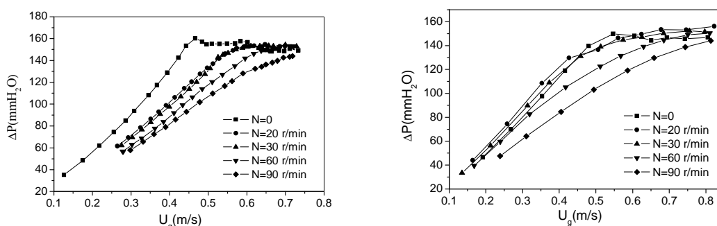
(a) d_p=1.69\text{mm} L_\theta=437\text{mm} , dual anchor impeller with an orifice gas distributor
