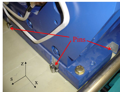
Figure 3.32: Positioning Pins
