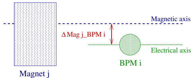
Figure 4.1: Alignment Offset
