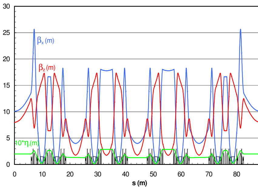
Figure 4.10: SOLEIL Storage Ring beta functions and dispersion function
