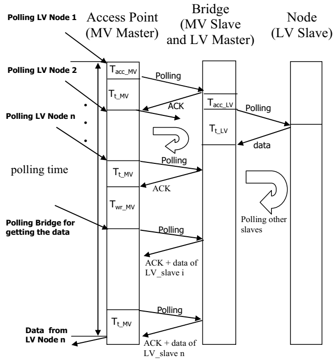
Figure 5.8: Schematic representation of average polling time at the Network Layer level in the case of with cash in the slave
