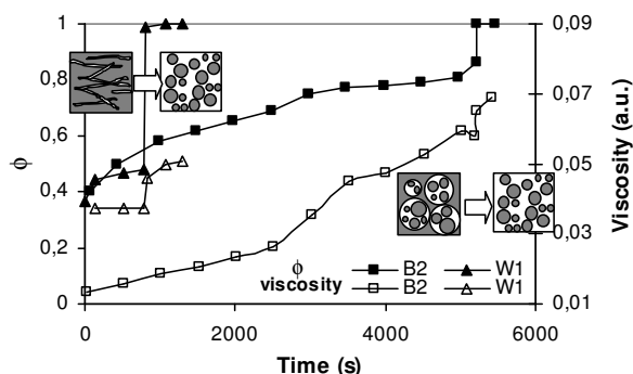
Figure 9. Viscosity follow-up and dispersed phase fraction under stirring for systems with different water viscosity. (B2) \eta_o = 0.001 Pa.s, \eta_w = 0.001 Pa.s; (W1) \eta_o = 0.02 Pa.s, \eta_w = 0.001 Pa.s. fw = 0.7
