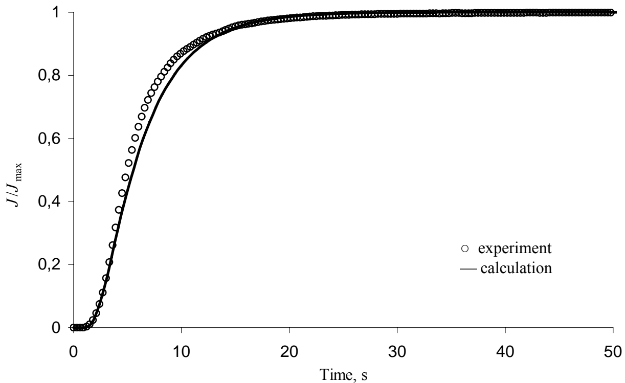
Fig. 4.1. Non-steady flux of \text{CO}_2 in SMV with stagnant liquid layer (distilled water, H_{liq} = 260 \mu\text{m} ).
