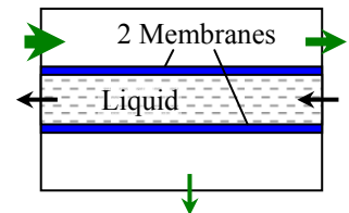
Fig. 1.: Schematic representation of SMV
