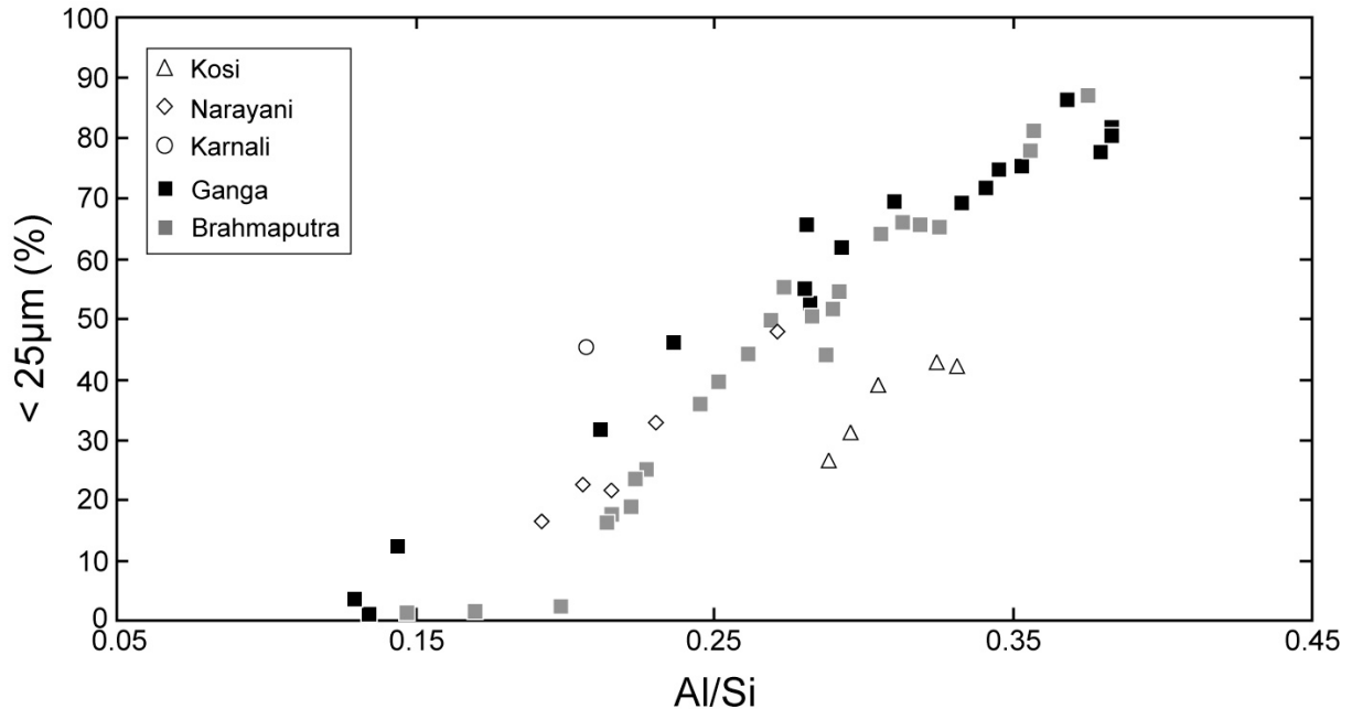
Figure 4.22: Co-variation of the proportion of fine (< 25 μm) particles with Al/Si ratio in G-B river sediments. Ganga and Brahmaputra sediments define comparable trends. This co-variation is generated by sediment segregation under hydrodynamic forces that concentrates fine grained phyllosilicates in surface suspended sediment and coarse quartz and feldspar in bed sediment.
