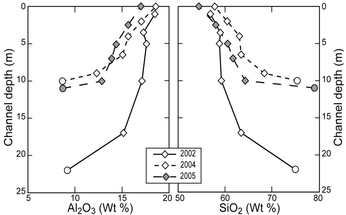
Figure 3.17: \text{SiO}_2 and \text{Al}_2\text{O}_3 concentrations in suspended (diamonds) and bed sediments (circles) as a function of sampling depth in the Ganga at Harding Bridge, Bangladesh. Variations are due to mineral sorting under hydrodynamic forces. Differences in channel depth are due to variations in the river bed geometry and do not reflect flood level changes.
