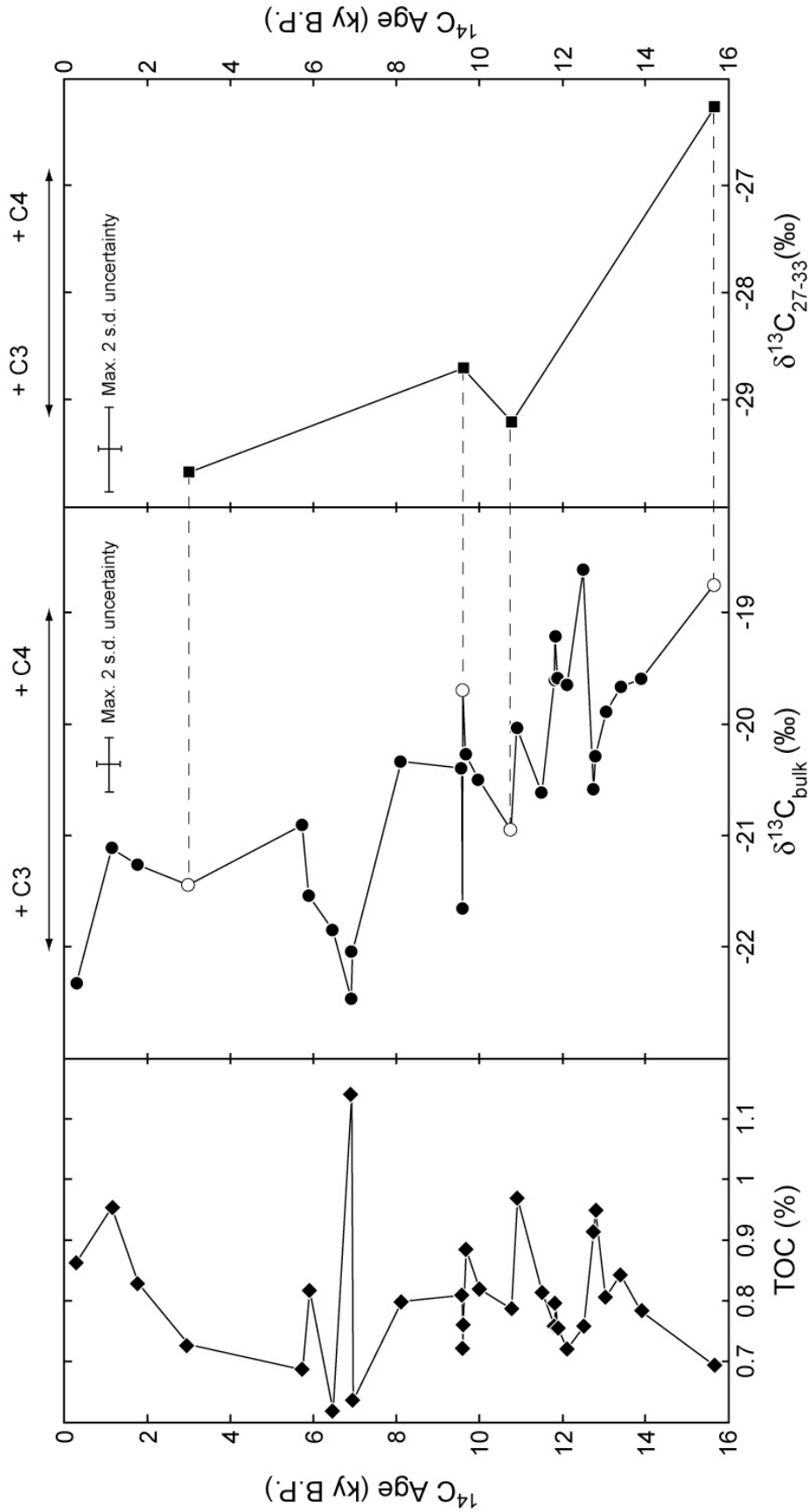
Figure 4.35: Evolution of C_{org} content and isotopic composition during the last 16 ka of sedimentation in the middle Bengal Fan. \delta^{13}C_{27-33} represents the weighted average of C27, C29, C31 and C33 n-alkanes \delta^{13}C . From 16 to 7 ka, \delta^{13}C shifts towards 3 to 4 ‰ more negative values.
