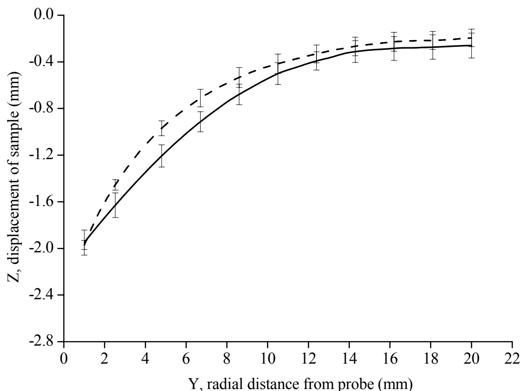
Figure 40. Surface displacement profile of 30-day-old Camembert cheese (—), Camembert cheese simulant (---). Error bars indicate standard deviation calculated from 6 and 3 repetitions for cheese and simulant respectively. Closest radial distance from probe was equal to 1 mm.
