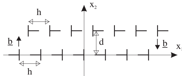
Figure X.9: Edge dipolar wall.
