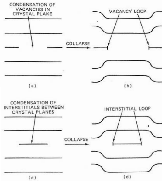
Figure II.15: Formation of vacancy and interstitial loops.
