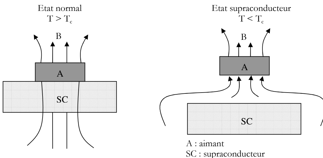
Figure I.2. Effet Meissner.
