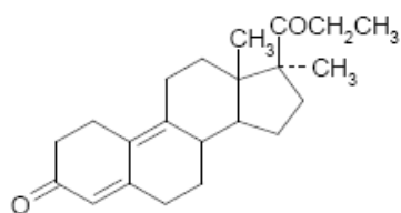
Promegestone
