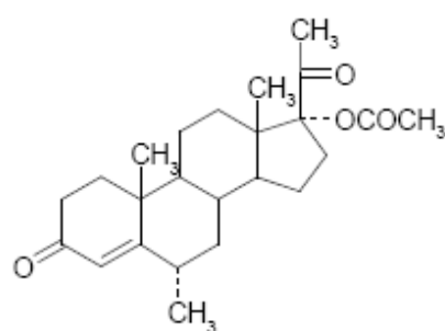
Medroxyprogesterone acetate
