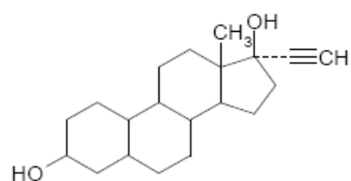
Tetrahydronorethisterone
