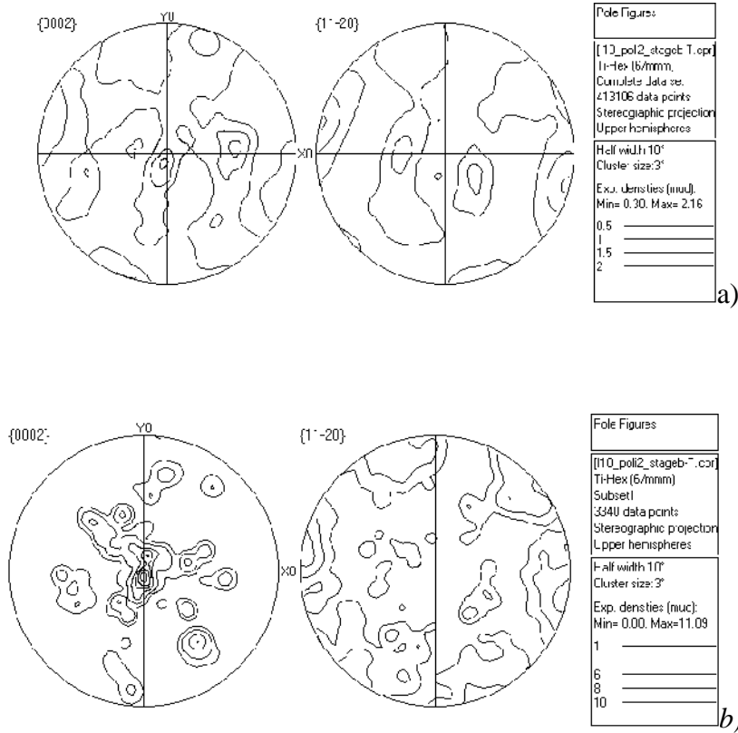
Figure CI10.16 Figure de pôles \{0002\}/\{11-20\}
