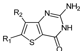
Figure 6 : Aminothiéno [3,2-d] pyrimidinone
