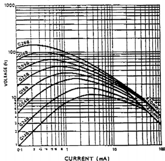
Voltage v. Current in Free Air at T_{amb} = 23^{\circ}C
