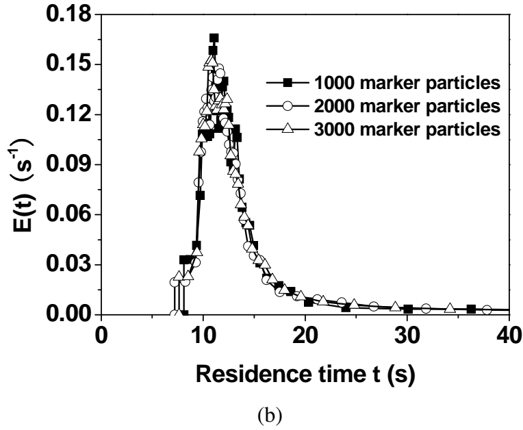
Fig. 4.5 Simulated residence time distributions with different marker particles. (a) KD2, screw speed = 120 rpm, feed rate = 10.7 kg/h; (b) KD3, screw speed = 150 rpm, feed rate = 17.8 kg/h.
