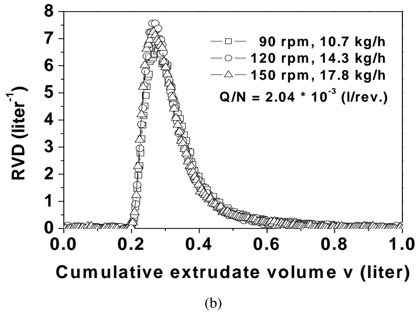
Fig. 3.9 RVD corresponding to probes 1 and 2, respectively. (a) Probe 1; (b) probe 2; screw configuration 1; Q/N = 2.04 \times 10^{-3} liter/revolution. Note that all the RVD curves overlap.
