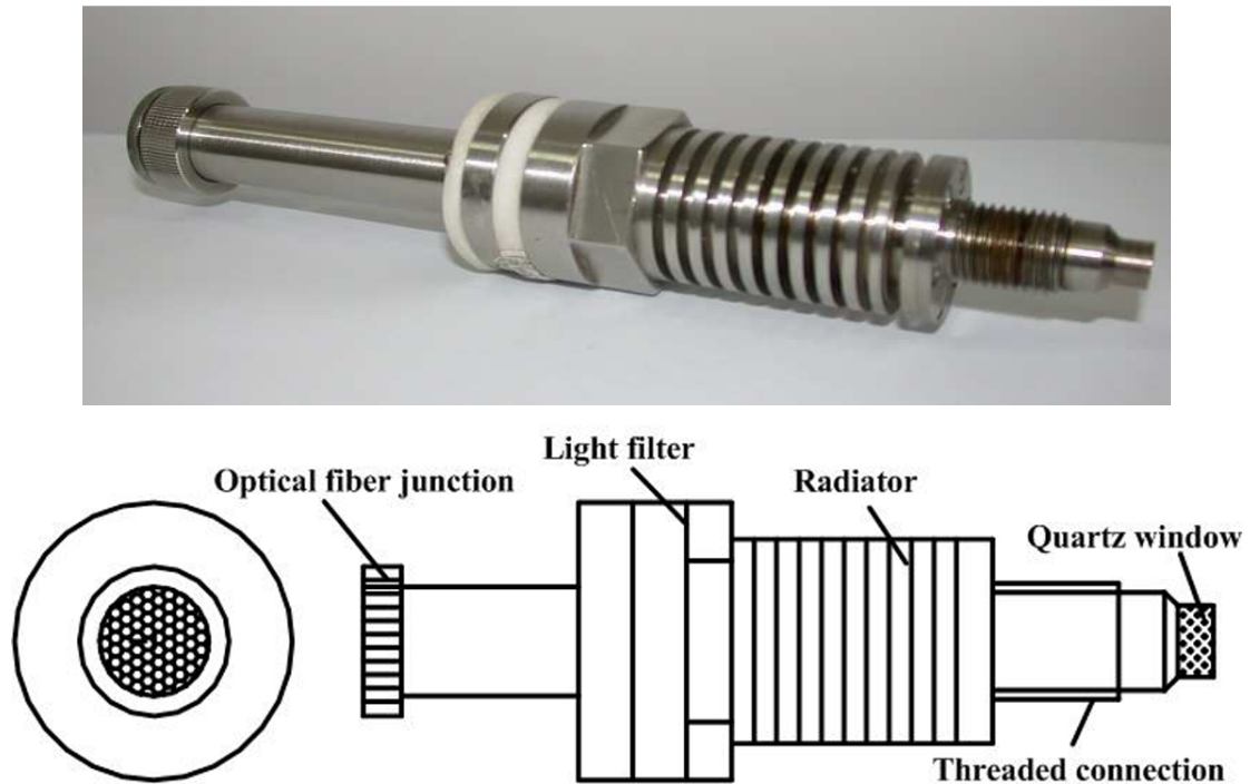
Fig. 2.4. A picture and a schematic diagram of optical probe.
