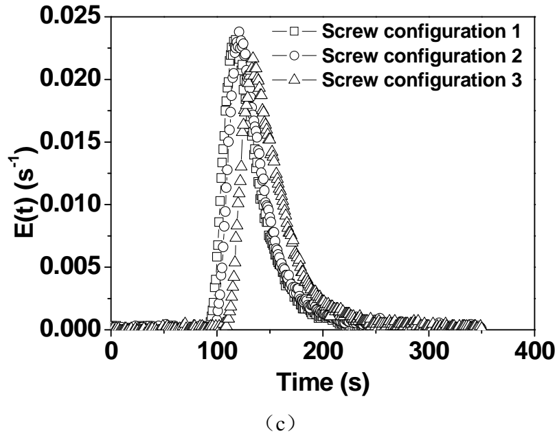
Fig. 2.10 Effect of the staggering angle of the kneading discs on the partial RTDs. (a) probe 1 (b) probe 2 (c) probe 3. Screw speed = 120 rpm; feed rate = 15.5 kg/h.
