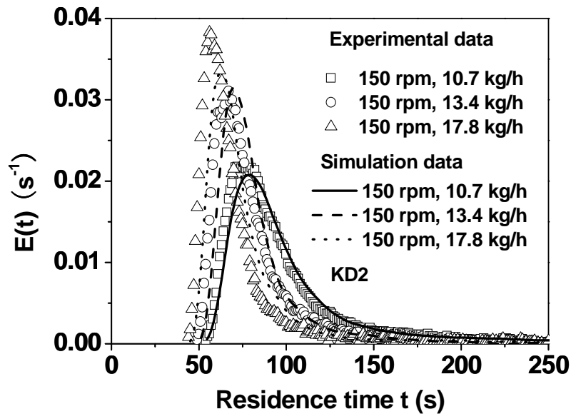
Fig. 4.9 Comparison of the local RTD between the numerical and experimental results for different feed rates.
