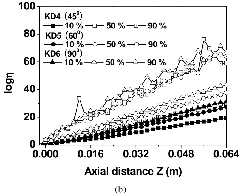
Fig. 4.13 Axial evolution of \log\eta : (a) arithmetic mean of \log\eta , (b) critical value of \log\eta for given percentiles of marker particles. Screw speed: 150 rpm, feed rate: 17.8 kg/h.
