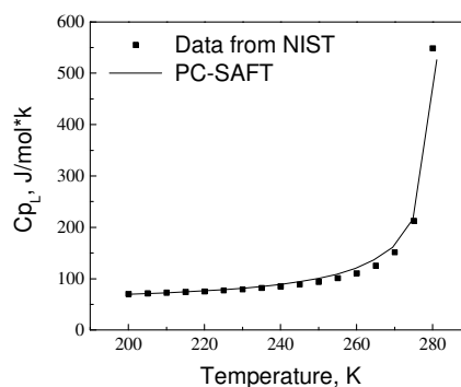
图3.2 乙烯饱和液相热容计算值和文献比较 Fig3.2 Comparison of ethylene liquid heat capacity between the literature and prediction
