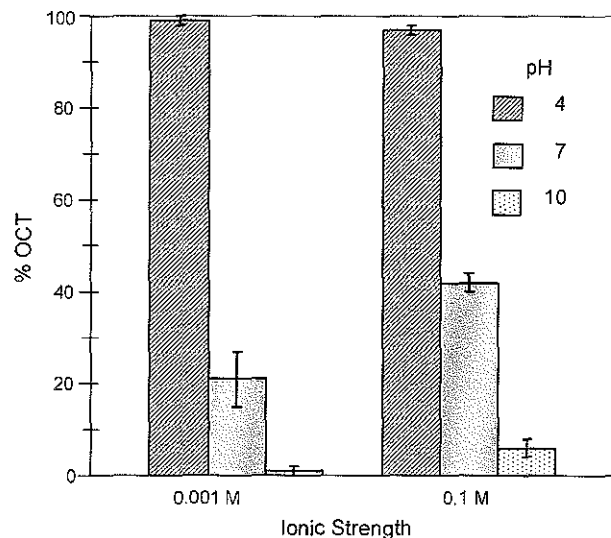
Fig. 1. Effect of pH and \text{KNO}_3 ionic strength on the percentage of cells trapped by the octane droplets.
