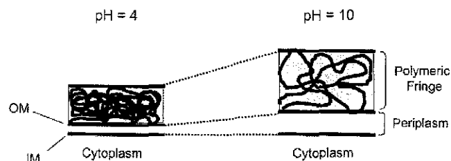
FIG. 3. Schematic view of the dynamic of the cell envelope in response to a change in pH from 4 to 10 (not drawn to scale). OM, outer membrane; IM, inner membrane.
