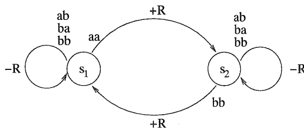
FIG. 6.5 – Shown is the multi-agent extension of the problem before. The optimal joint policy consists in selecting joint action aa and joint action bb with probability 0.5 each, while avoiding joint actions ab and ba . This synchronization can only be achieved via an external correlation device. The example is taken from [BHZ05].
