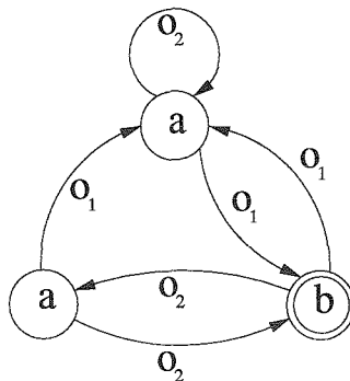
FIG. 3.11 – A deterministic finite state controller with 3 nodes for a problem with 2 actions ( a and b ) and 2 observations ( o_1 and o_2 ).
