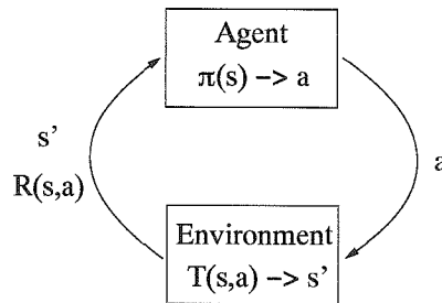
FIG. 3.3 – The basic cycle of reinforcement learning : an agent choses an action based on its internal policy \pi , the environment transitions to a new state, and provides the agent with an associated reinforcement signal R(s, a) .
