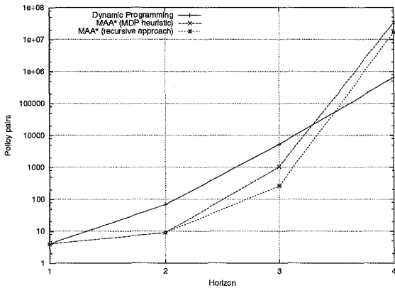
FIG. 9.7 – The number of evaluated policy pairs for dynamic programming, MAA* with the MDP heuristic, and recursive MAA* on the channel problem (logarithmic scale).
