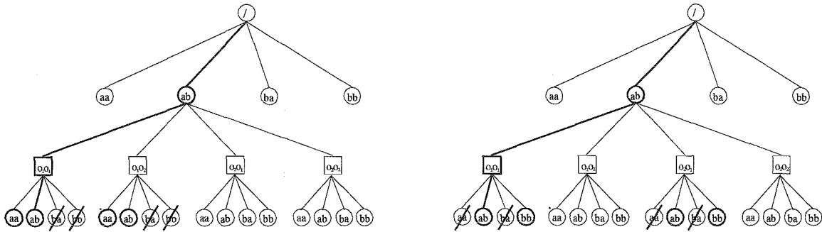
FIG. 7.2 – The two different subjective views of agent 1 and agent 2 respectively, when considering the evaluation of joint action \langle a, b \rangle that followed joint action \langle a, b \rangle and joint observation \langle o_1, o_1 \rangle in the tree of Figure 7.1 : each agent makes different assumptions about the correlation of this node with the joint actions of other nodes of the search tree.
