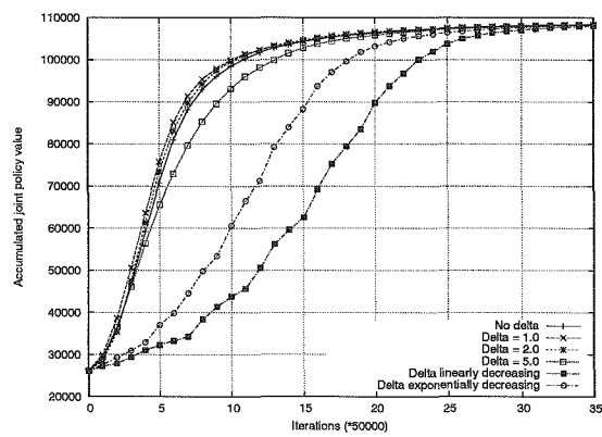
FIG. 9.21 – Soccer task : the joint policy value summed over both robots and all states for all 6 thresholds.
