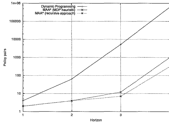
FIG. 9.8 – The actual memory requirements for dynamic programming, MAA* with the MDP heuristic, and recursive MAA* on the channel problem (logarithmic scale).
