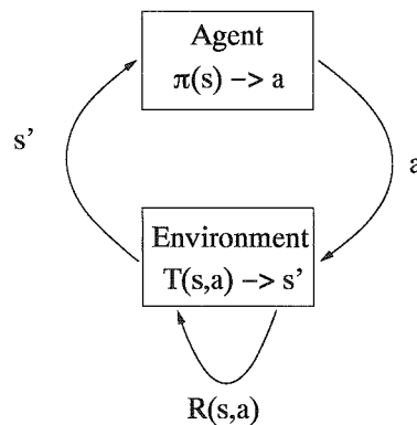
FIG. 3.1 – The basic cycle of policy execution : an agent chooses an action based on its internal policy \pi , the environment transitions to a new state, and a reward signal R(s, a) is produced and stored.
