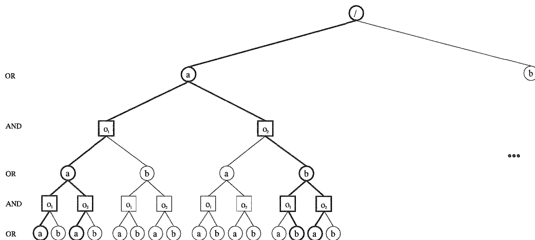
FIG. 3.10 – An extract of an AND/OR search tree for solving POMDPs. The nodes a and b are OR nodes and correspond to actions, whereas the nodes o_1 and o_2 are AND nodes and correspond to observations. A solution path is indicated in bold, and it represents the same policy as the one shown in Figure 3.5
