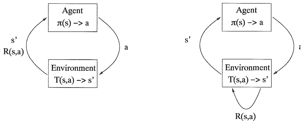
FIG. 8.4 – The fundamental difference between reinforcement learning (left) and planning (right). While agents are aware of their immediate reward in the first case, they have no knowledge about it during executing in the second case.
