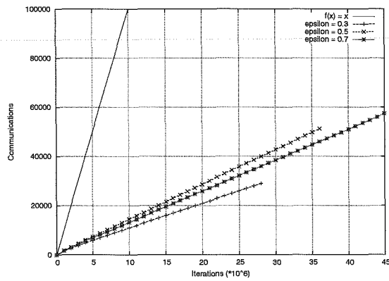
FIG. 9.18 – Coordination task : the total number of communications for three different exploration parameters ( \epsilon = 0.3 , \epsilon = 0.5 , and \epsilon = 0.7 ), again compared to the identity function f(x) = x .
