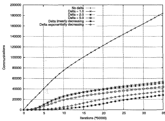
FIG. 9.20 – . Soccer task : the total number of communications for three fixed thresholds, two variable thresholds, and the no-threshold case.
