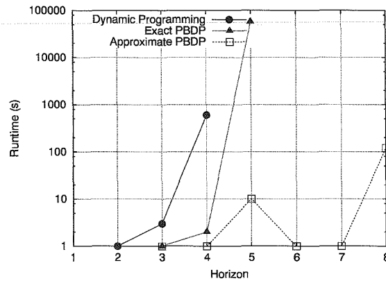
FIG. 9.11 – The effective runtime of the three approaches on the multi-access channel problem, measured in seconds and plotted on a logarithmic scale. The runtime of the approximate point-based dynamic programming approach is averaged over 10 trials.
