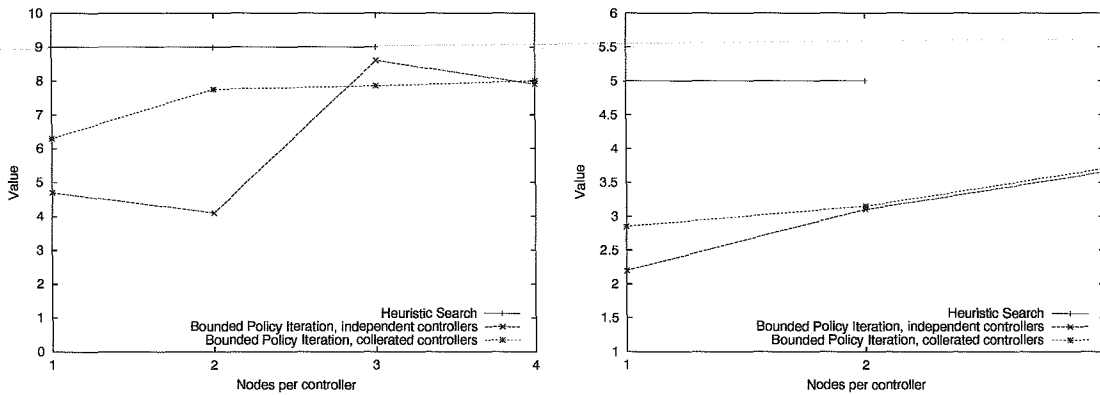
FIG. 9.13 – Value of optimal deterministic joint policy for the heuristic approach, and average value per trial run for two versions of bounded policy iteration on stochastic controllers. Left : Channel problem - Right : Meeting on a grid problem.
